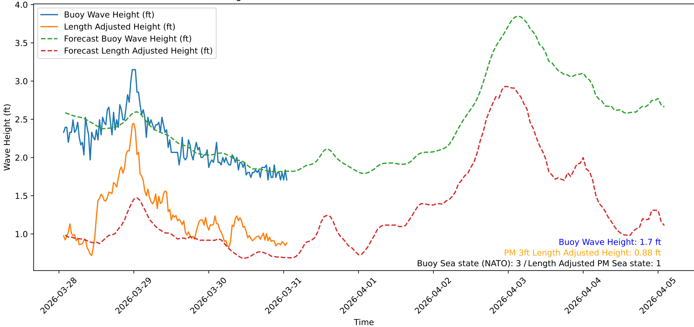
Wave Heights over Time for Oceanside Harbor at 2026-03-31 01:30:31
