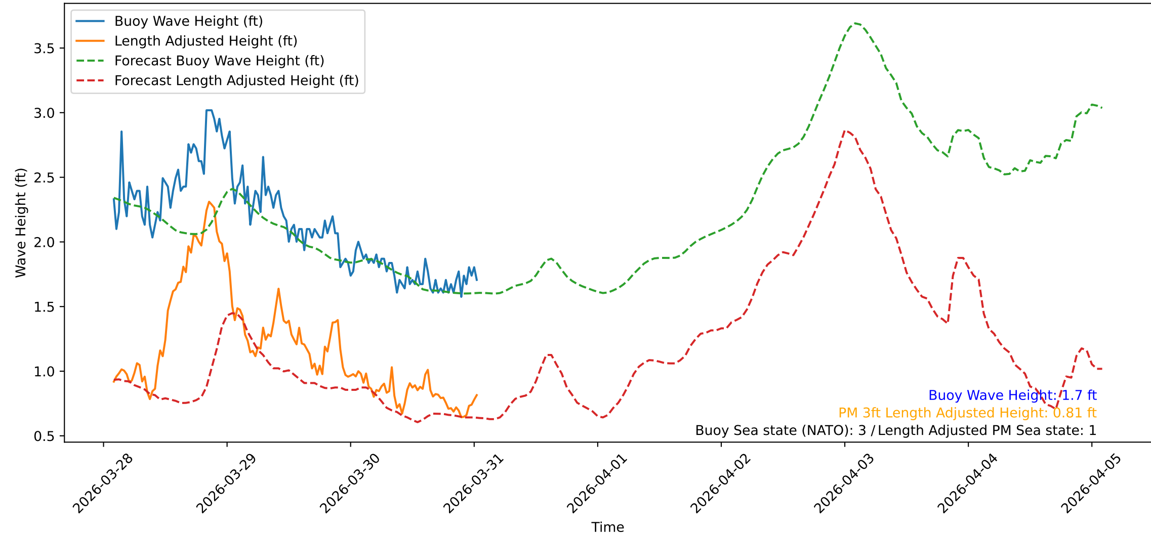
Wave Heights over Time for Red Beach at 2026-03-31 01:30:47
