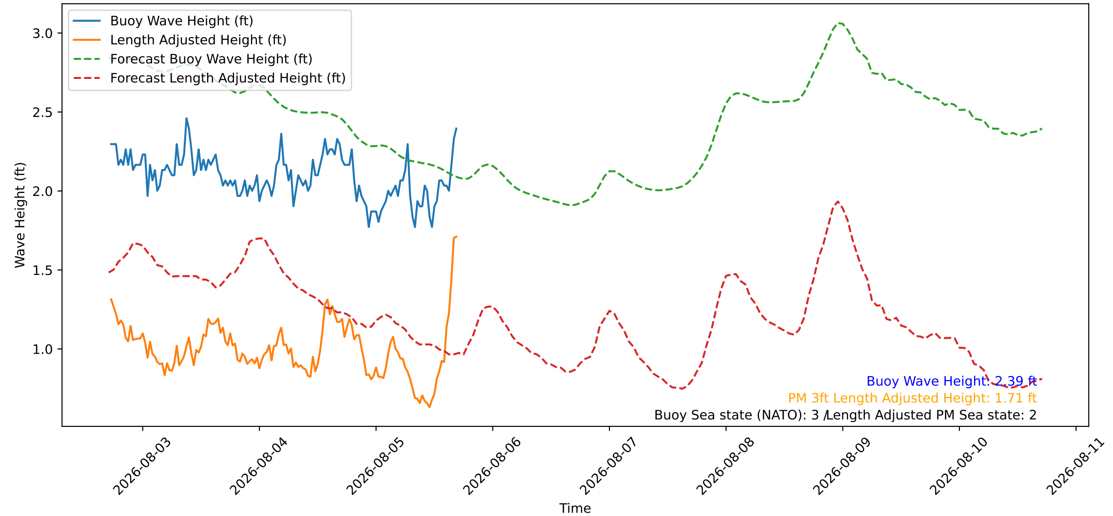
Wave Heights over Time for Red Beach at 2026-08-05 17:20:47
