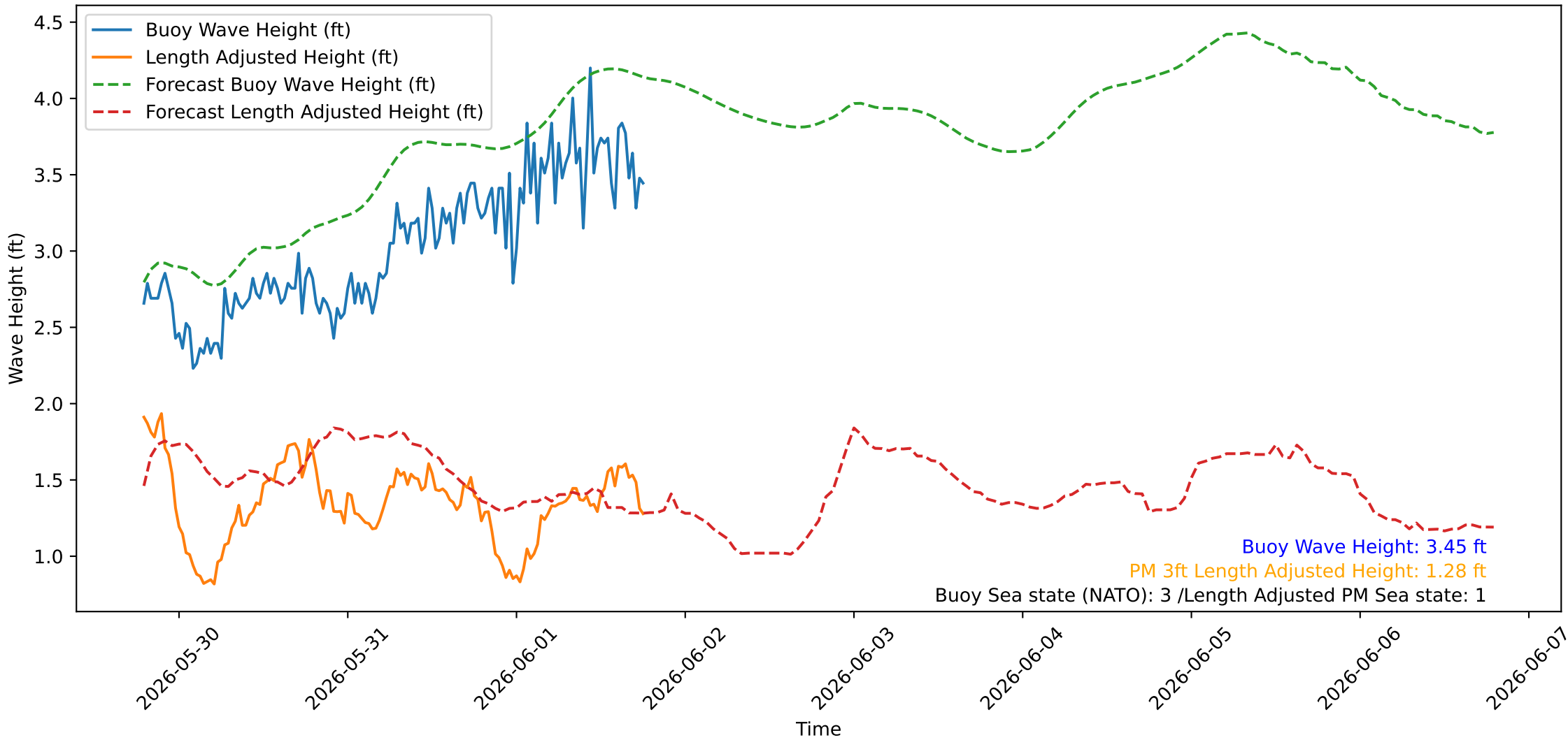
Wave Heights over Time for Red Beach at 2026-06-01 18:50:46
