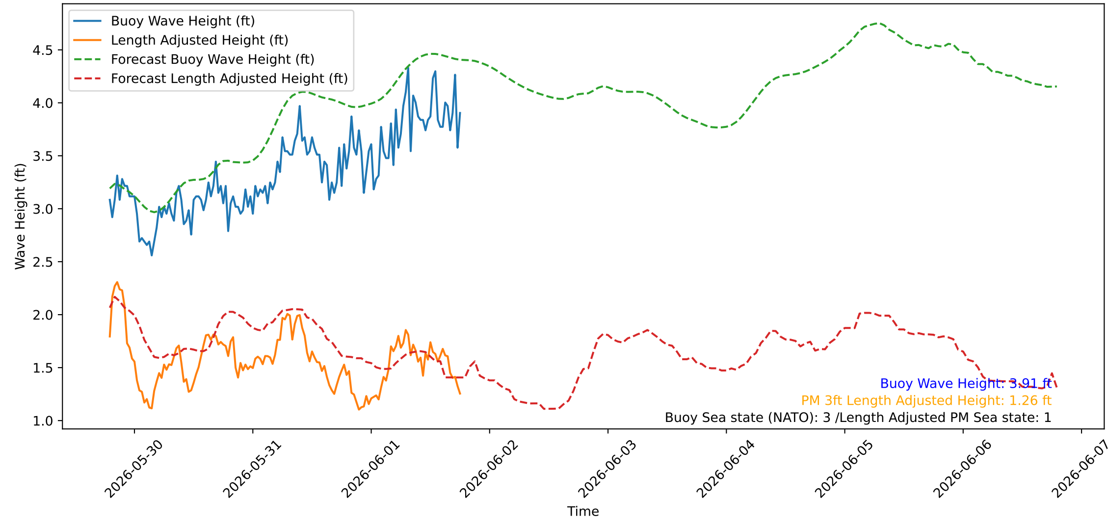
Wave Heights over Time for Green Beach at 2026-06-01 18:51:09
