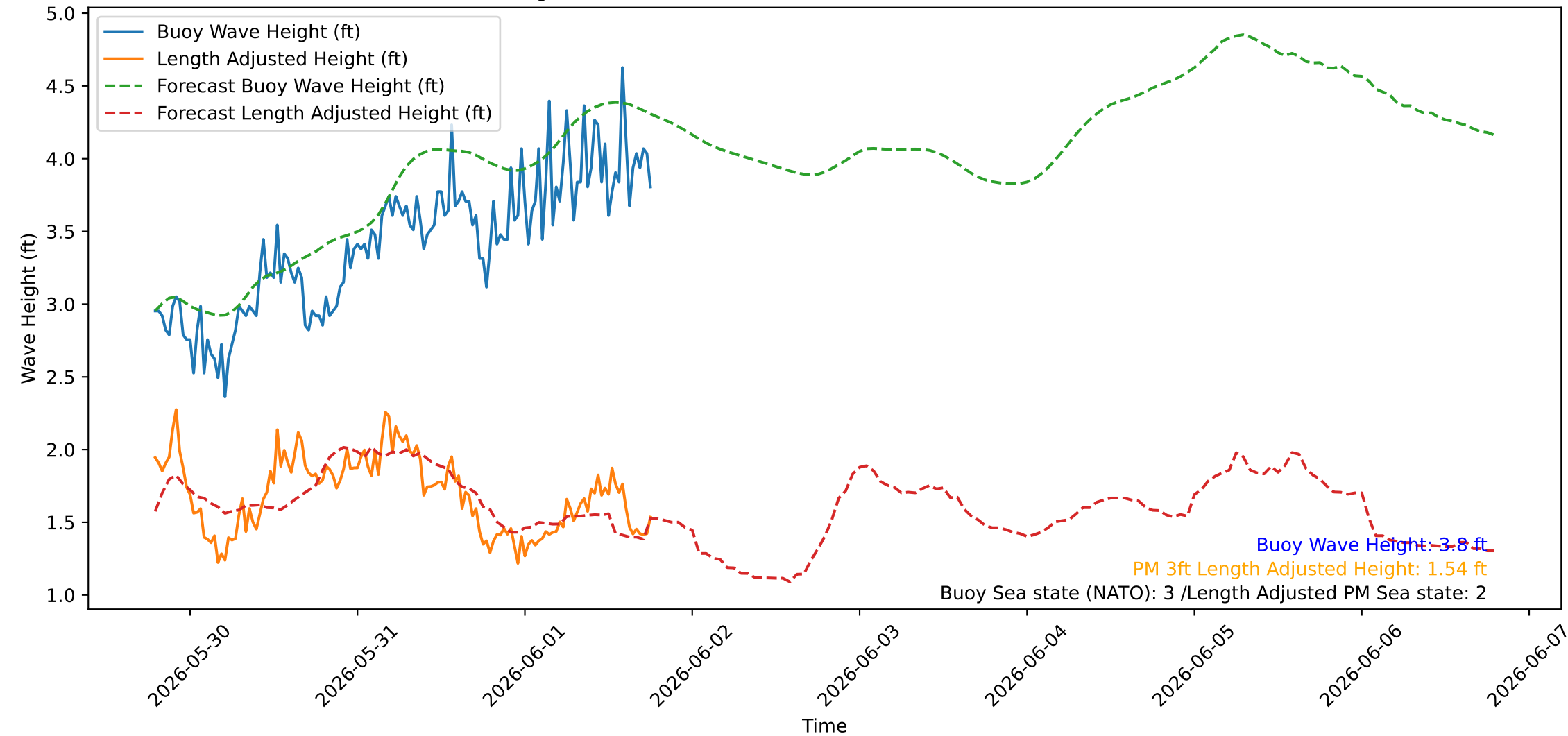
Wave Heights over Time for Oceanside Harbor at 2026-06-01 18:50:25
