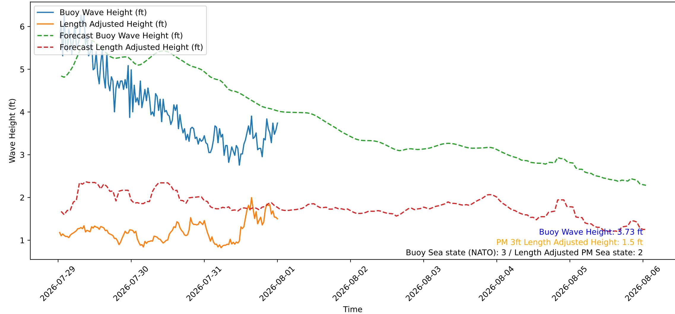
Wave Heights over Time for Green Beach at 2026-08-01 00:41:09
