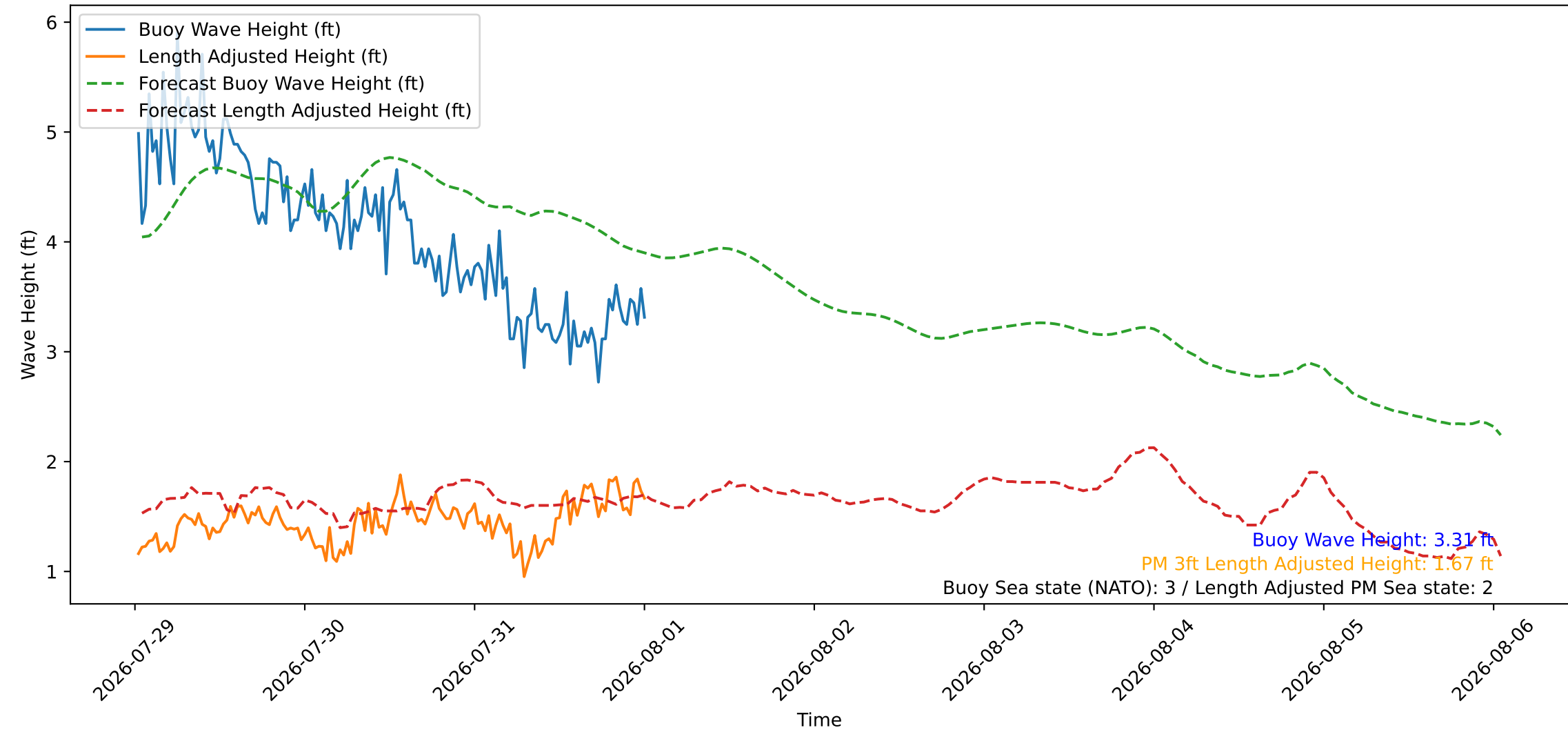
Wave Heights over Time for Oceanside Harbor at 2026-08-01 00:40:26
