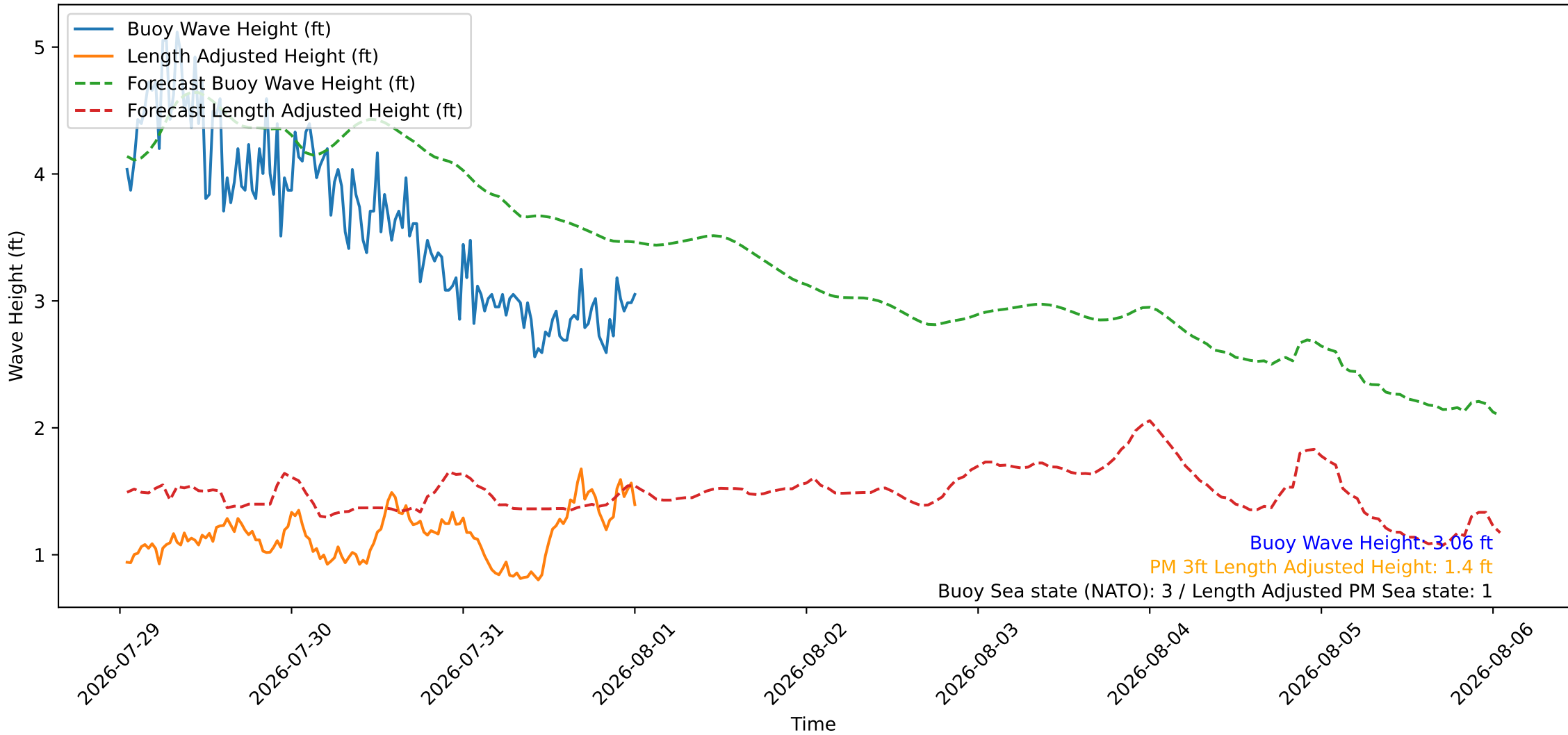
Wave Heights over Time for Red Beach at 2026-08-01 00:40:46
