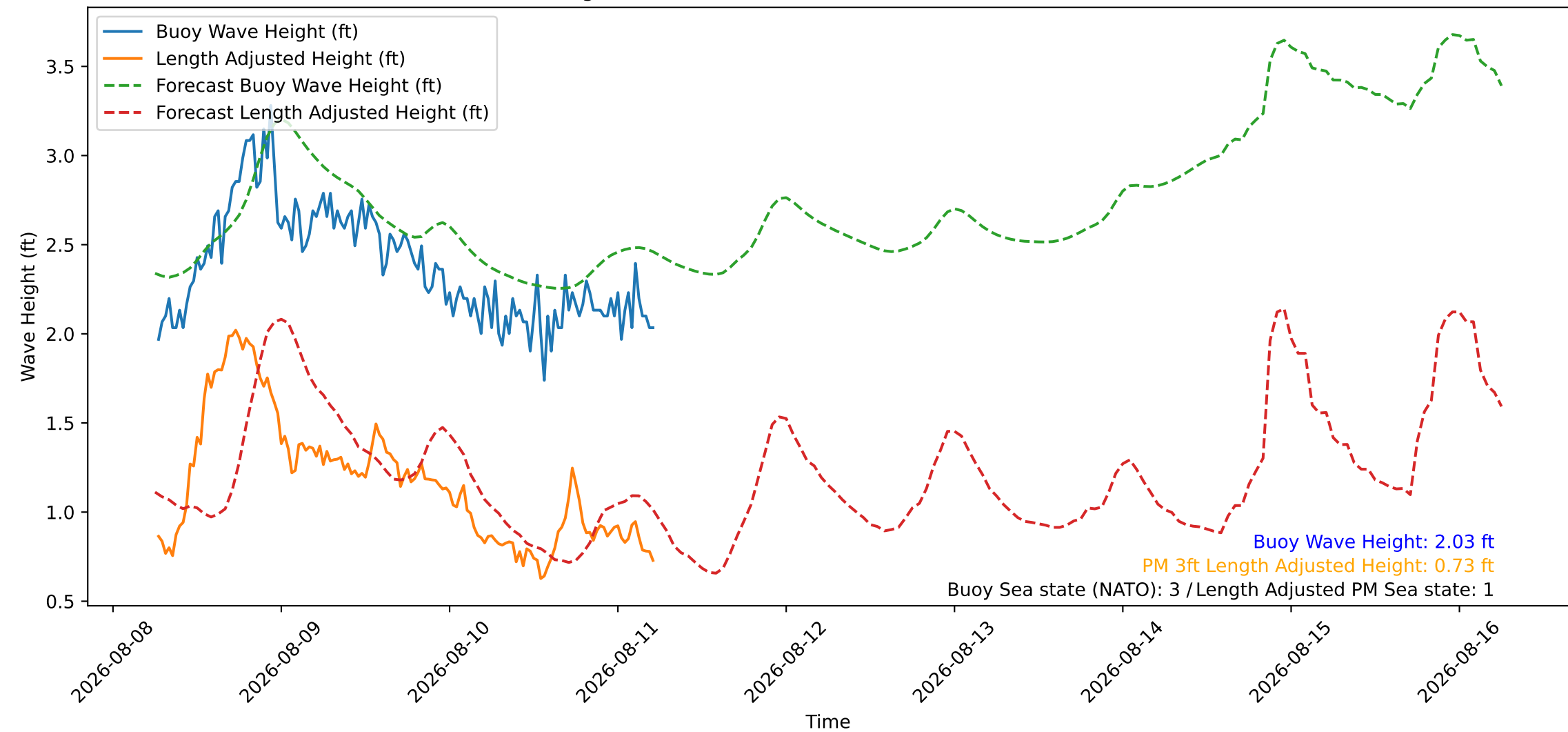
Wave Heights over Time for Red Beach at 2026-08-11 06:00:46
