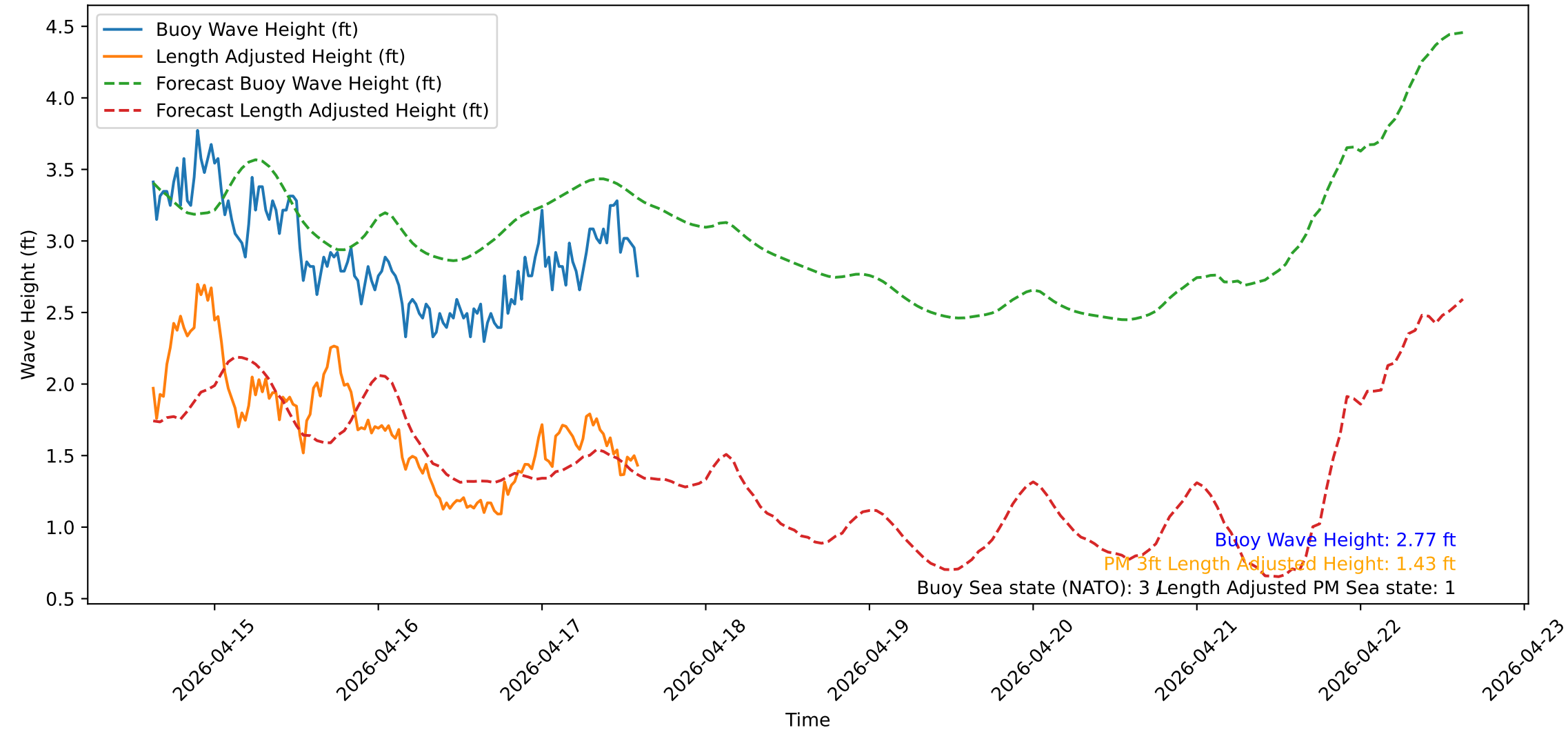
Wave Heights over Time for Oceanside Harbor at 2026-04-17 14:50:31
