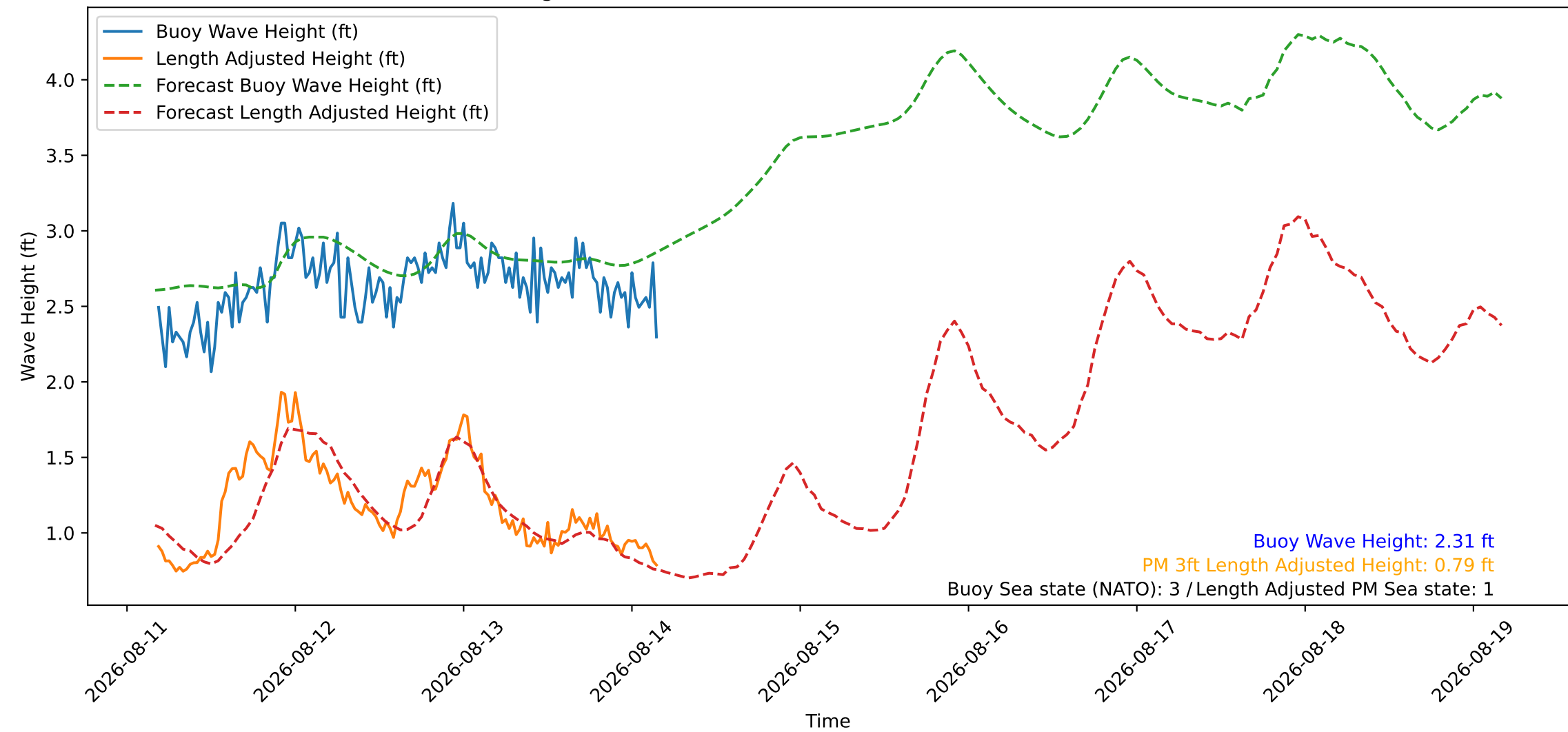
Wave Heights over Time for Oceanside Harbor at 2026-08-14 04:20:26
