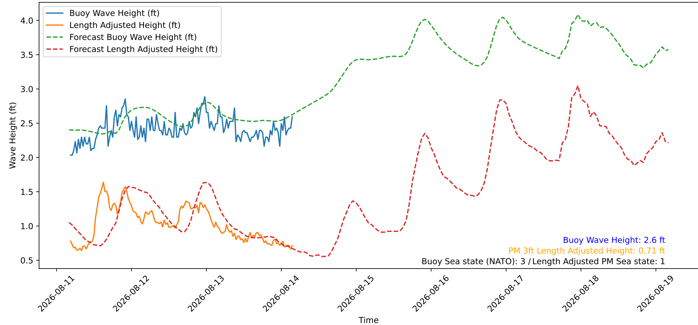
Wave Heights over Time for Red Beach at 2026-08-14 04:20:47
