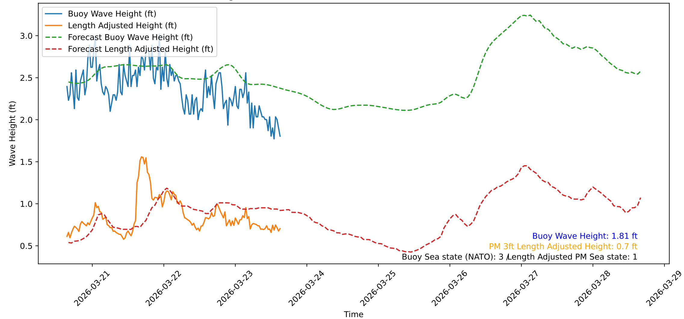
Wave Heights over Time for Oceanside Harbor at 2026-03-23 15:40:31
