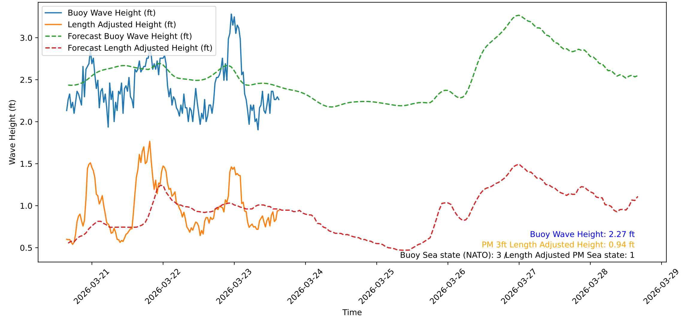
Wave Heights over Time for Green Beach at 2026-03-23 15:41:09
