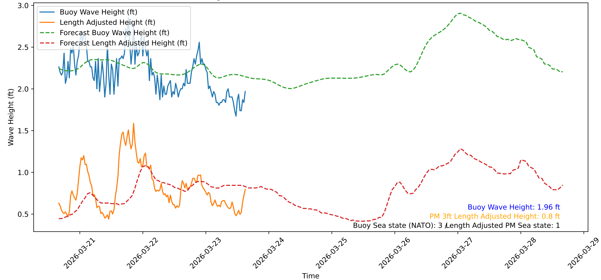
Wave Heights over Time for Red Beach at 2026-03-23 15:40:47
