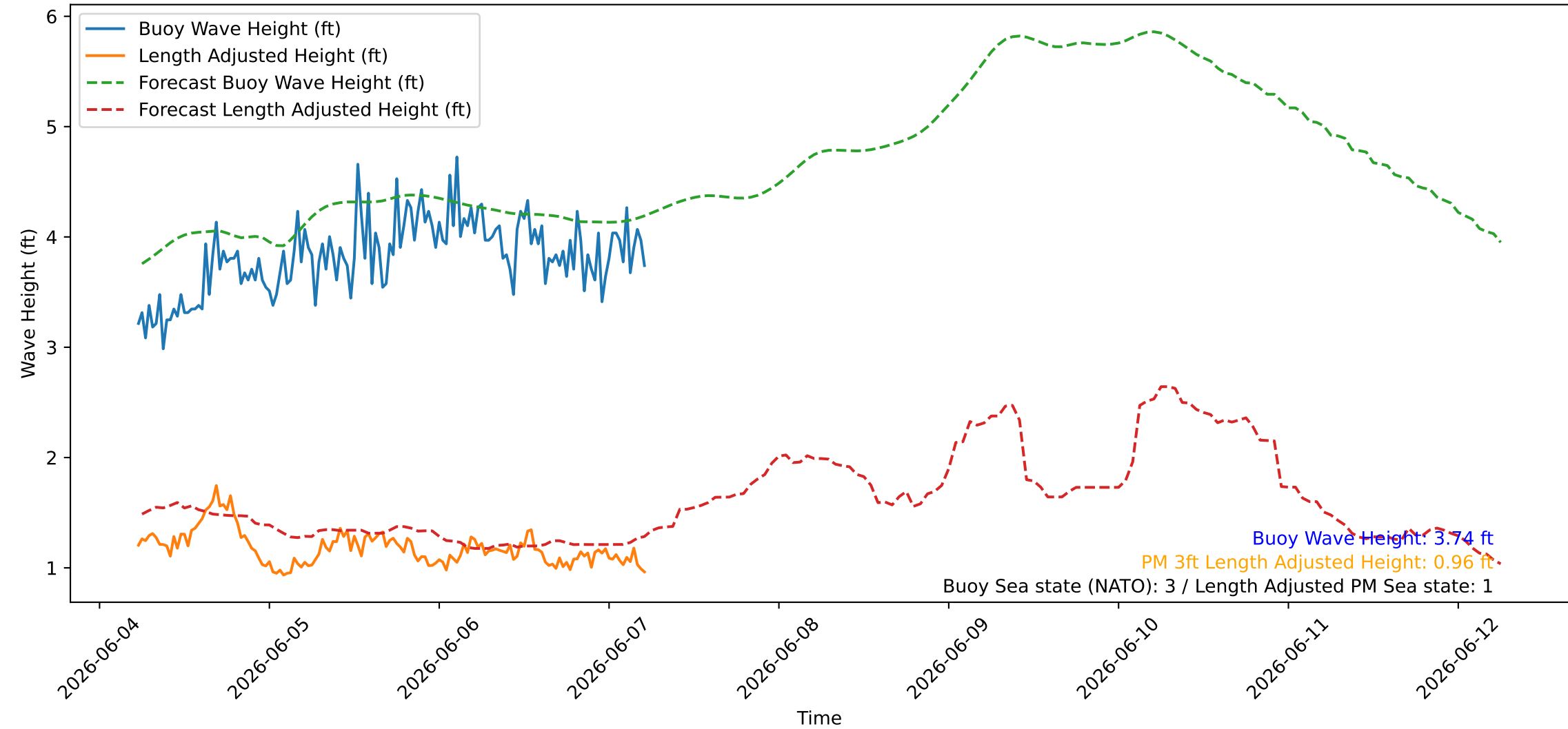
Wave Heights over Time for Green Beach at 2026-06-07 05:41:09
