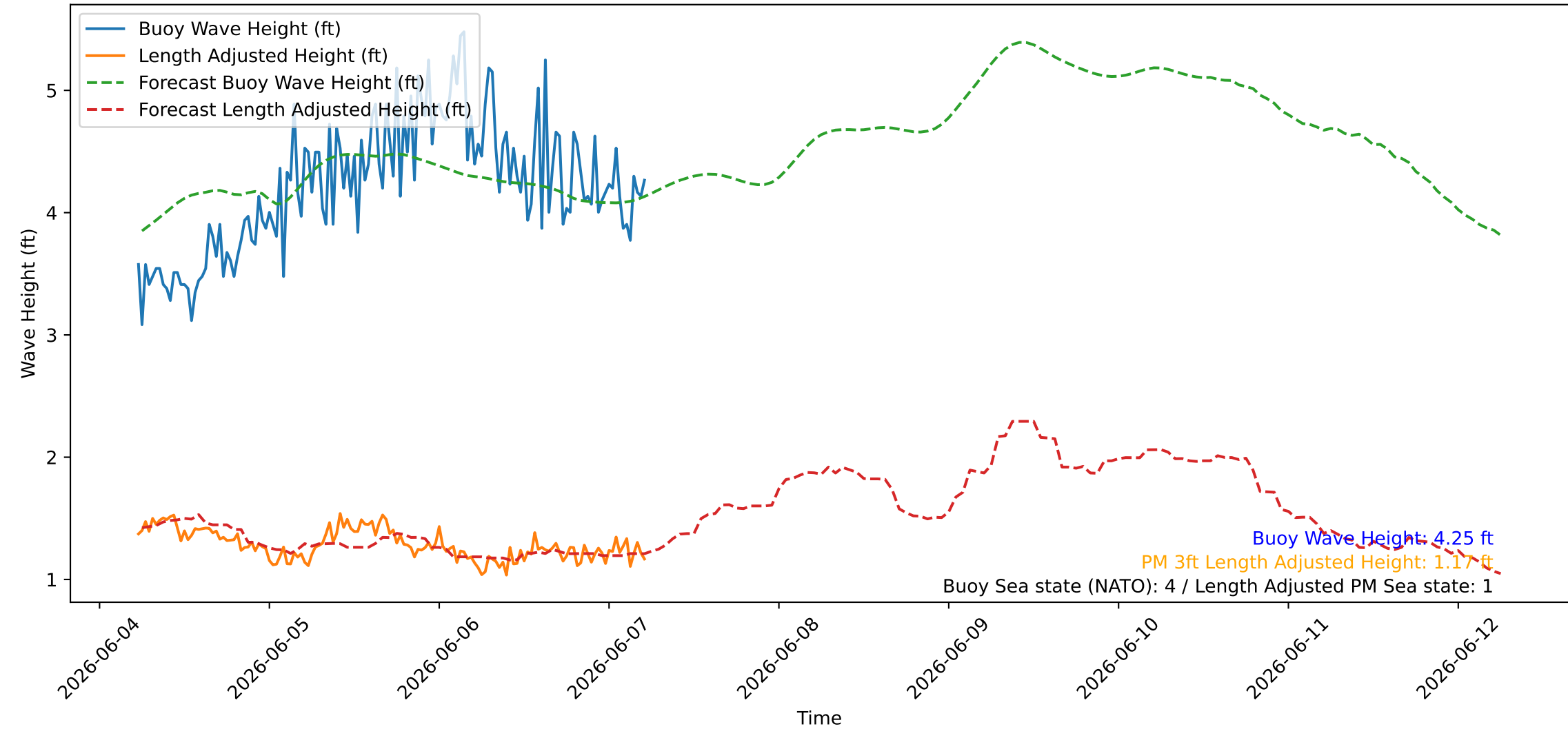
Wave Heights over Time for Oceanside Harbor at 2026-06-07 05:40:26
