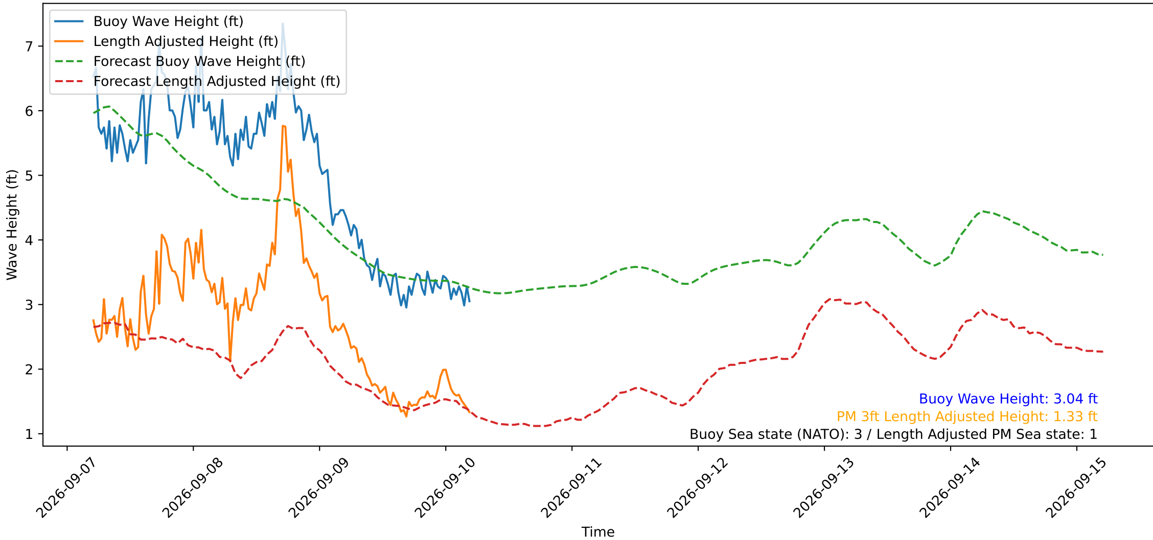
Wave Heights over Time for Oceanside Harbor at 2026-09-10 05:10:29
