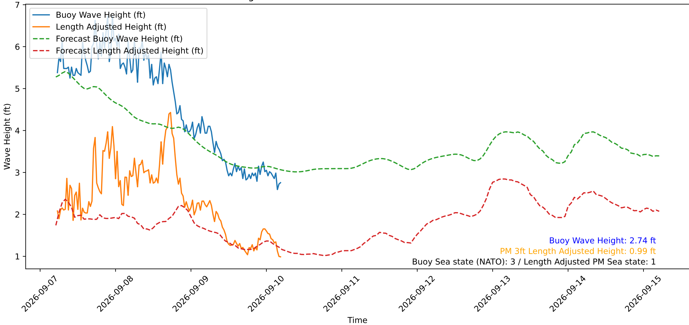
Wave Heights over Time for Red Beach at 2026-09-10 05:10:49
