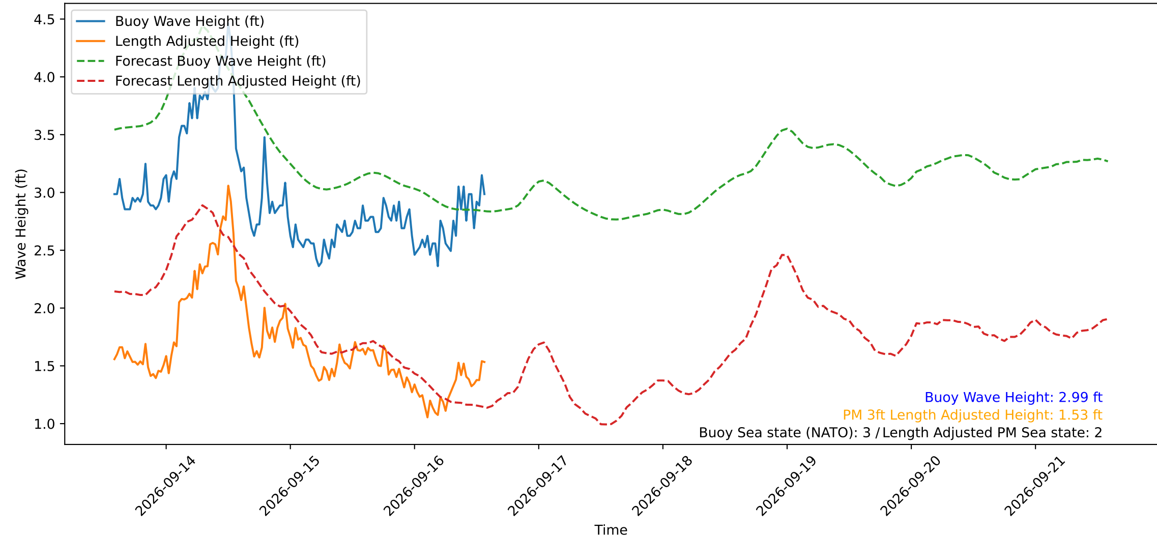
Wave Heights over Time for Oceanside Harbor at 2026-09-16 14:10:29
