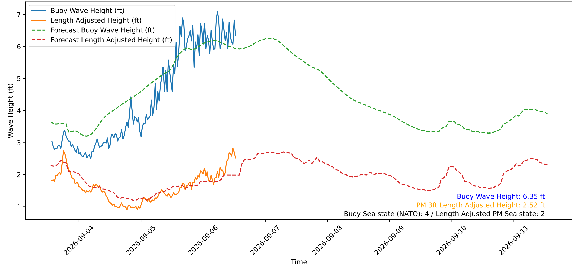
Wave Heights over Time for Green Beach at 2026-09-06 13:11:13
