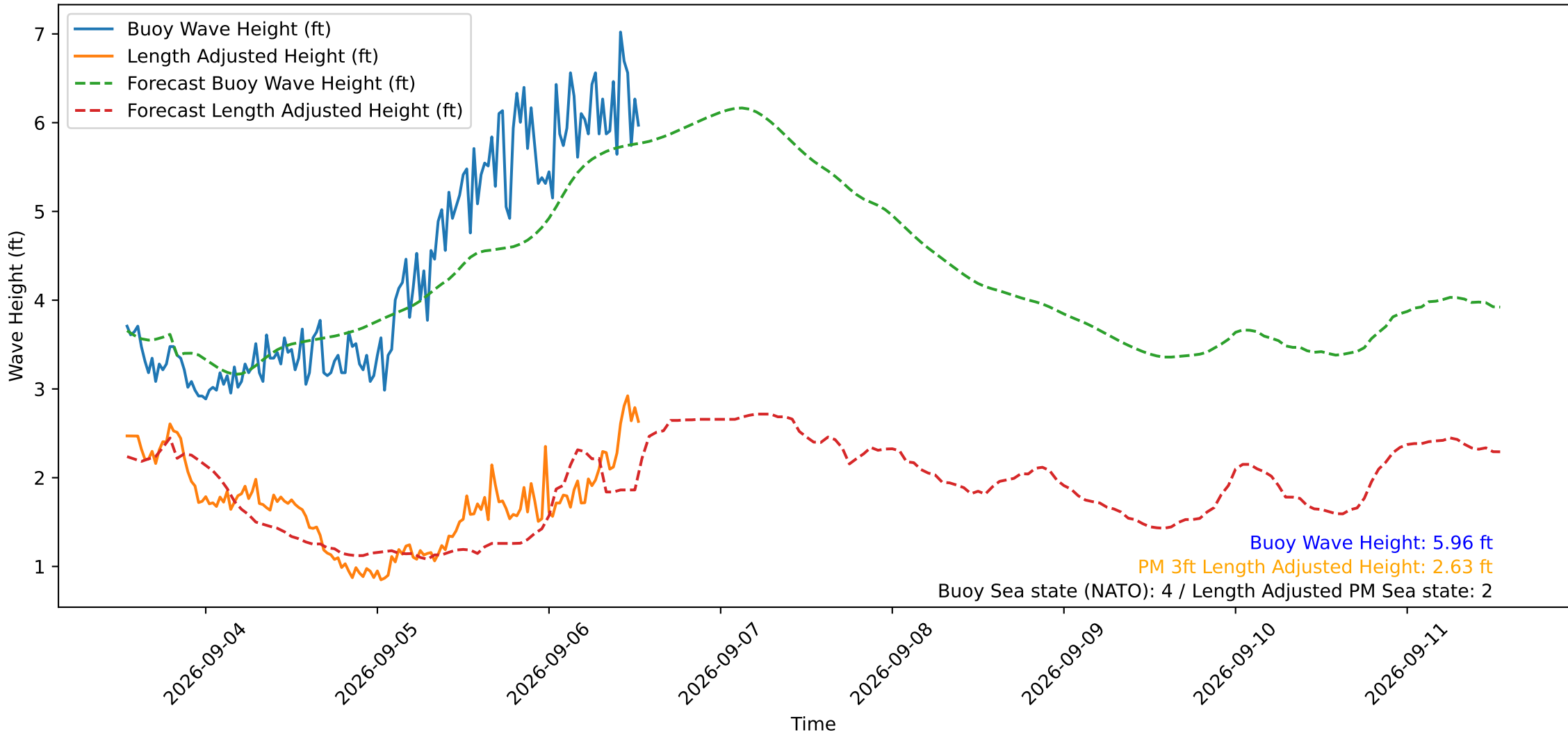
Wave Heights over Time for Oceanside Harbor at 2026-09-06 13:10:30
