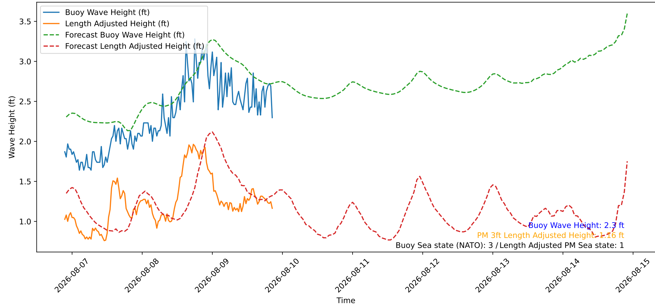
Wave Heights over Time for Oceanside Harbor at 2026-08-09 21:30:26
