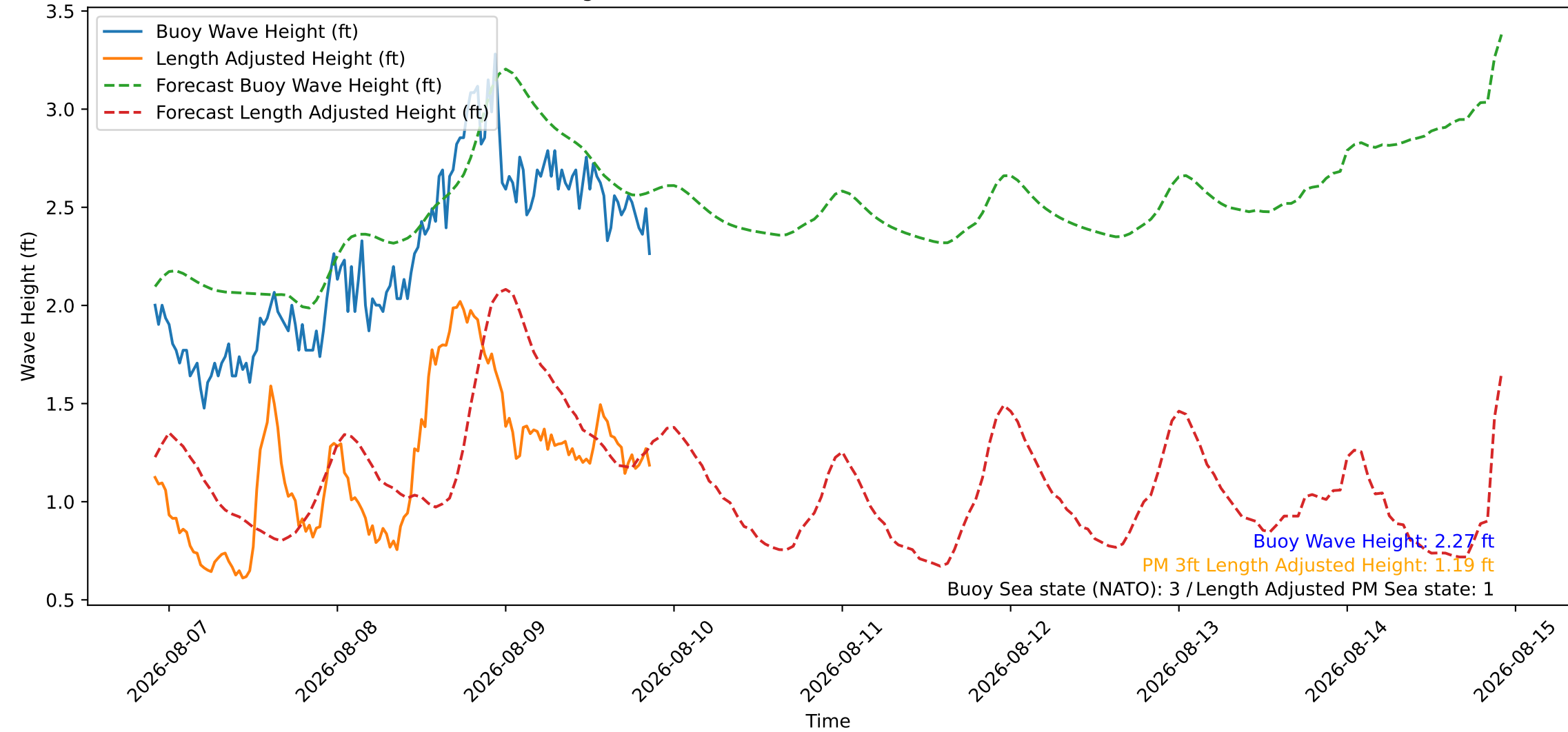
Wave Heights over Time for Red Beach at 2026-08-09 21:30:46
