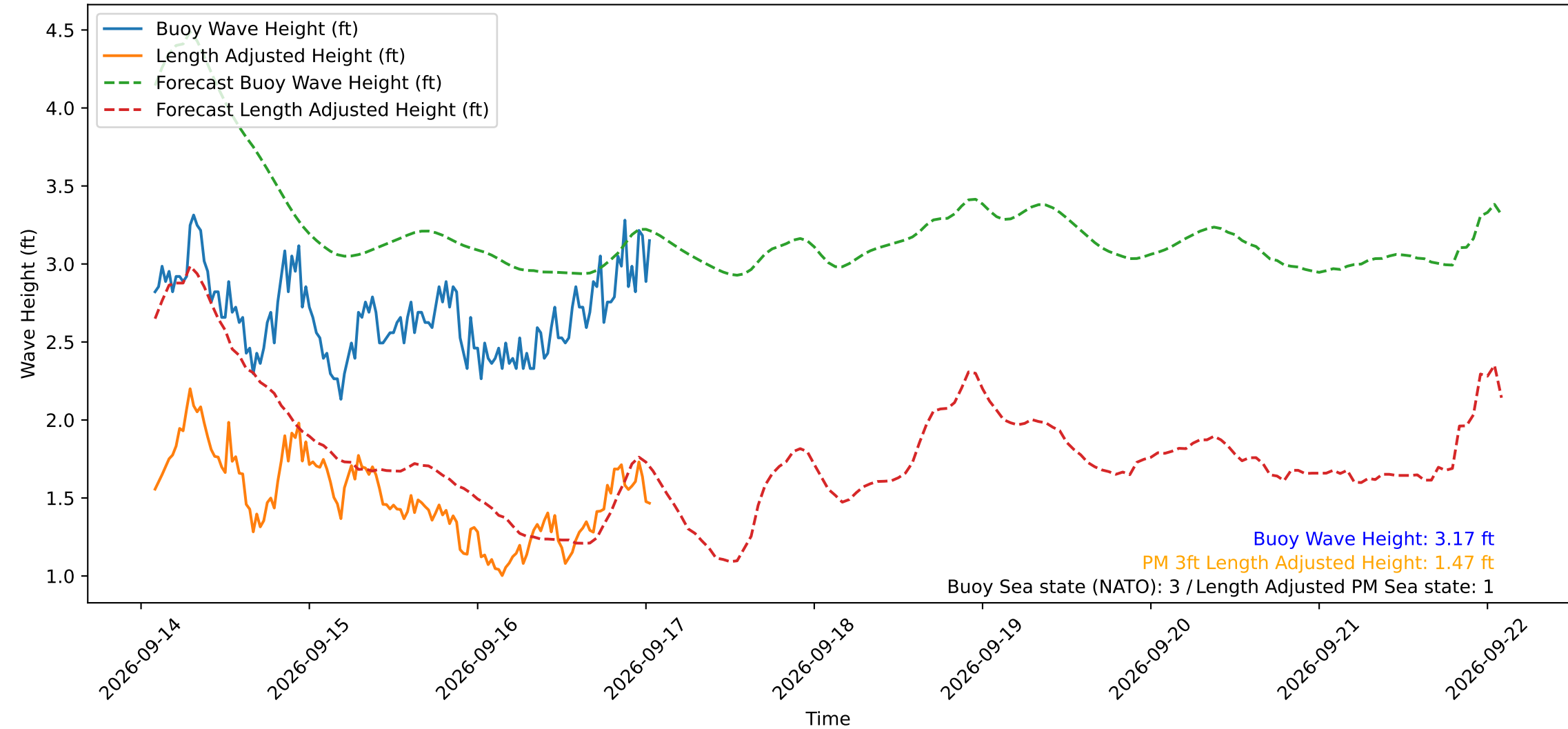
Wave Heights over Time for Green Beach at 2026-09-17 01:31:13
