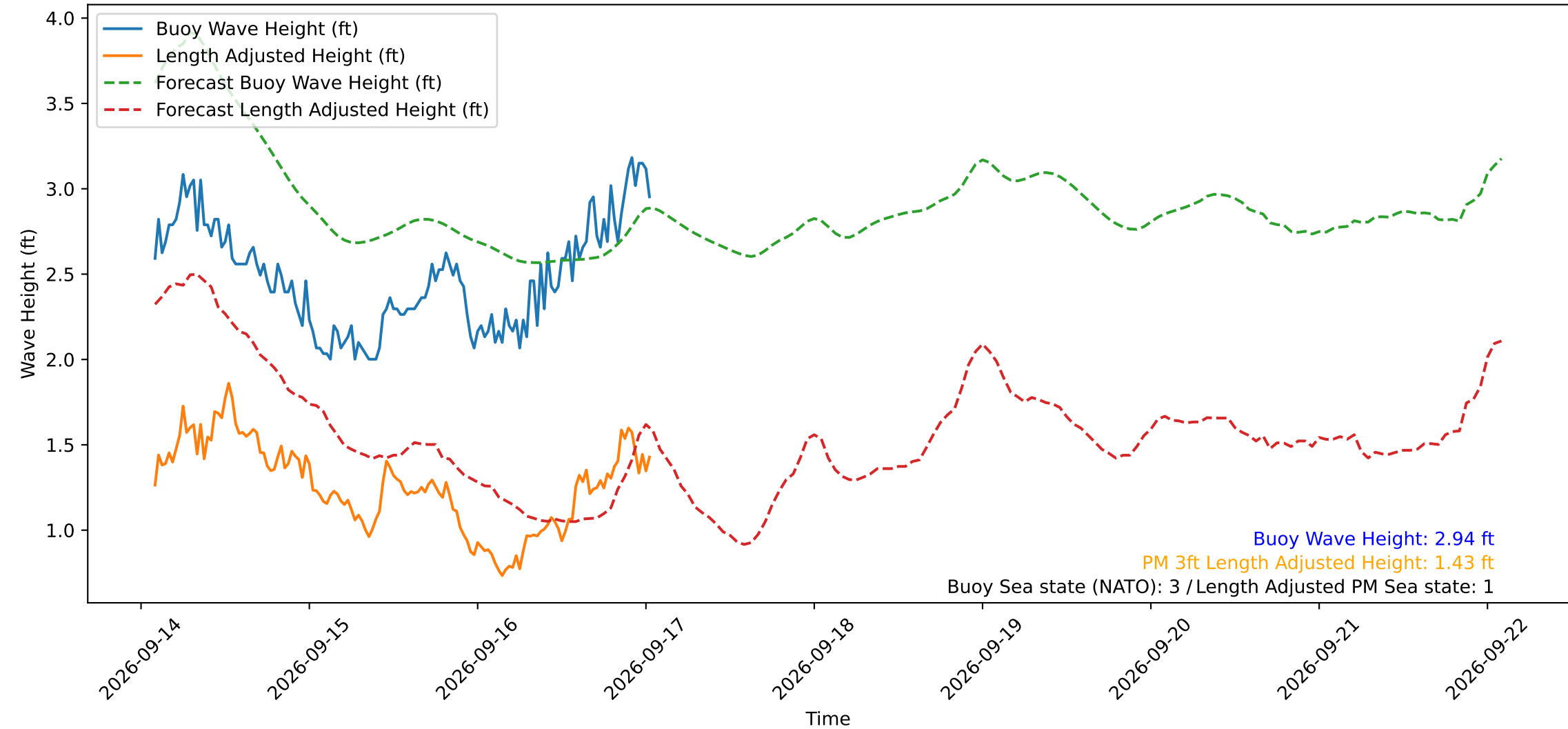
Wave Heights over Time for Red Beach at 2026-09-17 01:30:50
