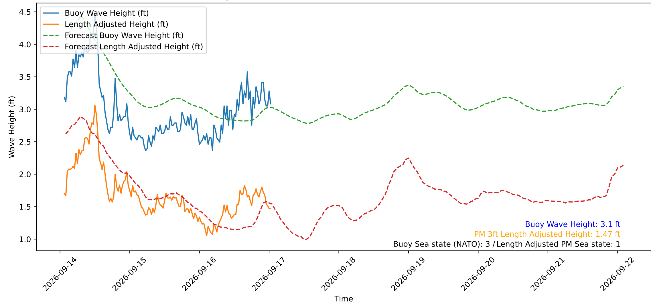
Wave Heights over Time for Oceanside Harbor at 2026-09-17 01:30:30
