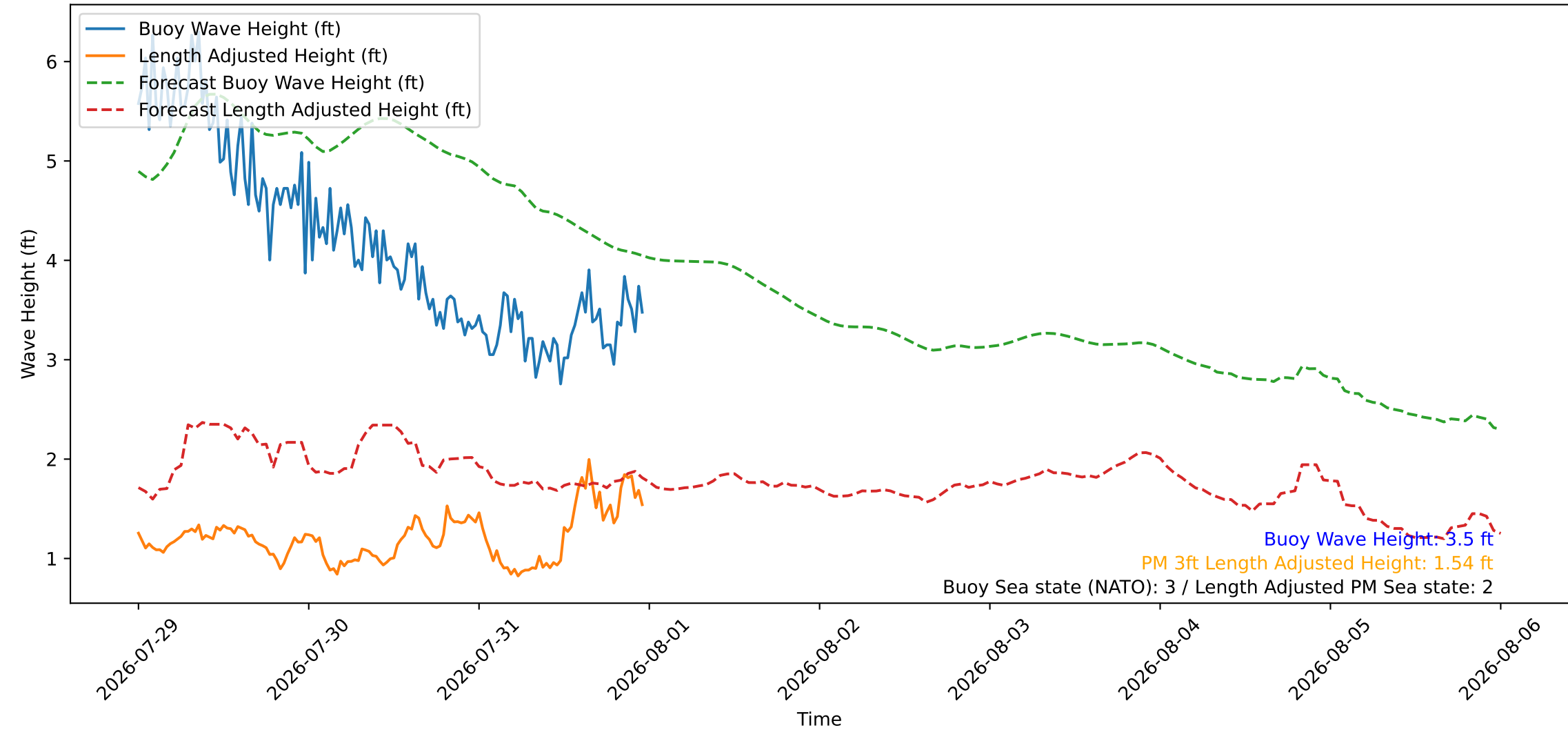
Wave Heights over Time for Green Beach at 2026-08-01 00:01:09
