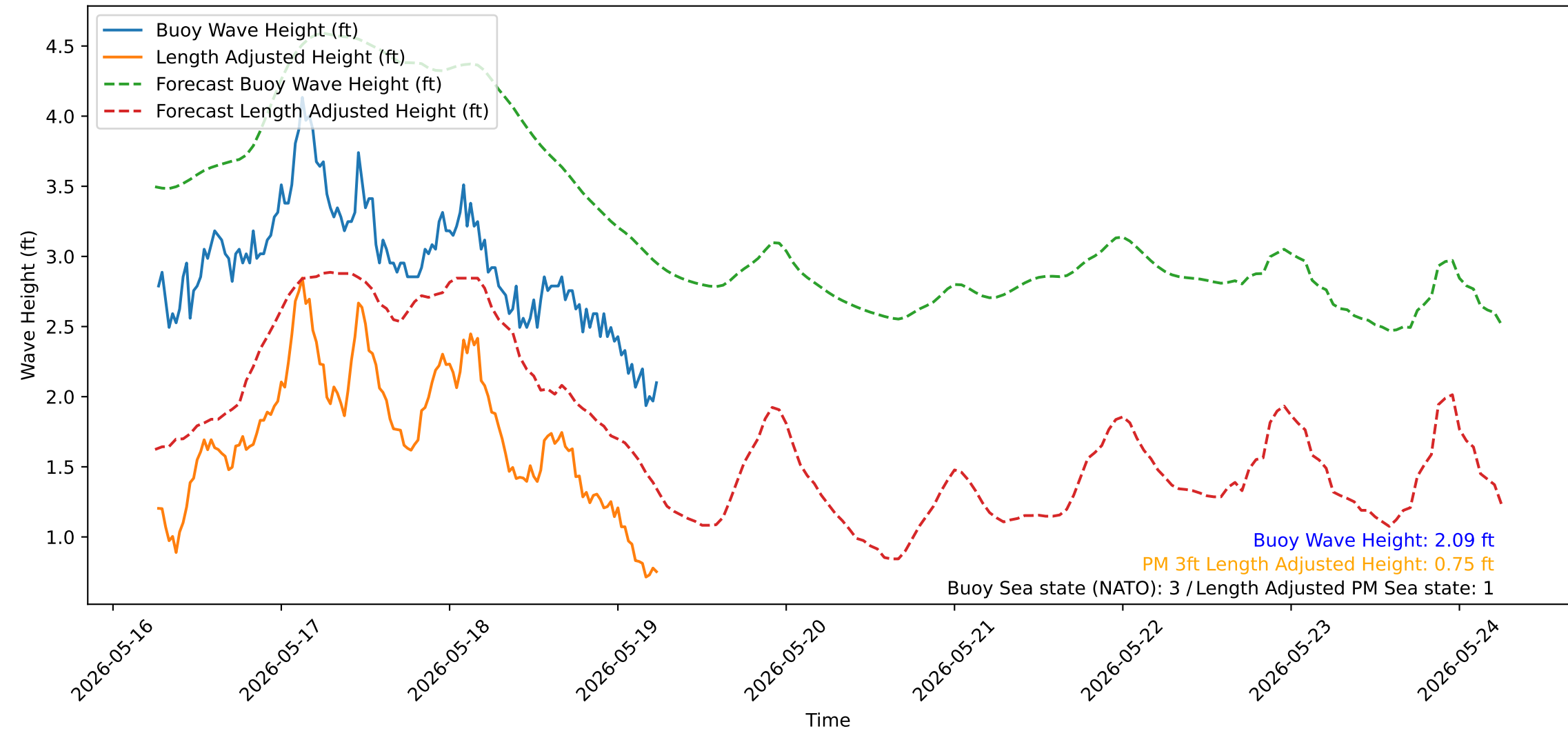
Wave Heights over Time for Red Beach at 2026-05-19 06:20:52
