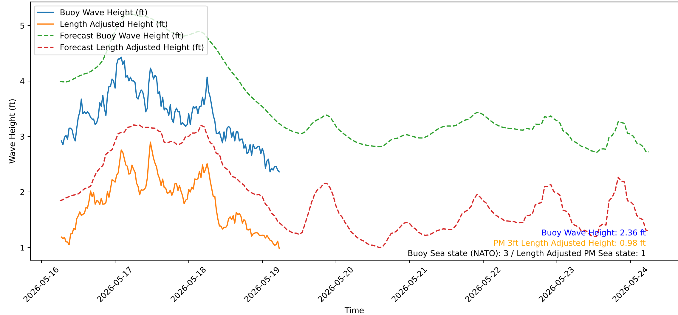
Wave Heights over Time for Green Beach at 2026-05-19 06:21:14
