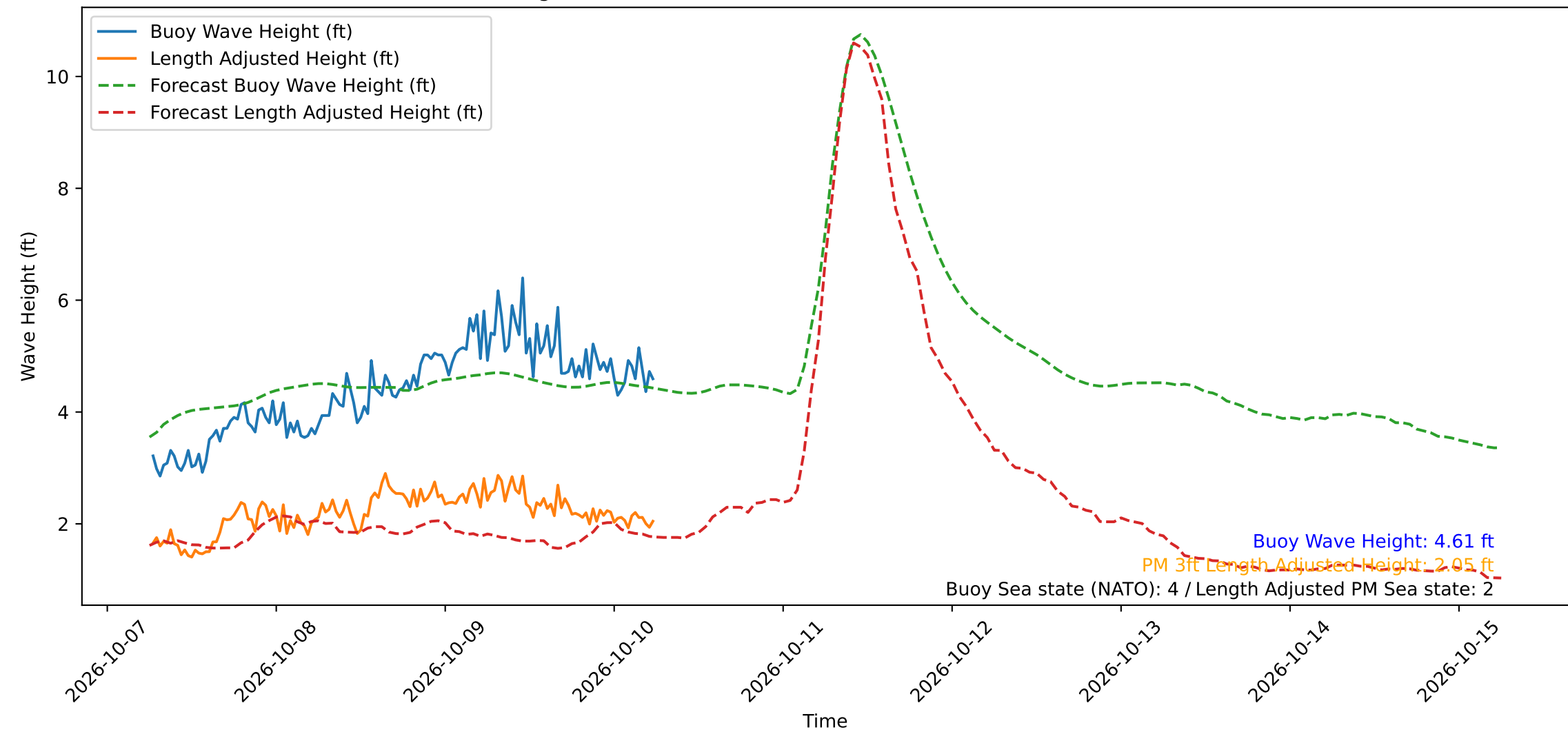
Wave Heights over Time for Oceanside Harbor at 2026-10-10 06:20:29
