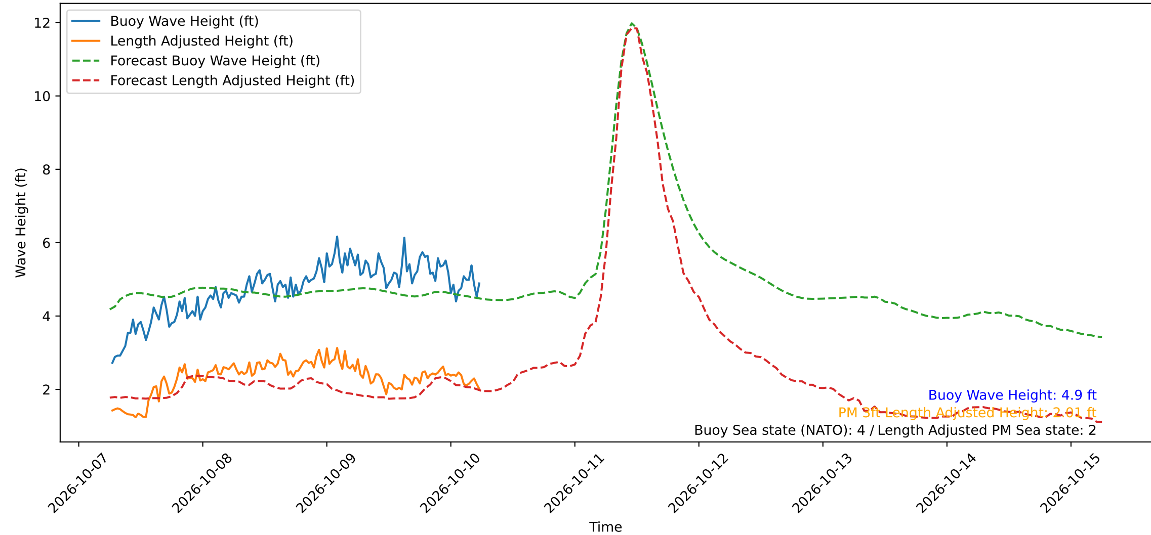
Wave Heights over Time for Green Beach at 2026-10-10 06:21:15
