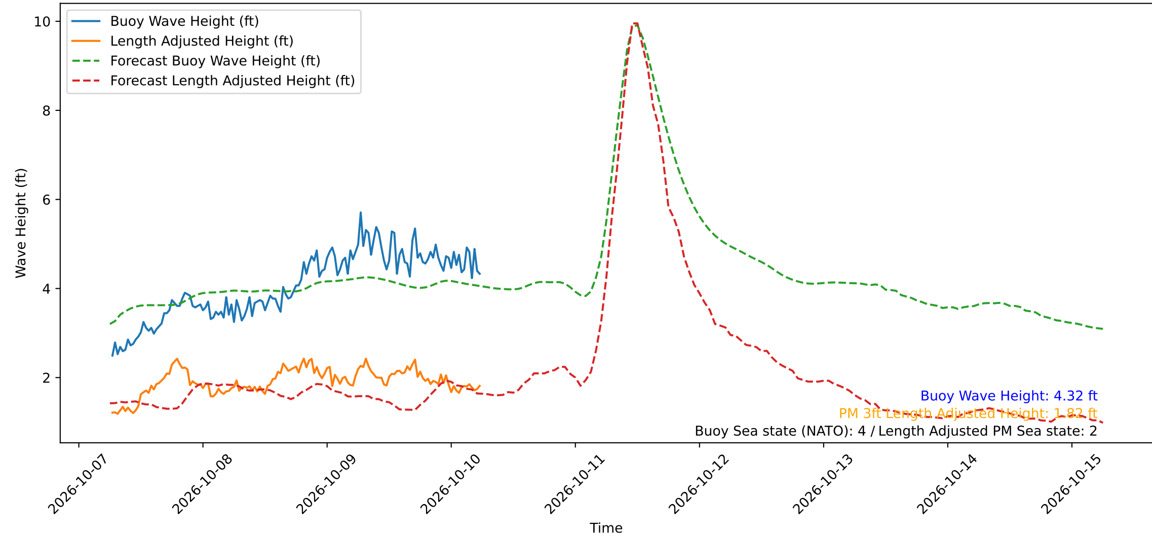
Wave Heights over Time for Red Beach at 2026-10-10 06:20:51
