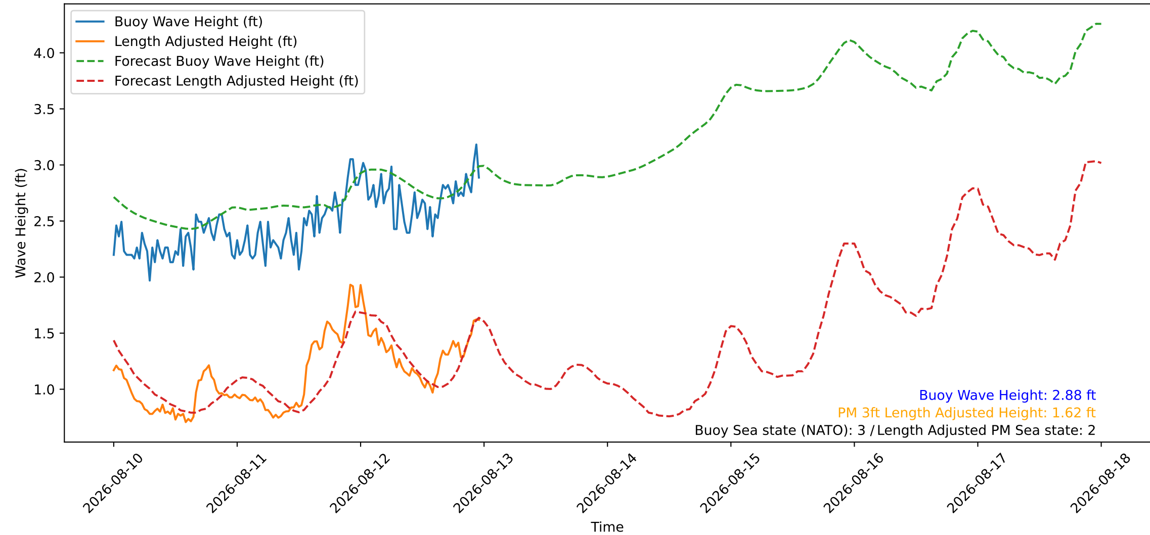
Wave Heights over Time for Oceanside Harbor at 2026-08-13 00:00:26
