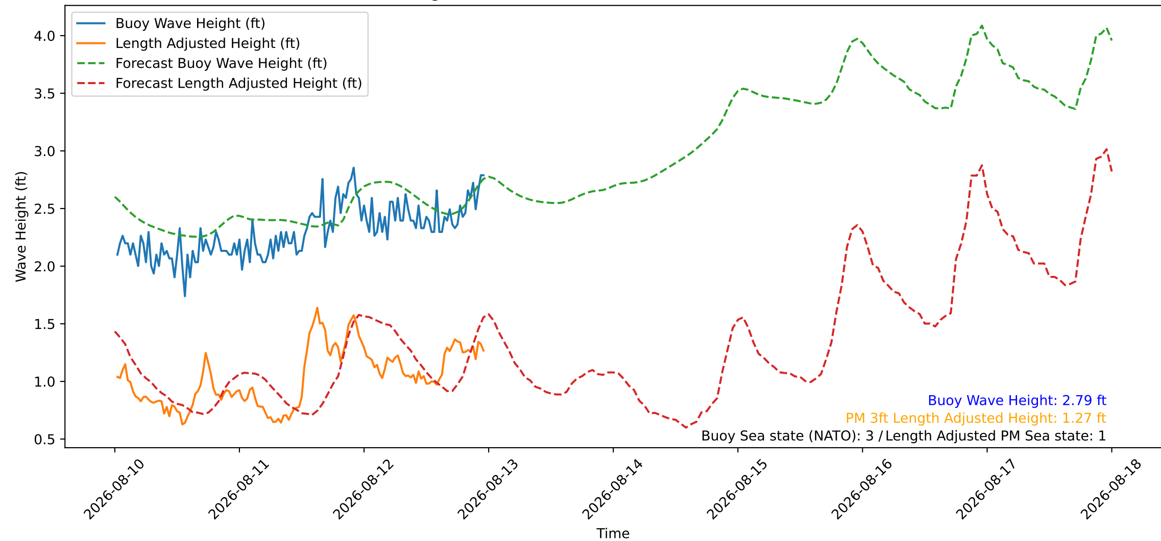
Wave Heights over Time for Red Beach at 2026-08-13 00:00:46
