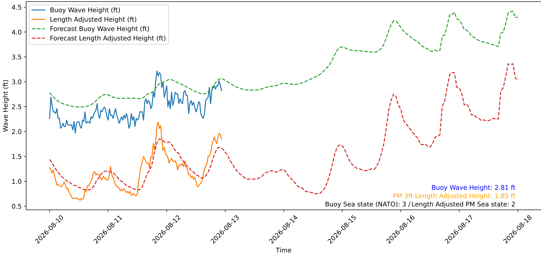
Wave Heights over Time for Green Beach at 2026-08-13 00:01:08
