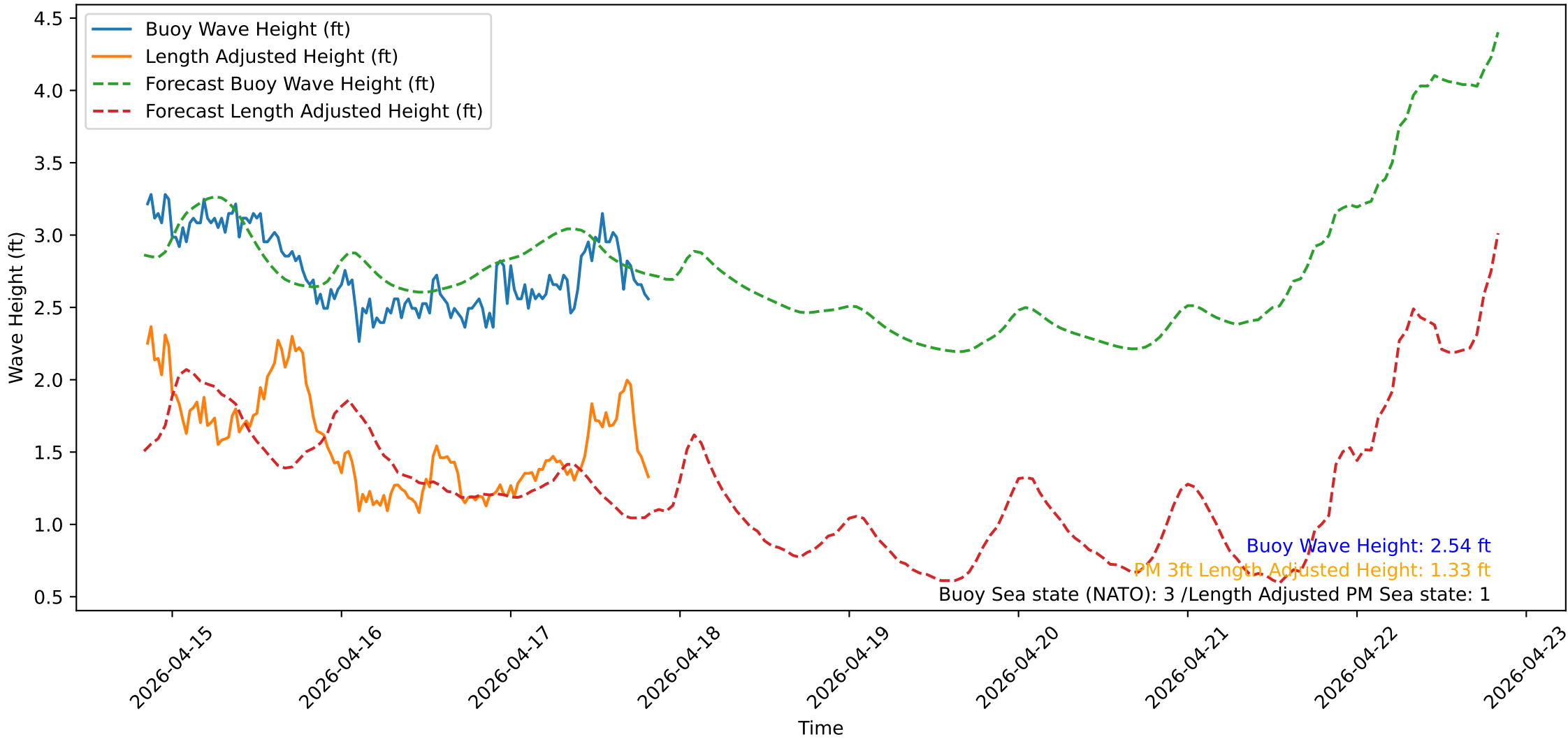
Wave Heights over Time for Red Beach at 2026-04-17 20:10:52
