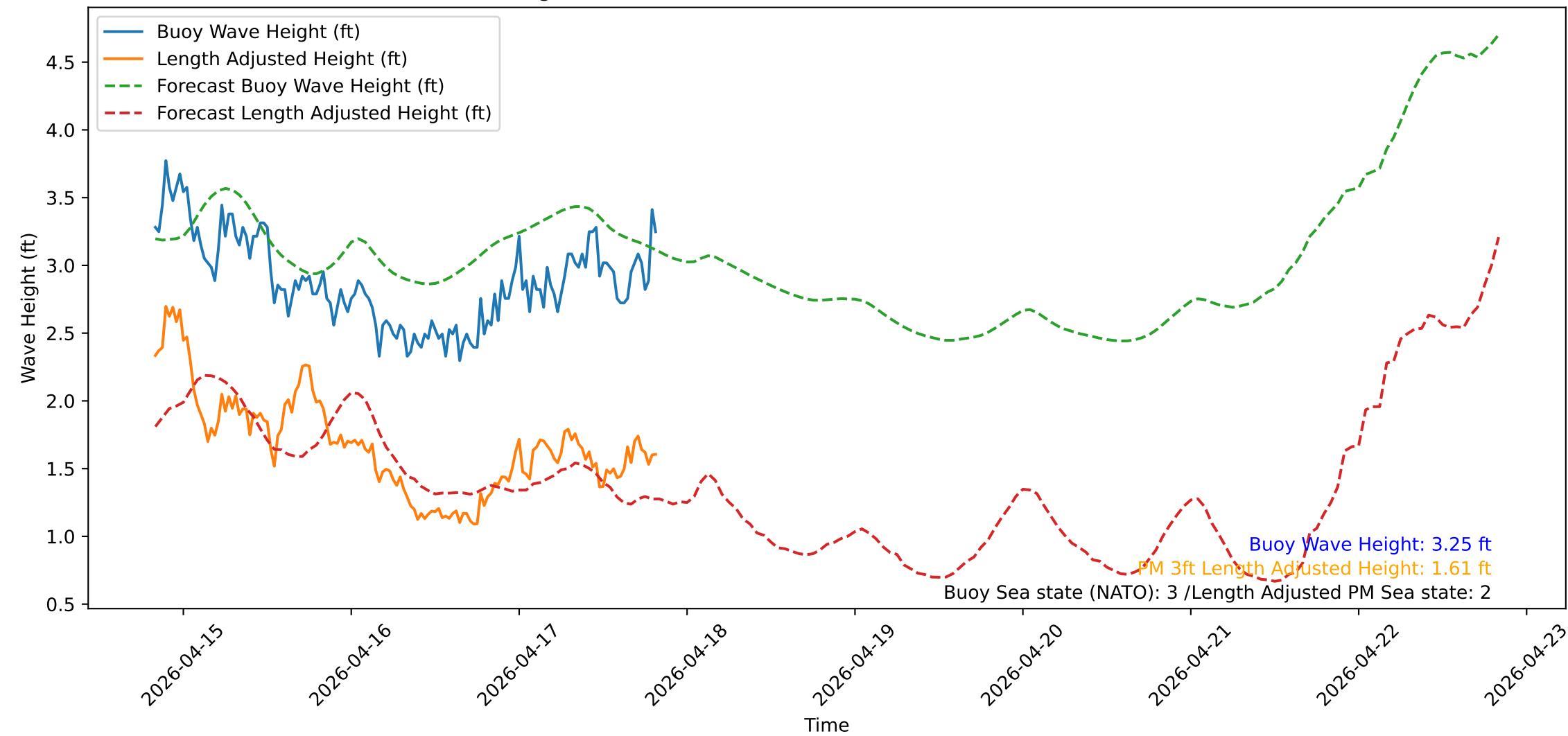
Wave Heights over Time for Oceanside Harbor at 2026-04-17 20:10:32
