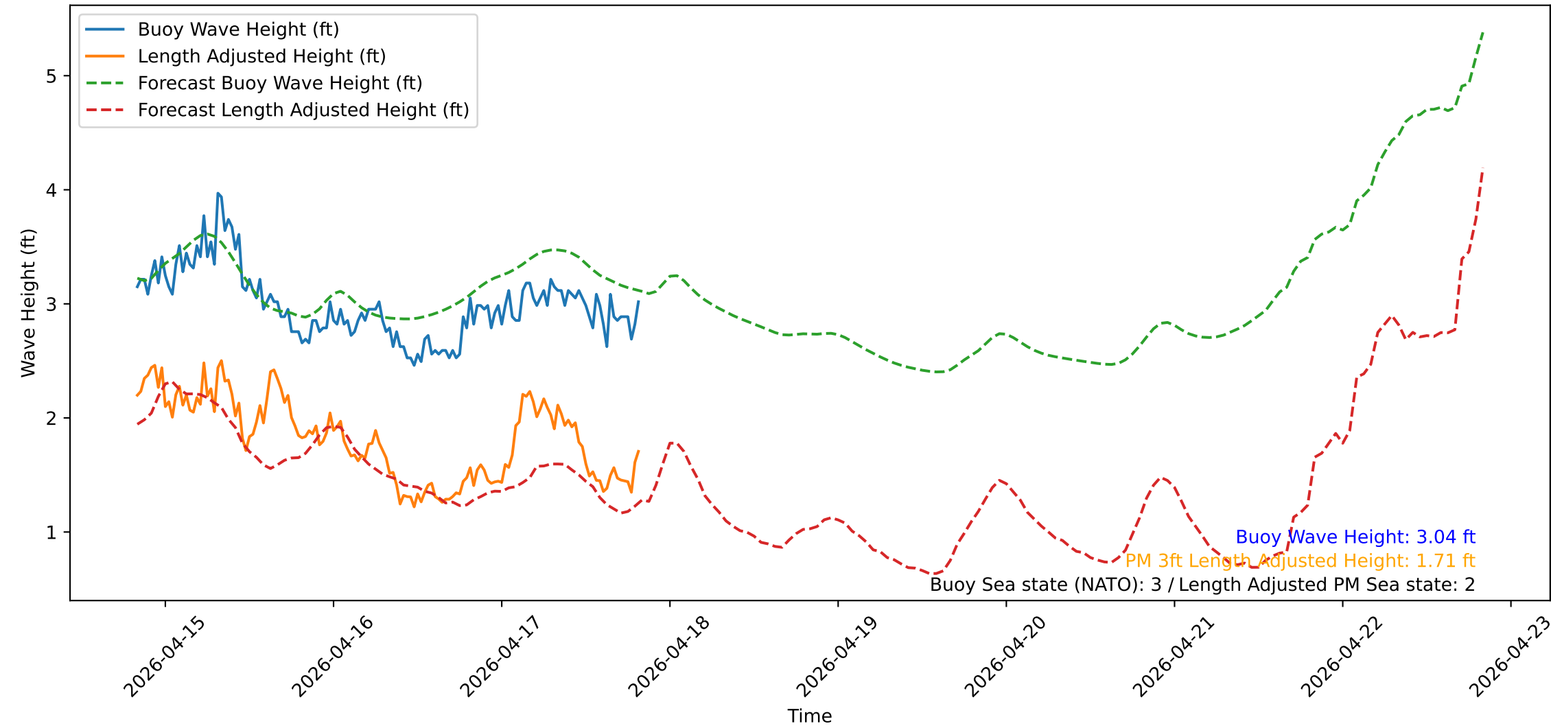
Wave Heights over Time for Green Beach at 2026-04-17 20:11:15
