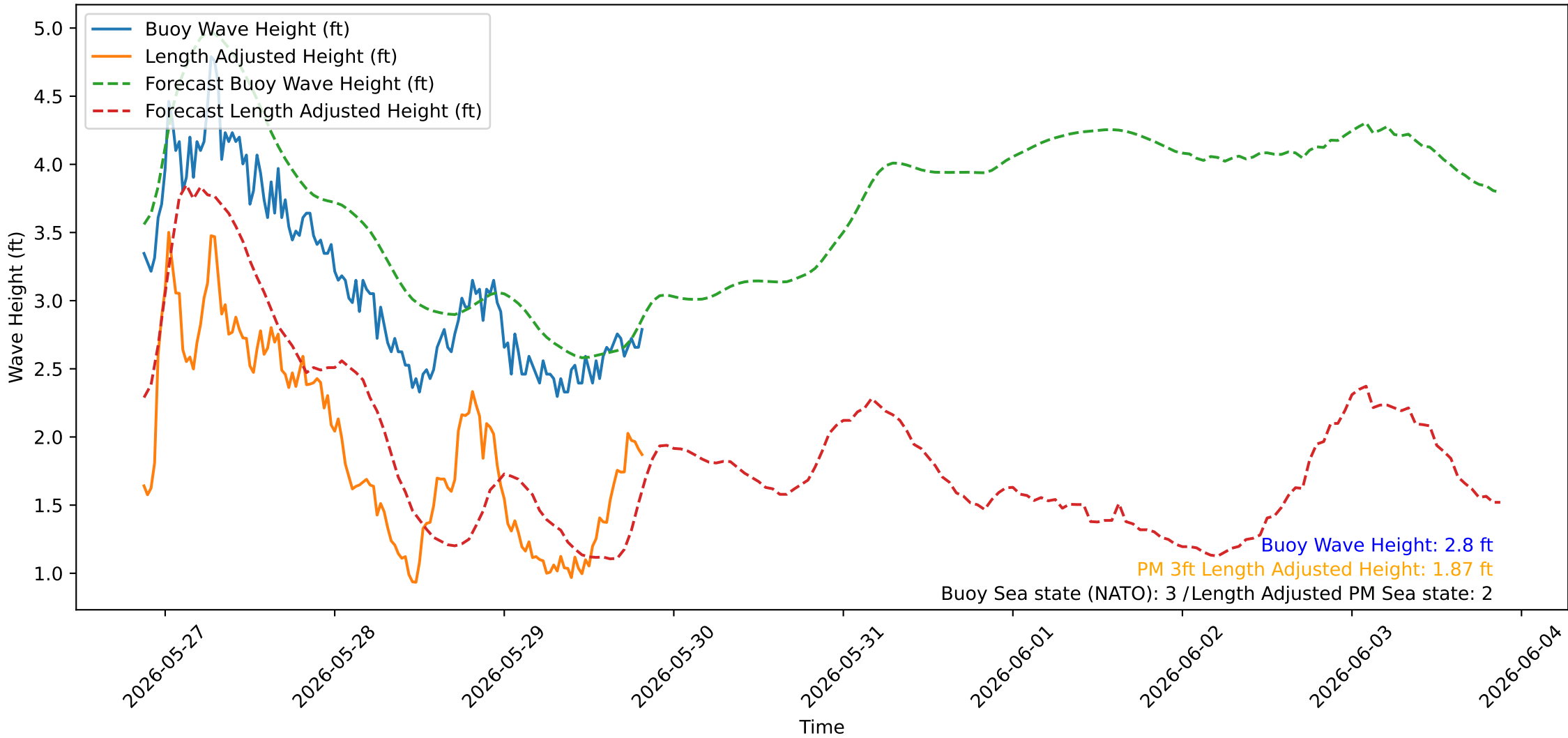
Wave Heights over Time for Red Beach at 2026-05-29 20:30:42
