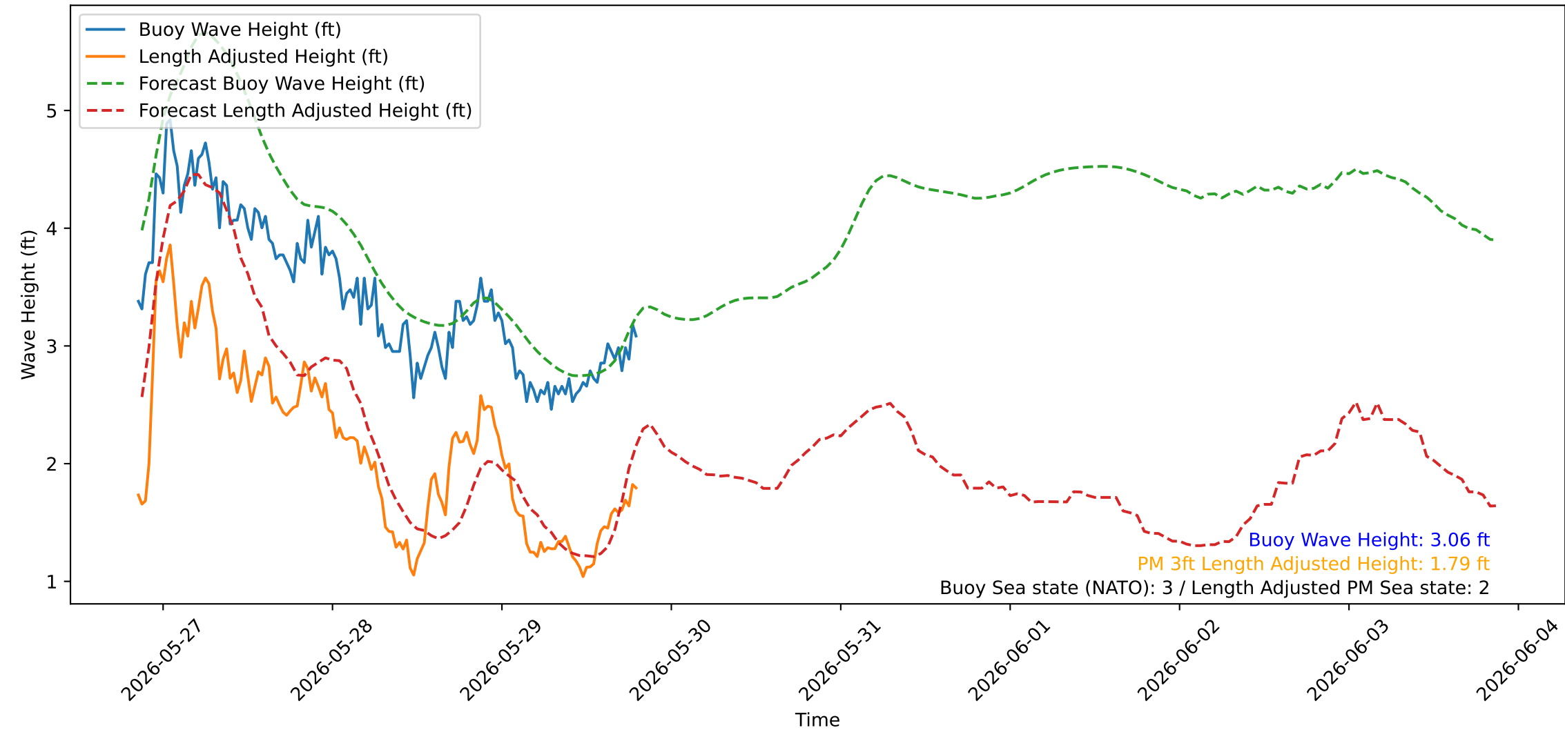
Wave Heights over Time for Green Beach at 2026-05-29 20:31:05
