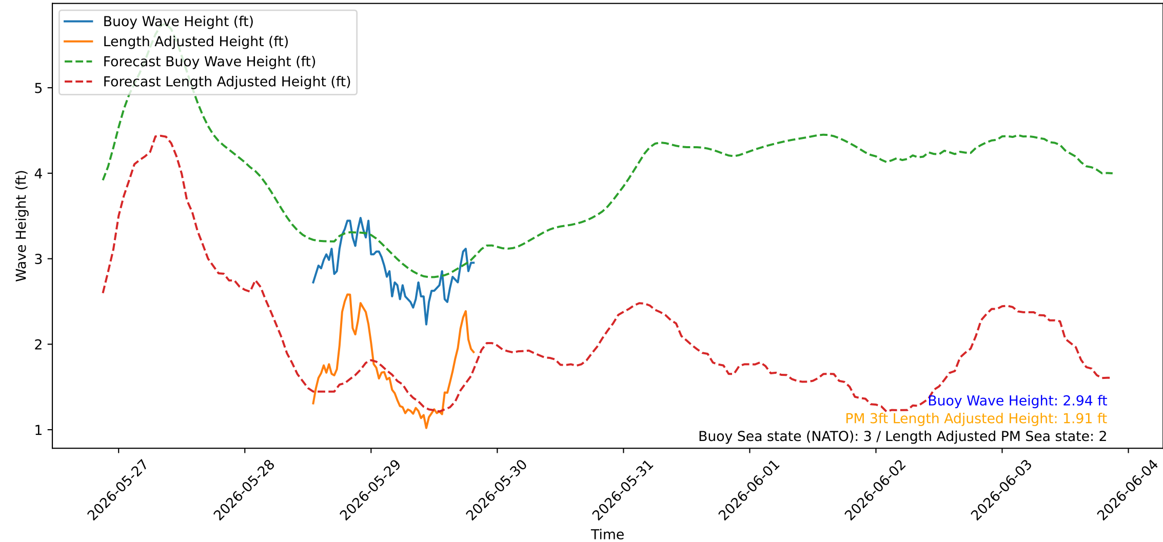
Wave Heights over Time for Oceanside Harbor at 2026-05-29 20:30:22
