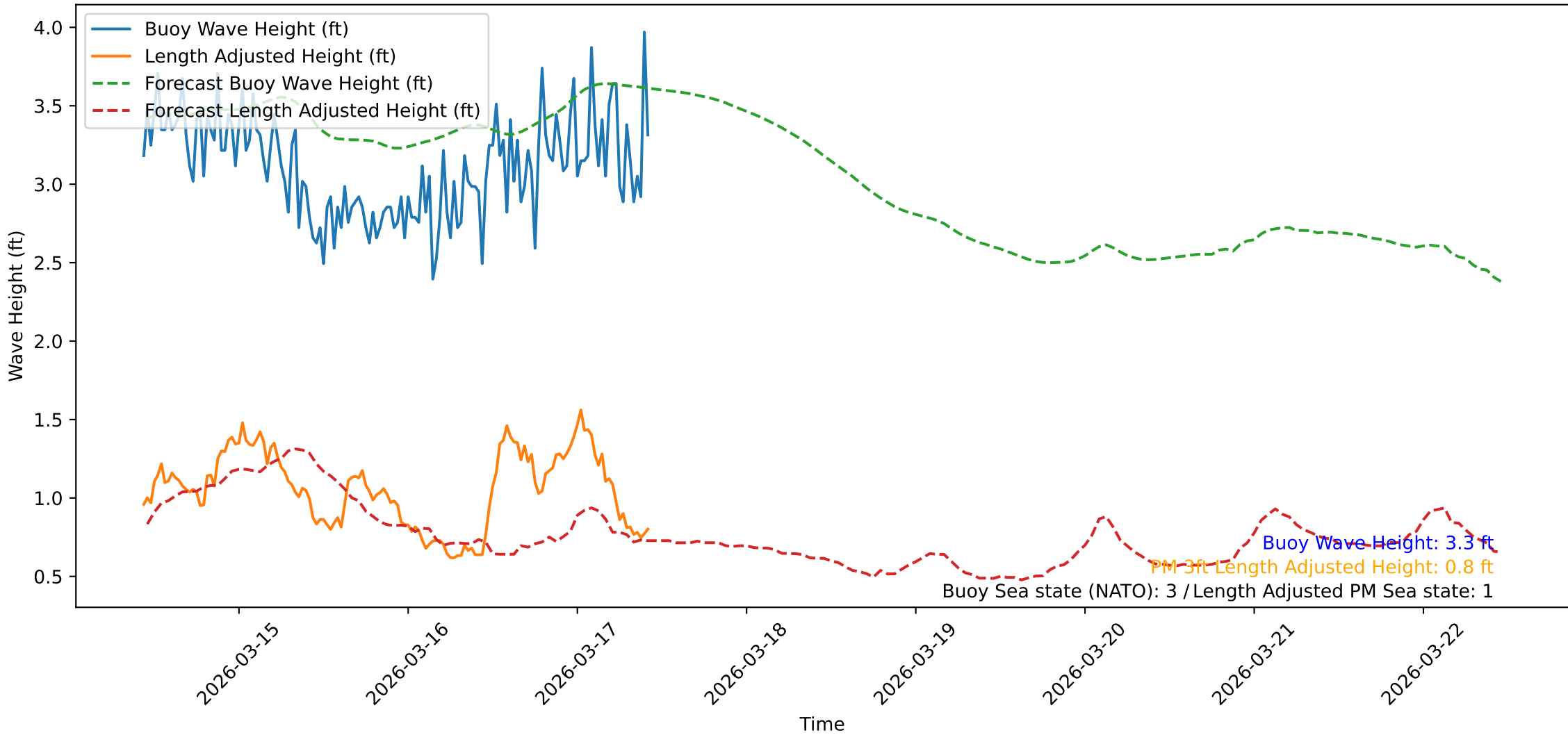
Wave Heights over Time for Oceanside Harbor at 2026-03-17 10:40:43
