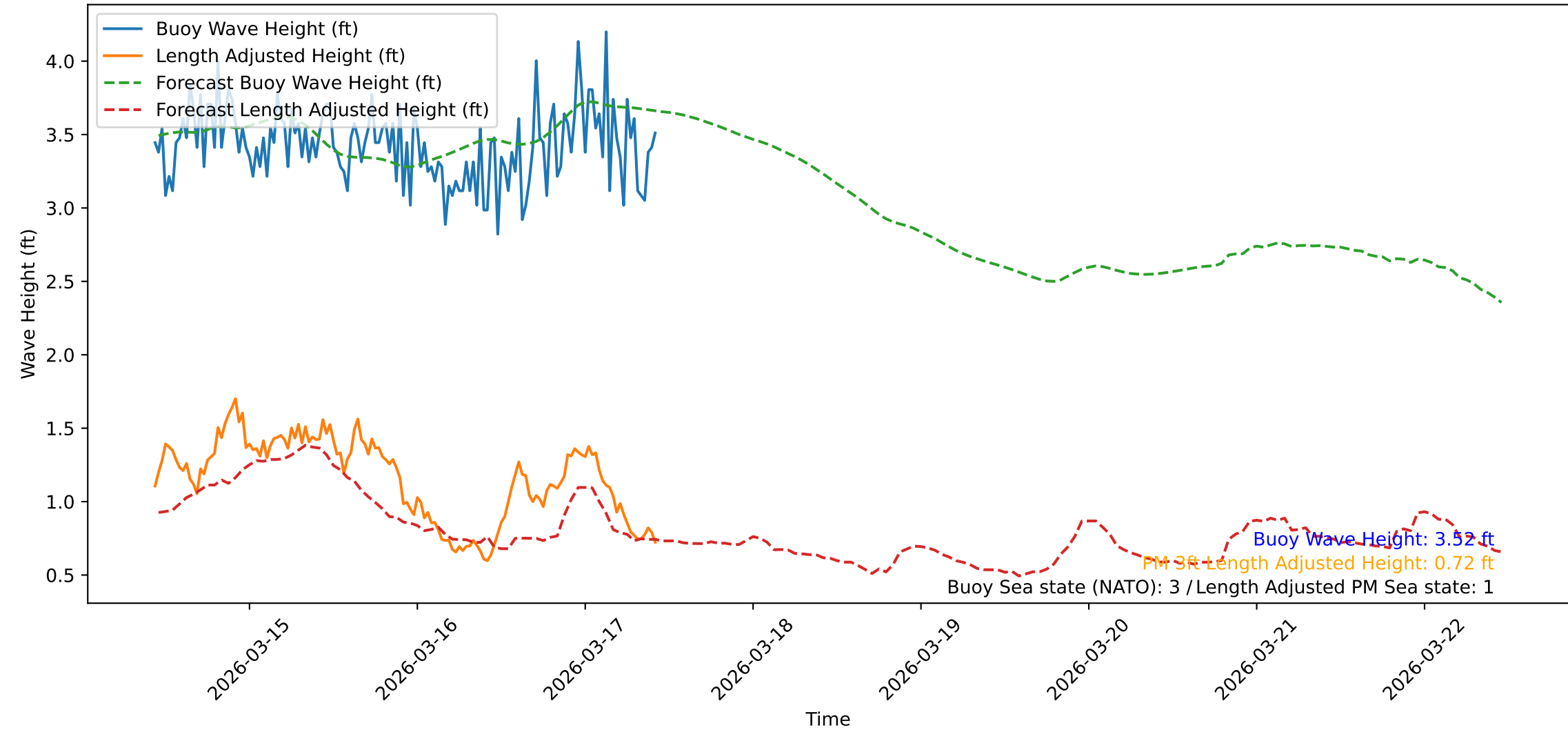
Wave Heights over Time for Green Beach at 2026-03-17 10:41:46
