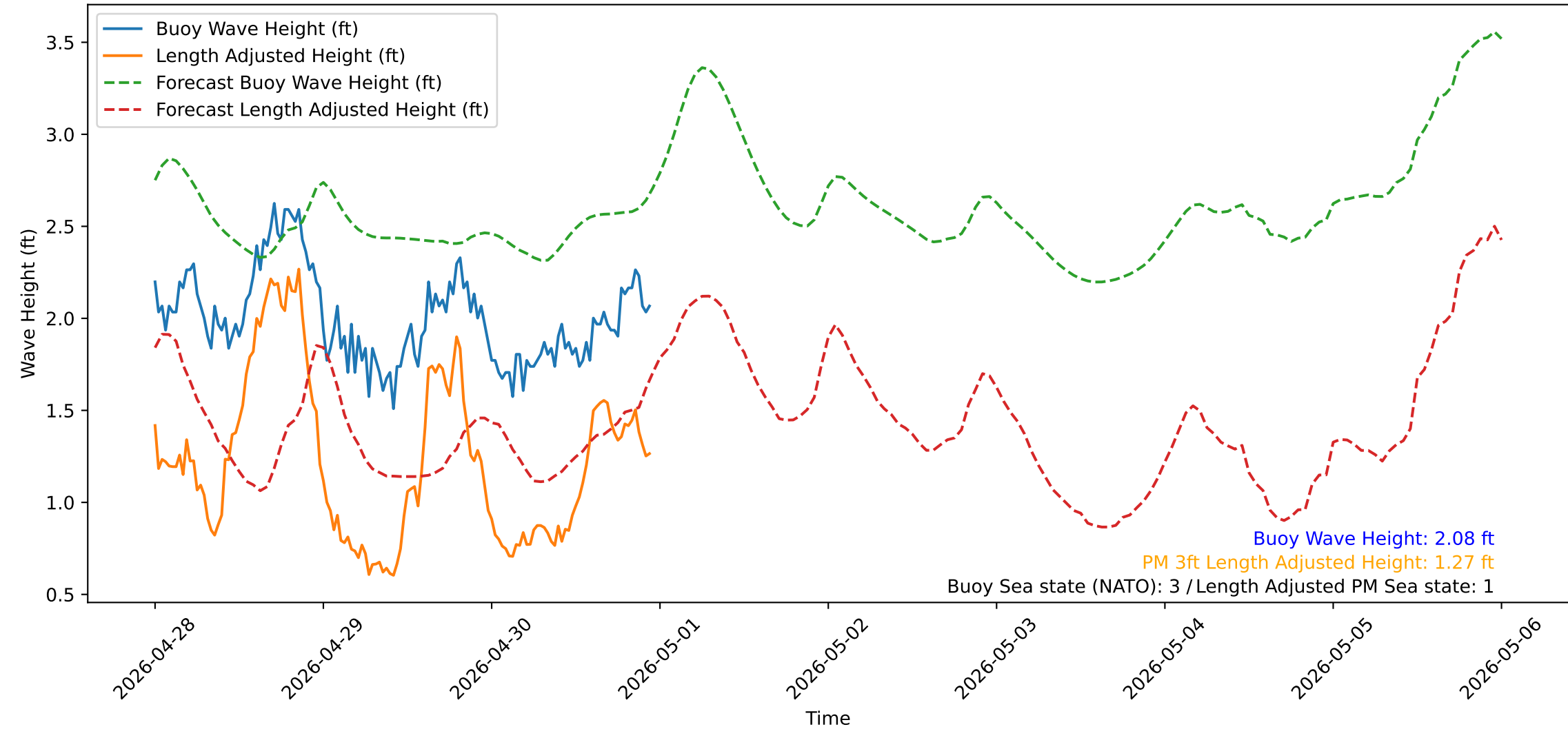
Wave Heights over Time for Red Beach at 2026-04-30 23:30:50
