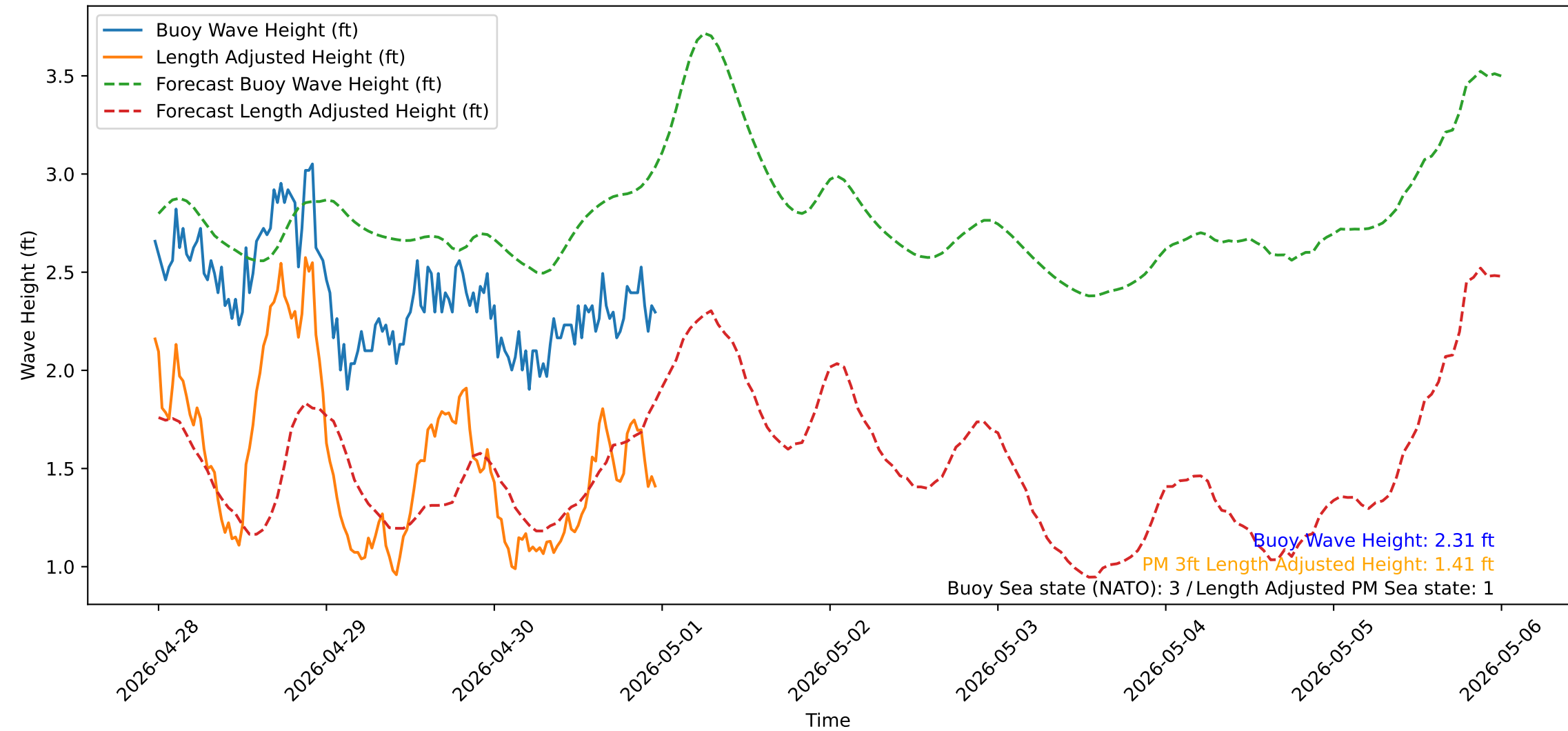
Wave Heights over Time for Oceanside Harbor at 2026-04-30 23:30:31
