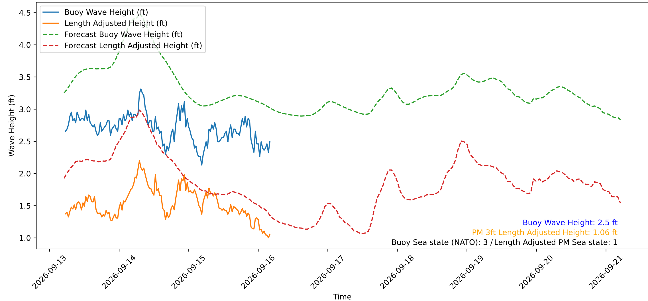
Wave Heights over Time for Green Beach at 2026-09-16 05:01:11
