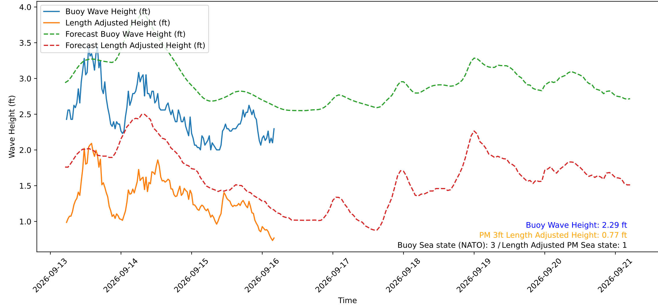
Wave Heights over Time for Red Beach at 2026-09-16 05:00:49
