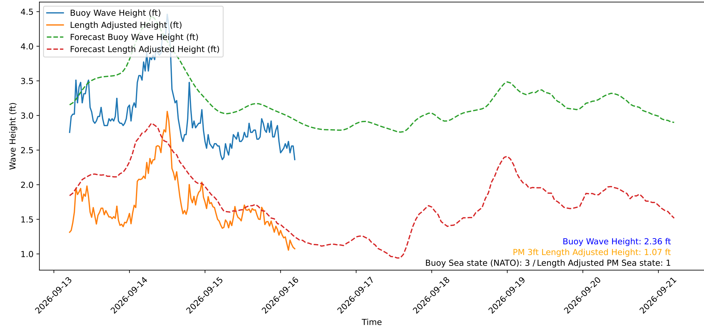
Wave Heights over Time for Oceanside Harbor at 2026-09-16 05:00:30
