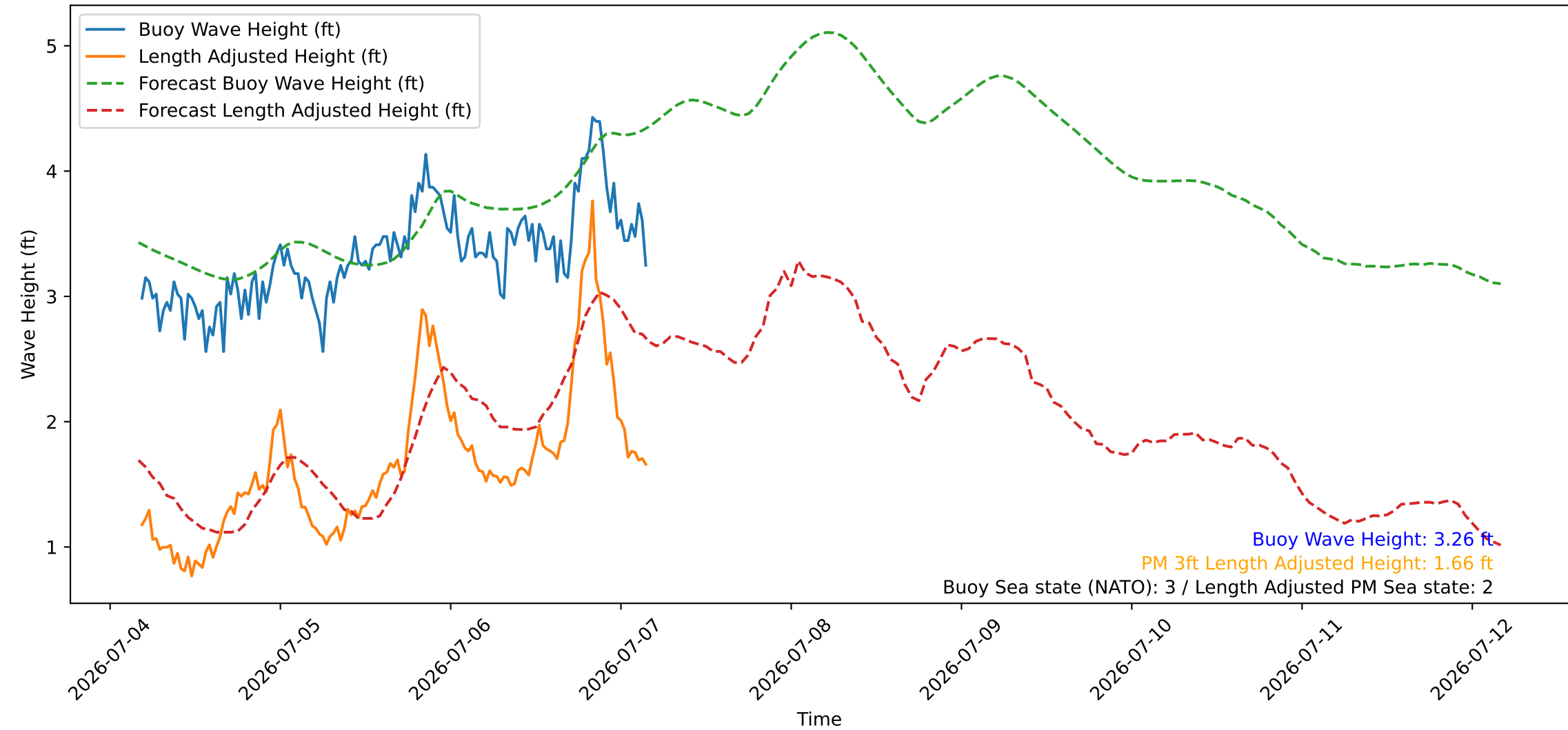
Wave Heights over Time for Green Beach at 2026-07-07 04:21:09
