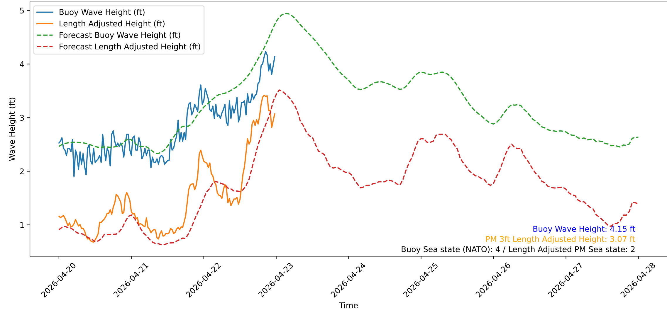
Wave Heights over Time for Oceanside Harbor at 2026-04-23 00:10:31
