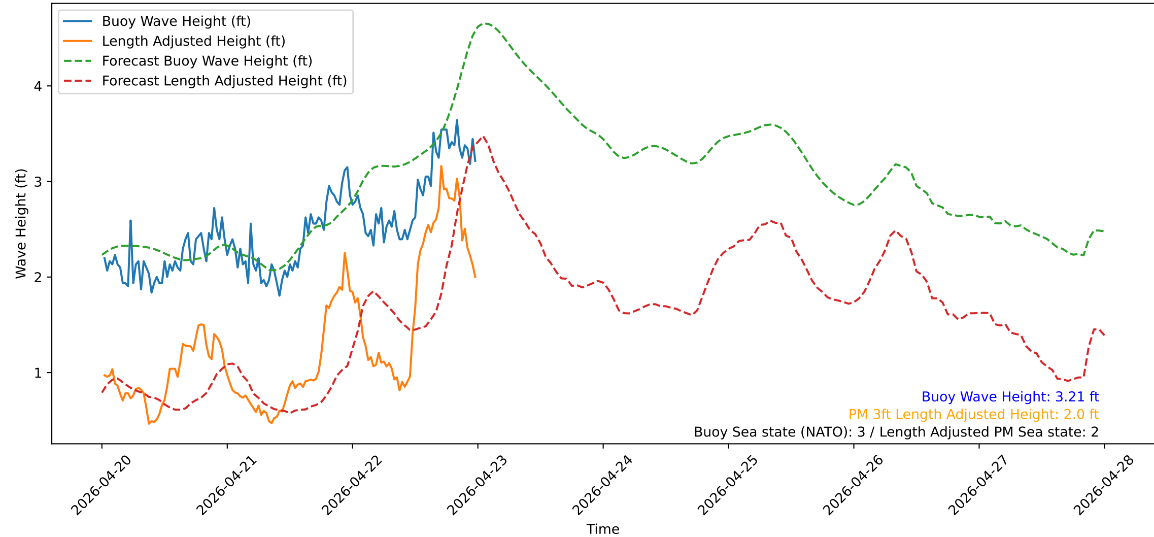
Wave Heights over Time for Red Beach at 2026-04-23 00:10:51
