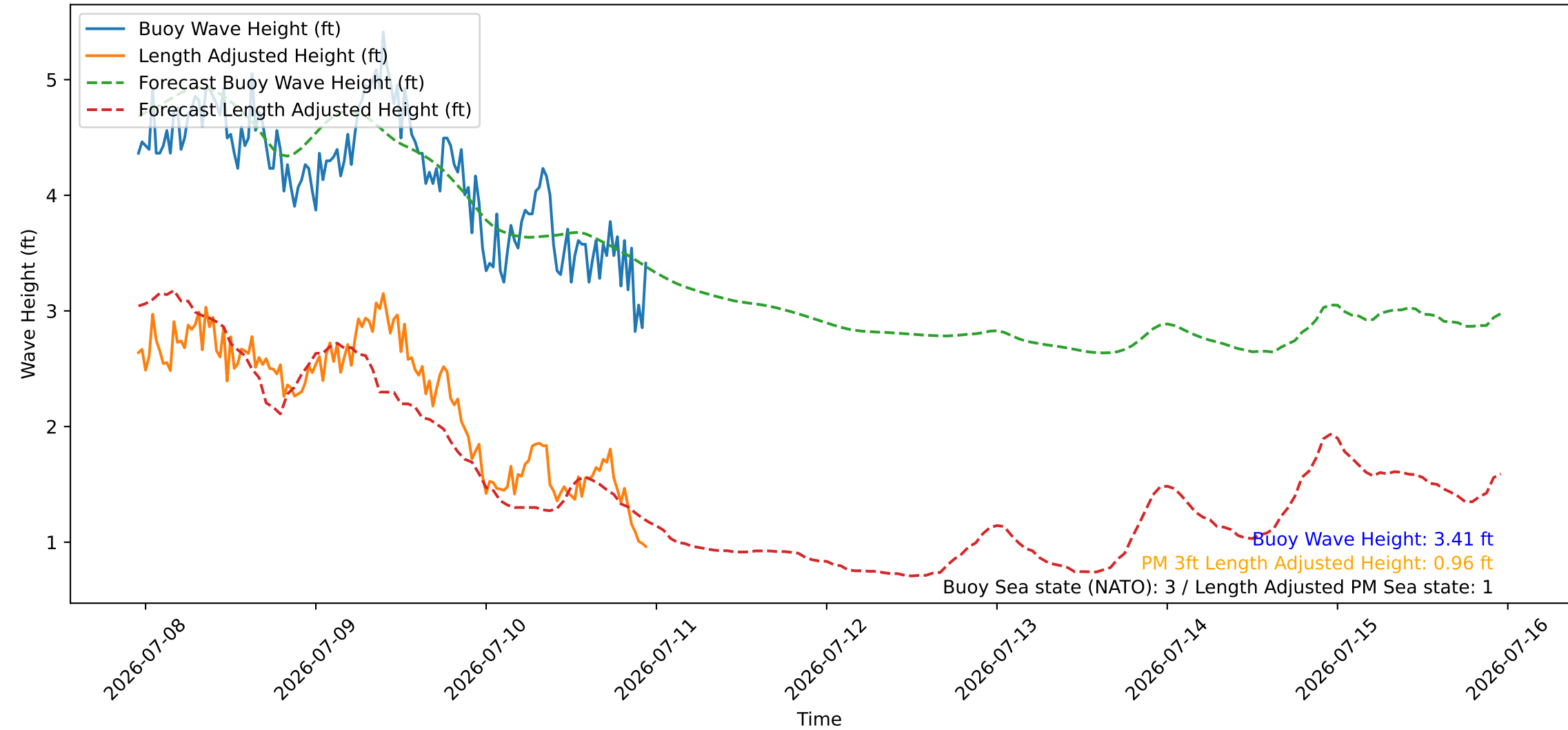
Wave Heights over Time for Oceanside Harbor at 2026-07-10 23:10:25
