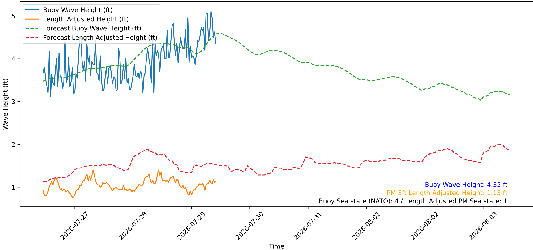
Wave Heights over Time for Red Beach at 2026-07-29 10:50:48
