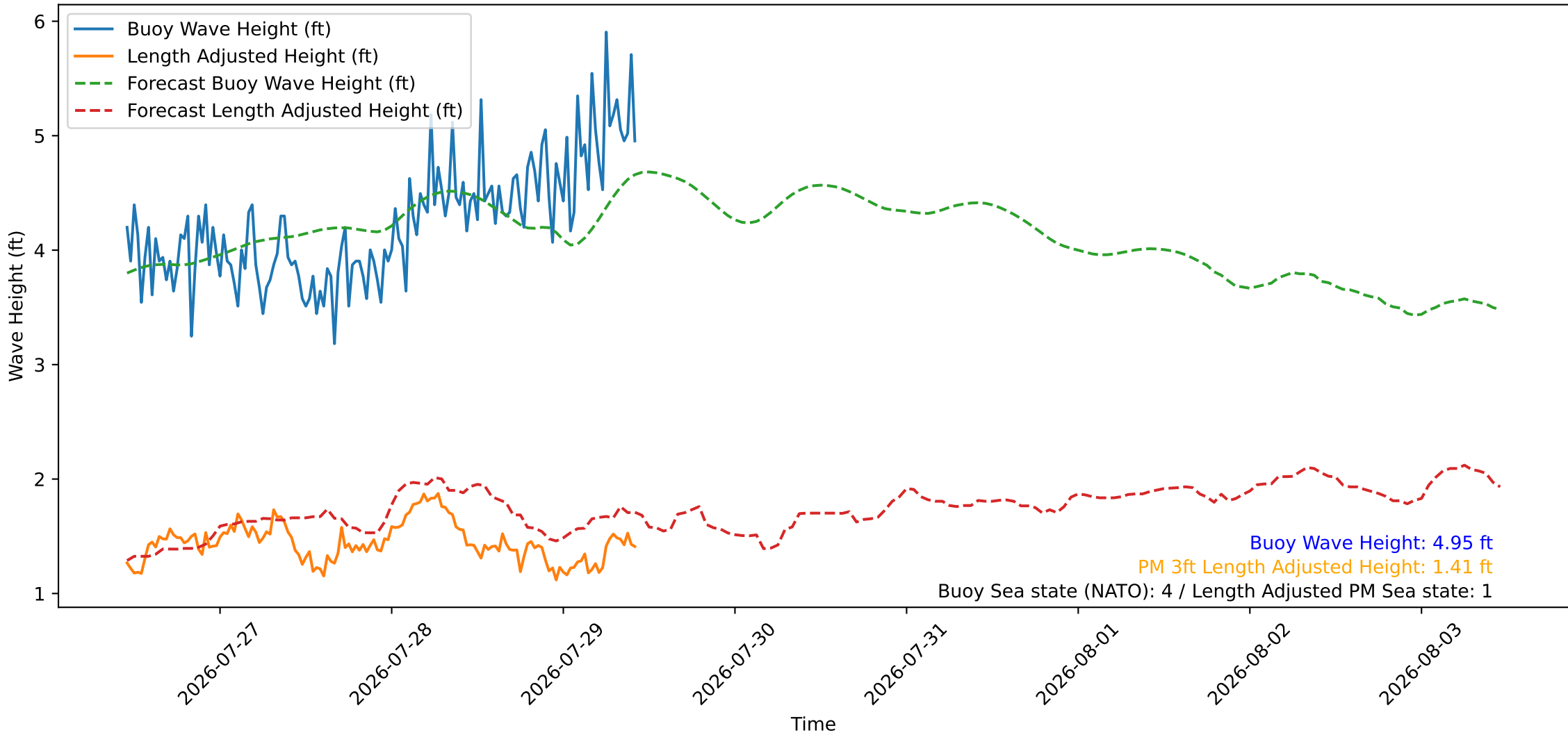
Wave Heights over Time for Oceanside Harbor at 2026-07-29 10:50:27
