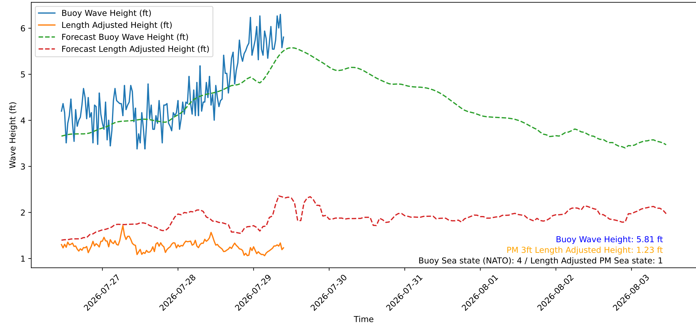
Wave Heights over Time for Green Beach at 2026-07-29 10:51:10
