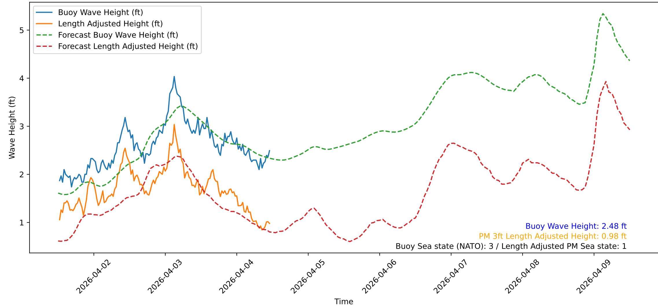
Wave Heights over Time for Oceanside Harbor at 2026-04-04 12:20:31
