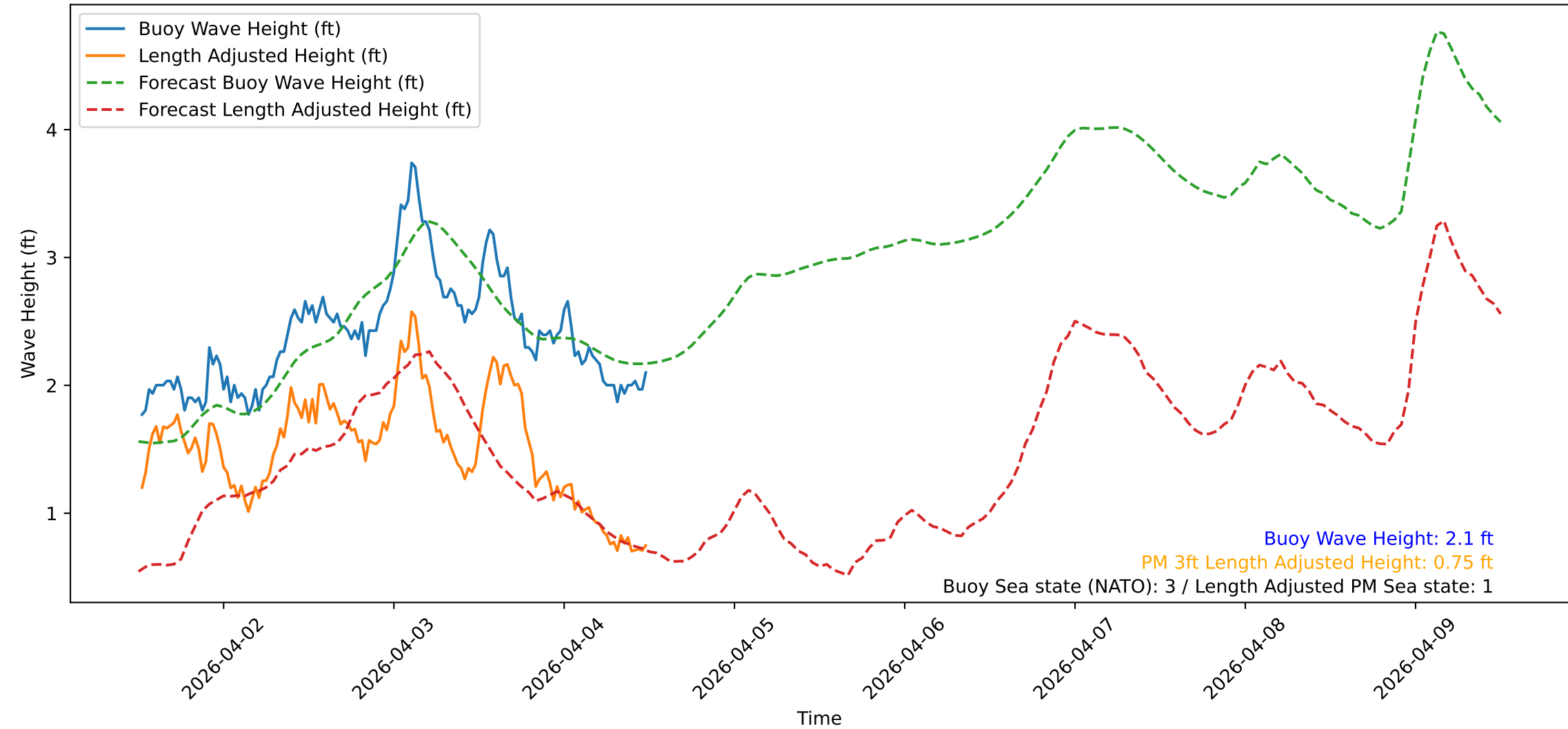
Wave Heights over Time for Red Beach at 2026-04-04 12:20:47
