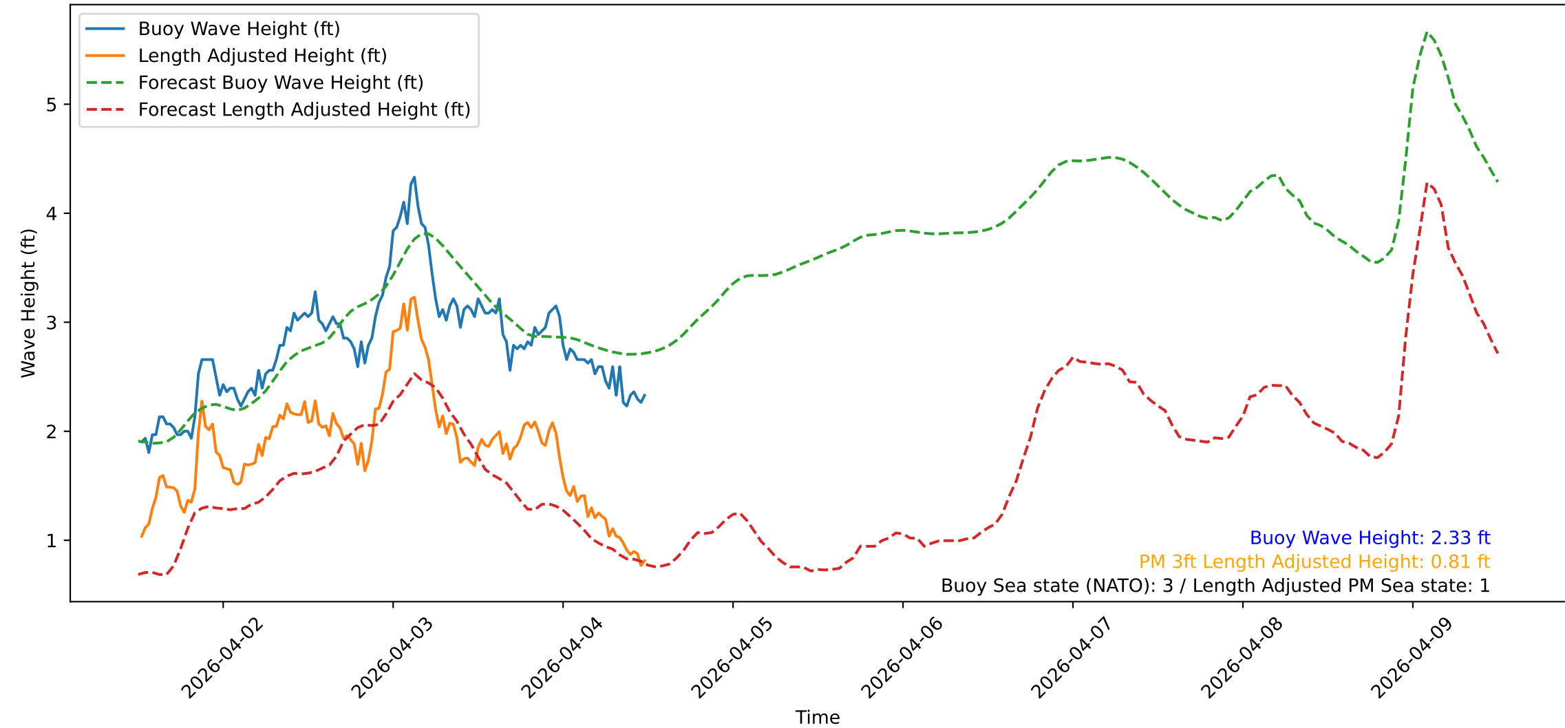
Wave Heights over Time for Green Beach at 2026-04-04 12:21:10
