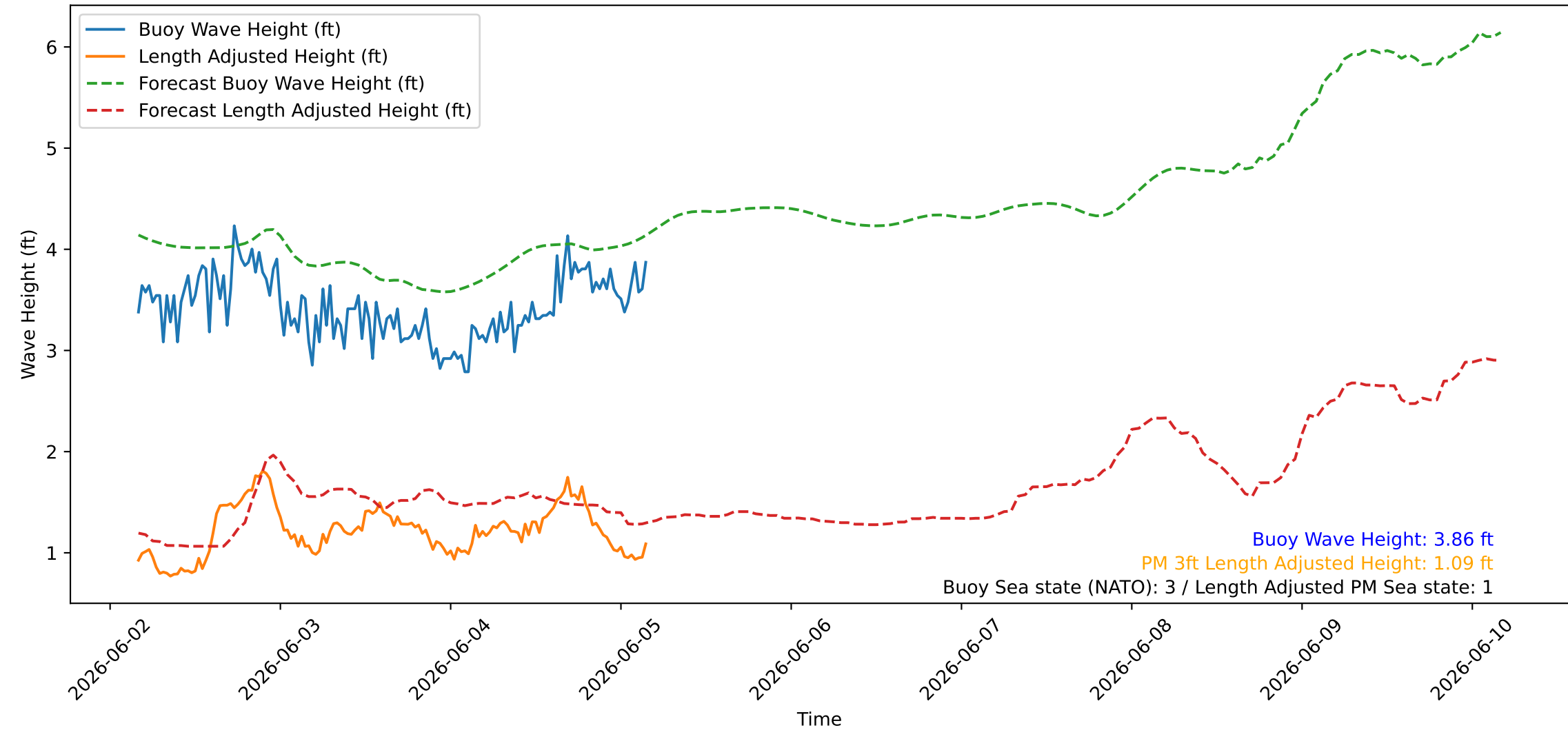
Wave Heights over Time for Green Beach at 2026-06-05 04:11:08
