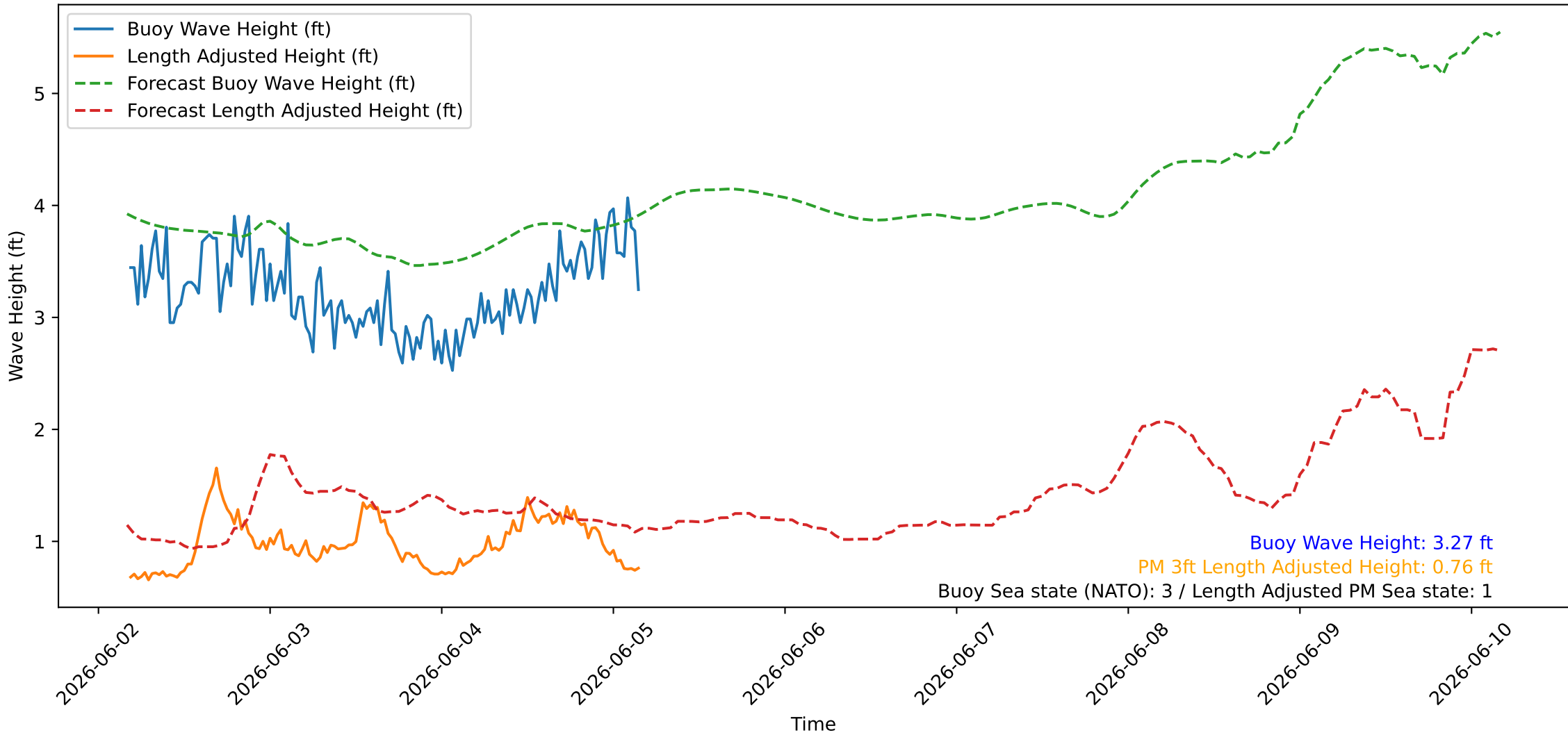
Wave Heights over Time for Red Beach at 2026-06-05 04:10:45
