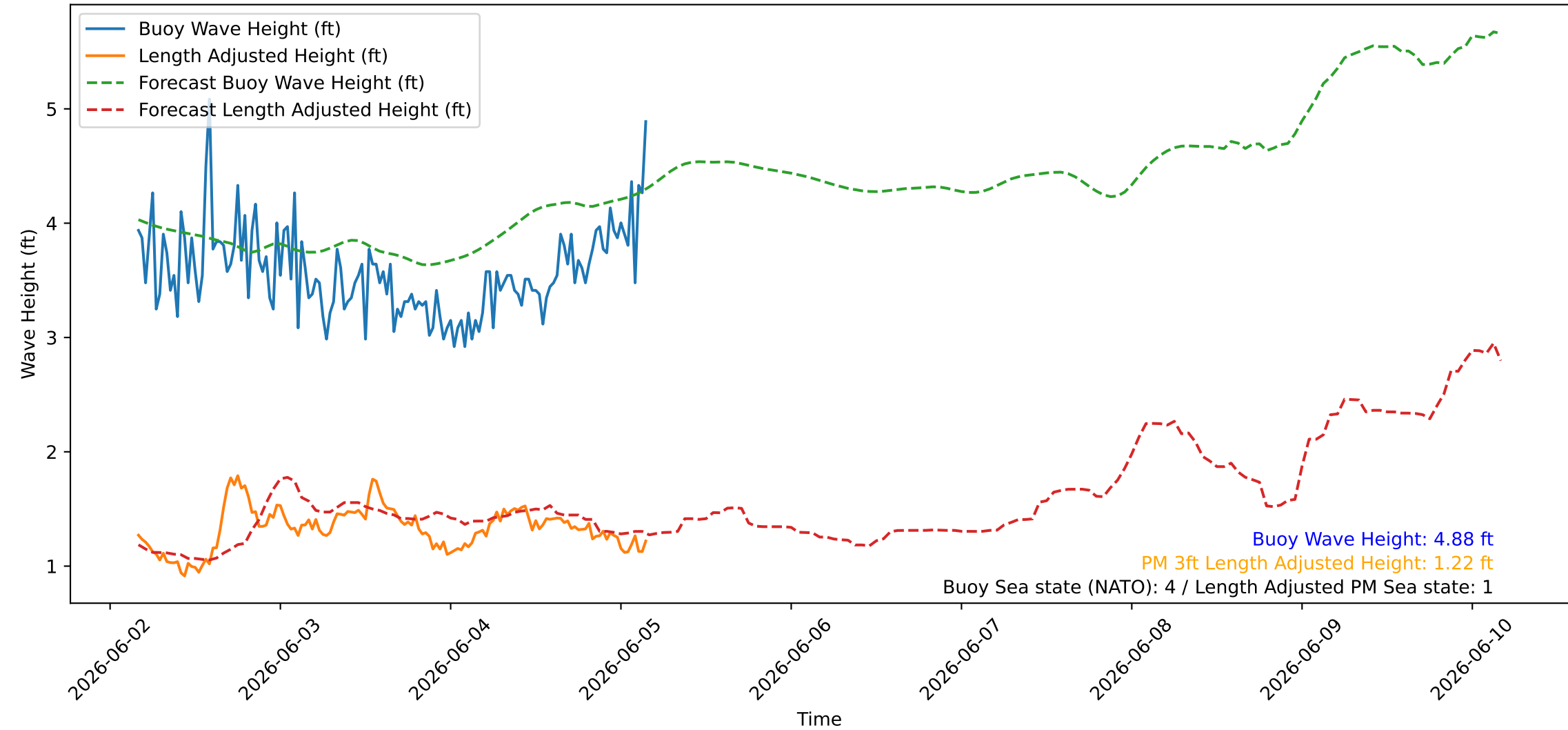
Wave Heights over Time for Oceanside Harbor at 2026-06-05 04:10:26
