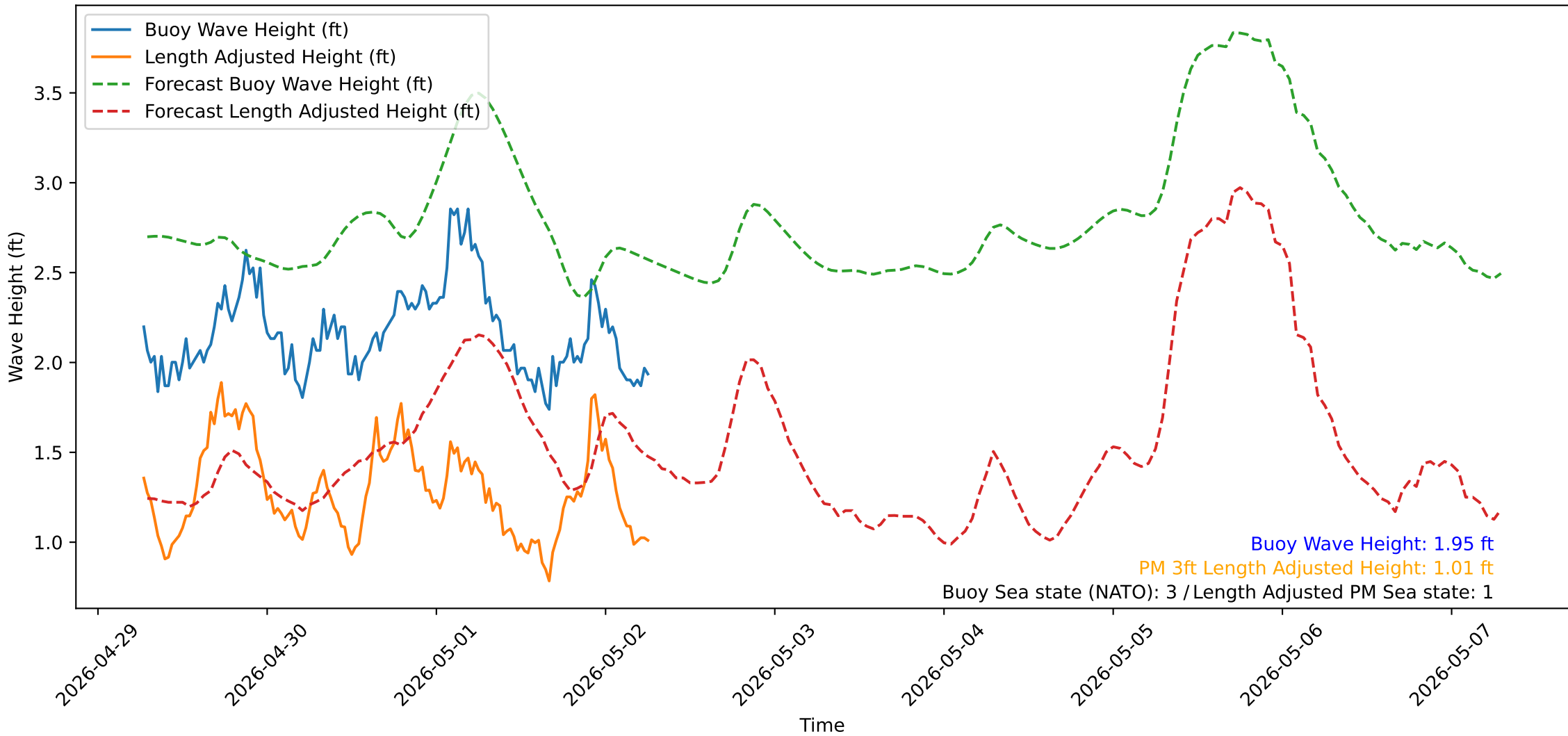
Wave Heights over Time for Green Beach at 2026-05-02 06:41:13
