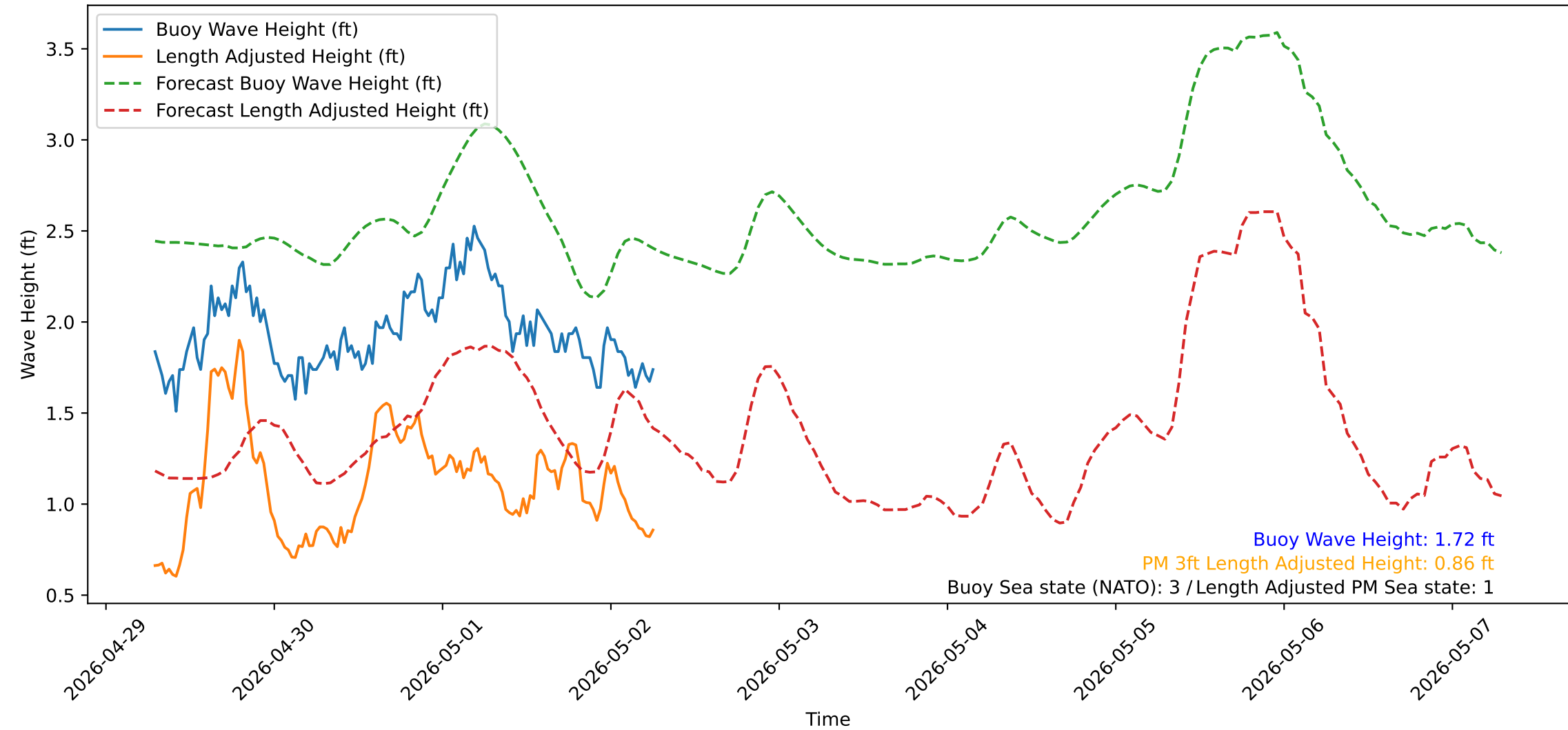
Wave Heights over Time for Red Beach at 2026-05-02 06:40:51
