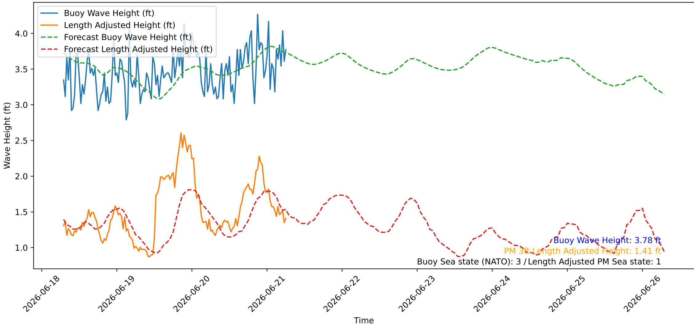
Wave Heights over Time for Oceanside Harbor at 2026-06-21 06:50:26
