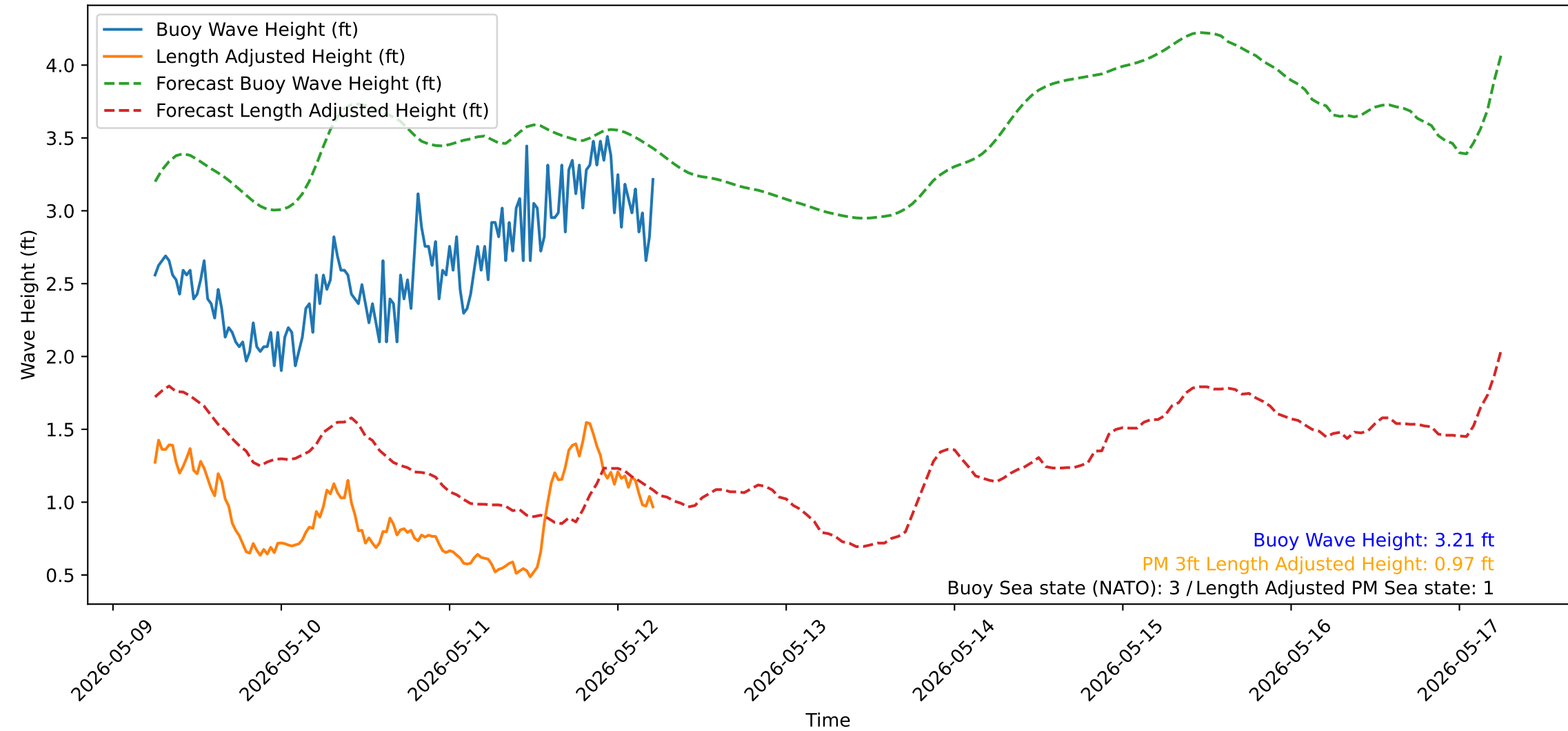
Wave Heights over Time for Green Beach at 2026-05-12 05:51:13
