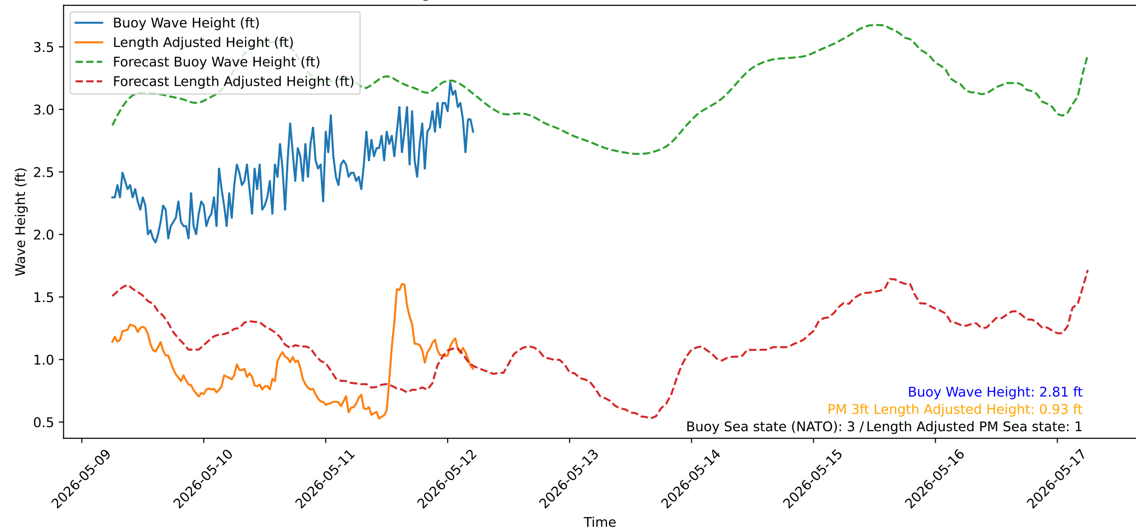
Wave Heights over Time for Red Beach at 2026-05-12 05:50:51
