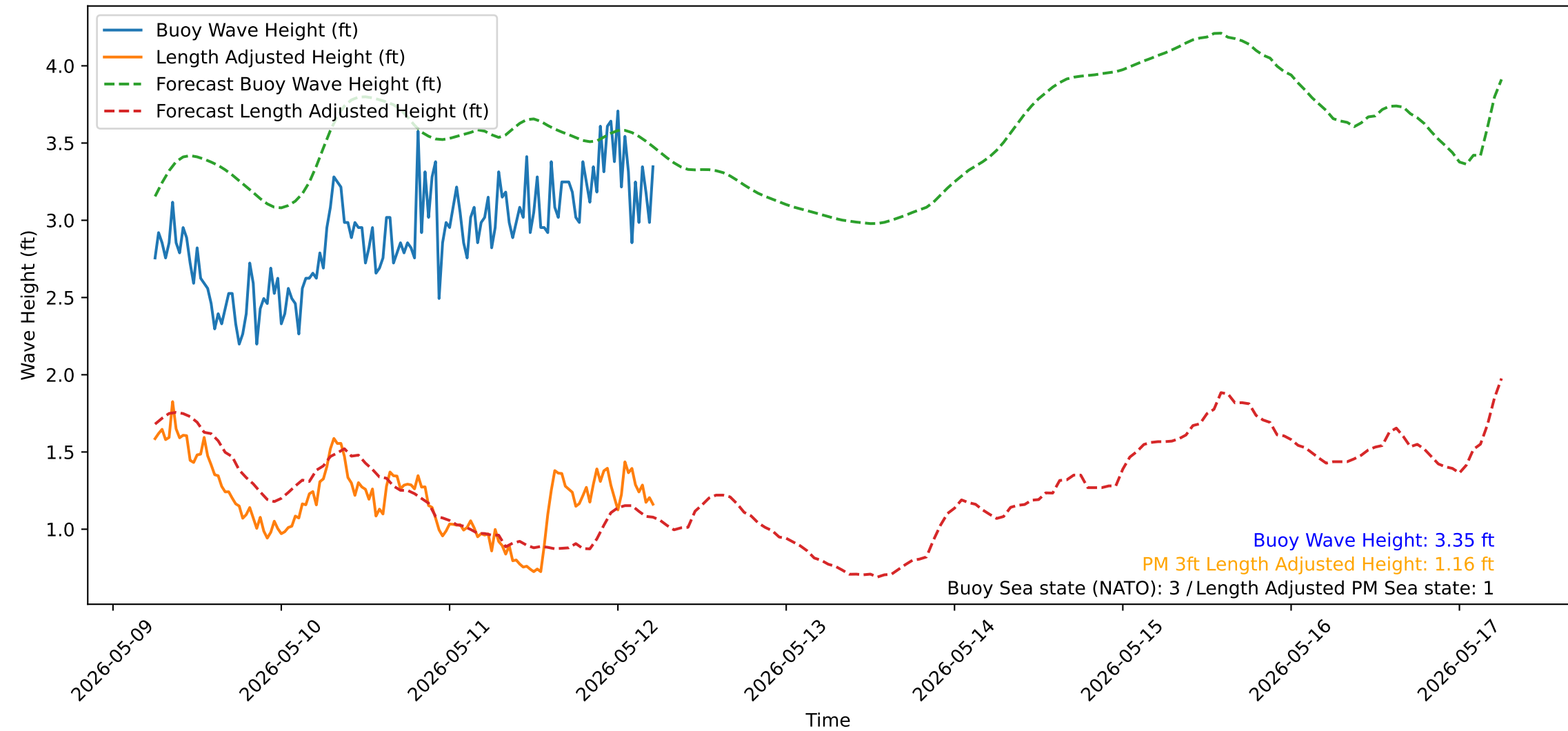
Wave Heights over Time for Oceanside Harbor at 2026-05-12 05:50:31
