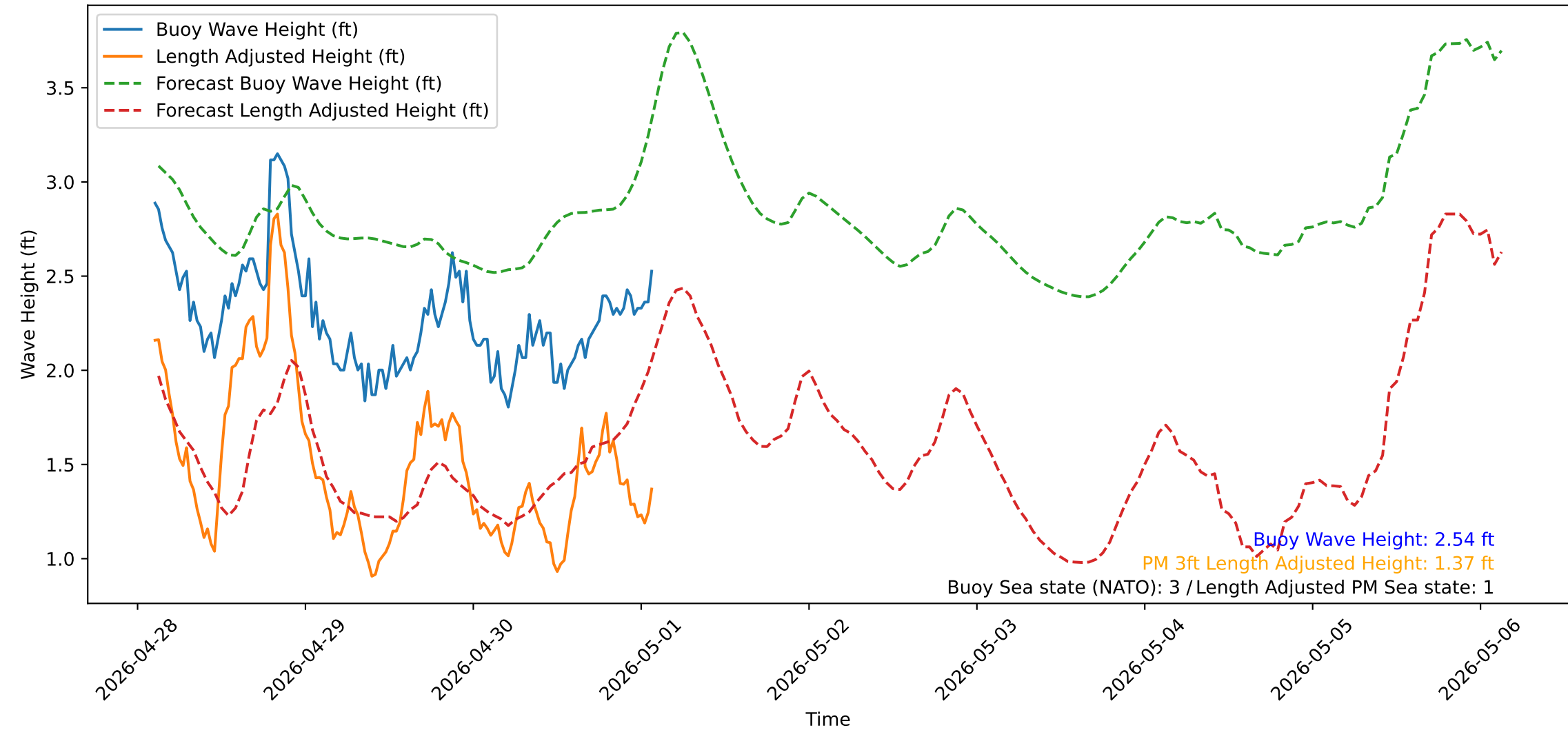
Wave Heights over Time for Green Beach at 2026-05-01 02:31:12
