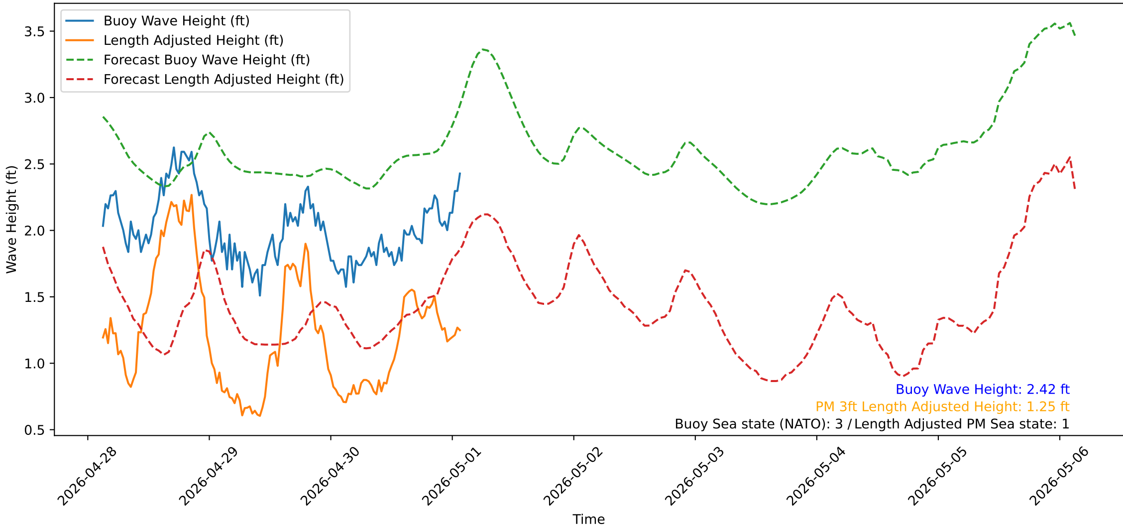
Wave Heights over Time for Red Beach at 2026-05-01 02:30:50
