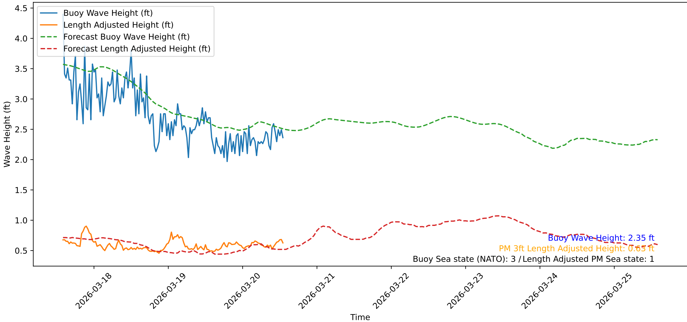
Wave Heights over Time for Oceanside Harbor at 2026-03-20 13:50:33
