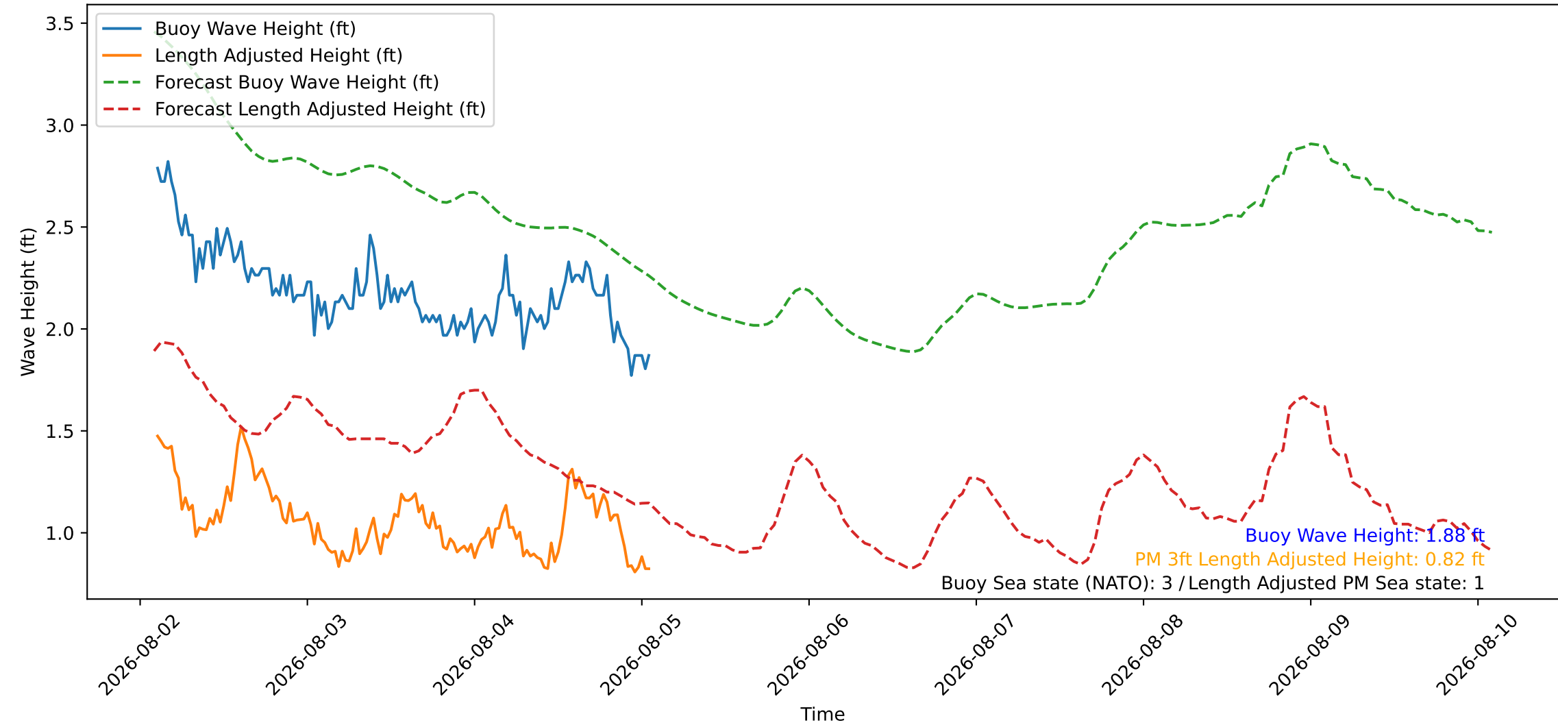
Wave Heights over Time for Red Beach at 2026-08-05 02:10:46
