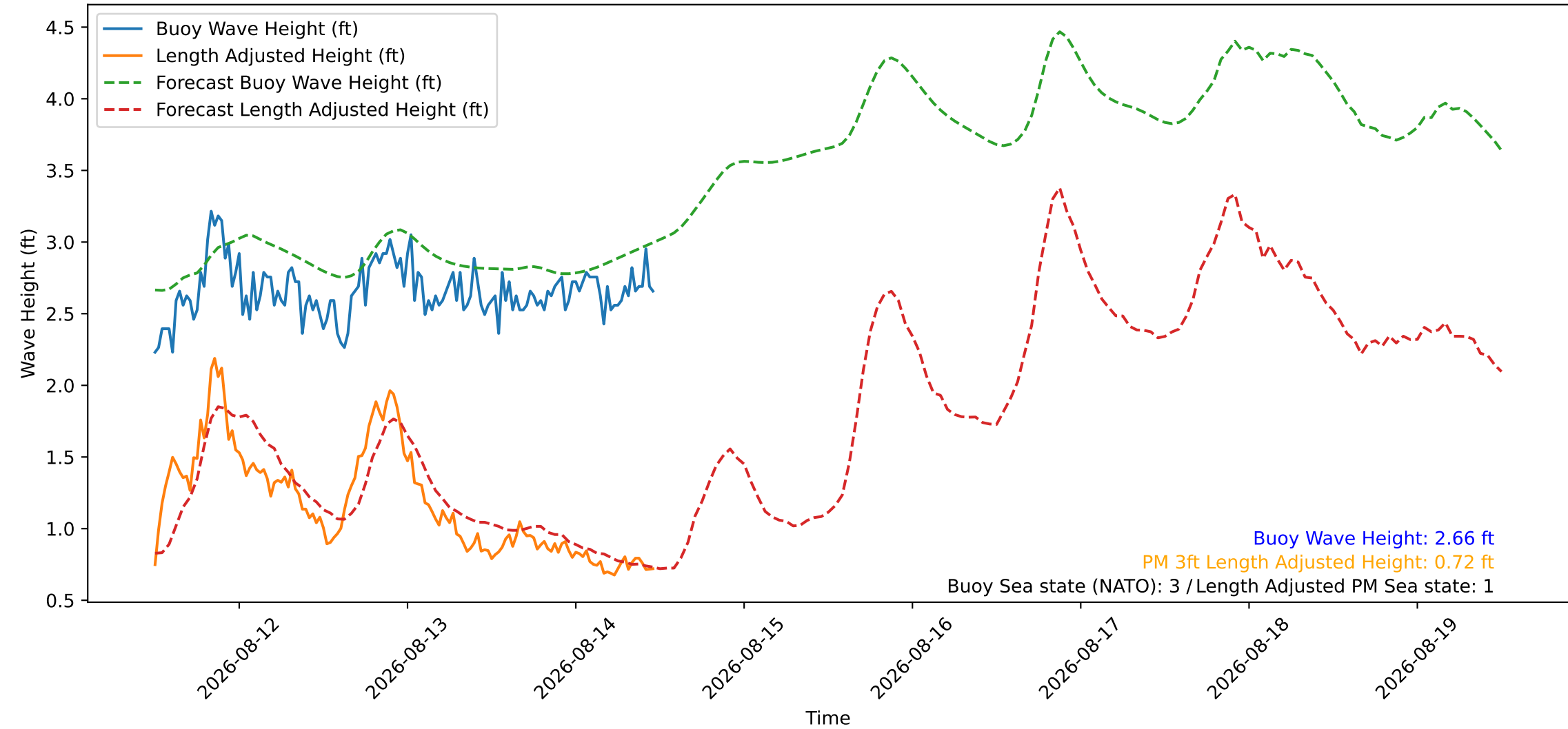
Wave Heights over Time for Green Beach at 2026-08-14 12:01:07
