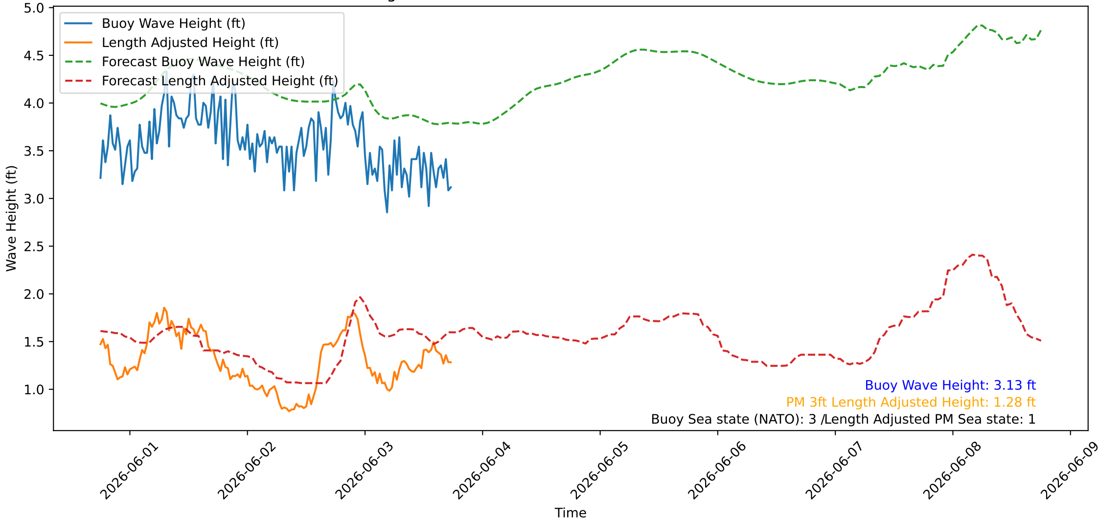
Wave Heights over Time for Green Beach at 2026-06-03 18:11:08
