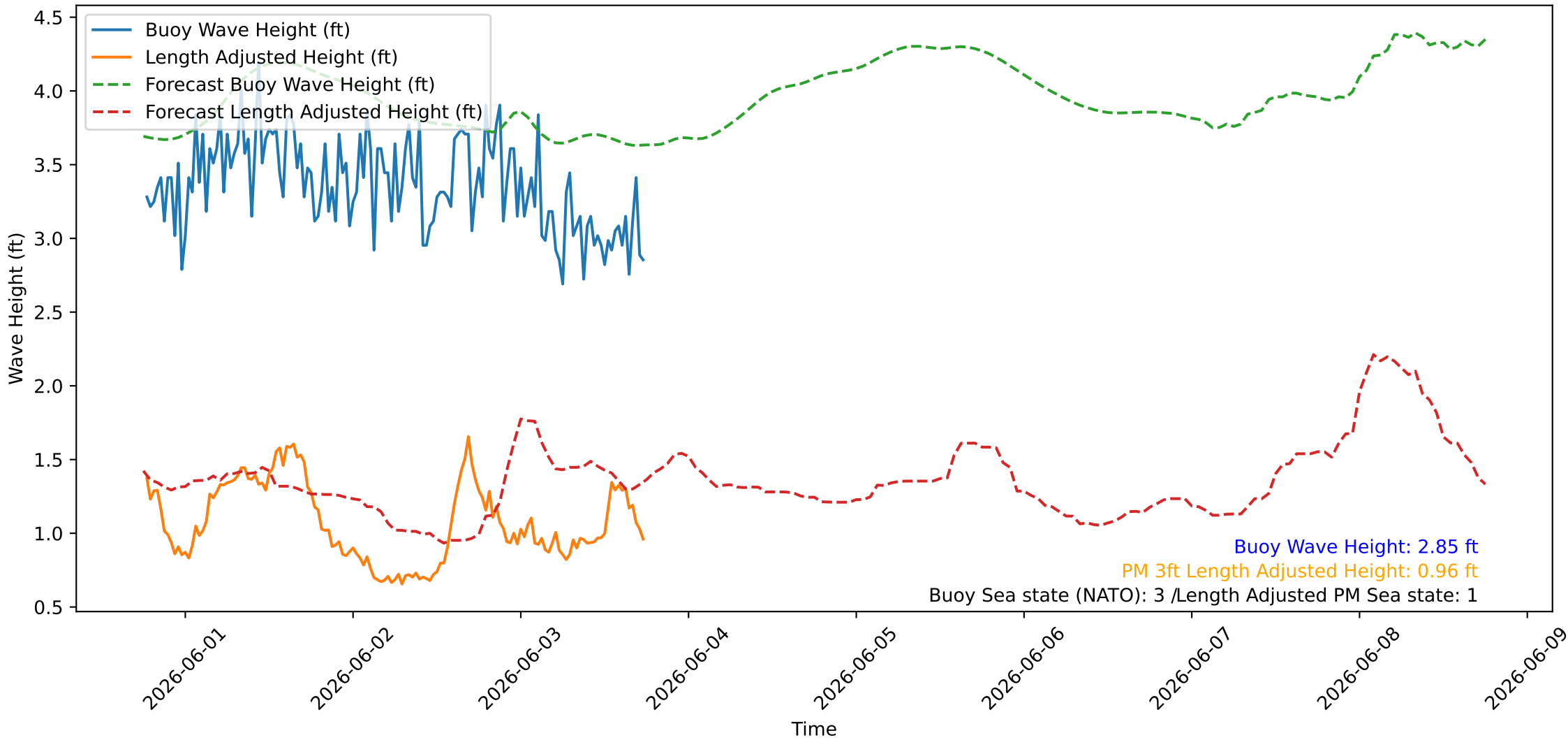
Wave Heights over Time for Red Beach at 2026-06-03 18:10:46
