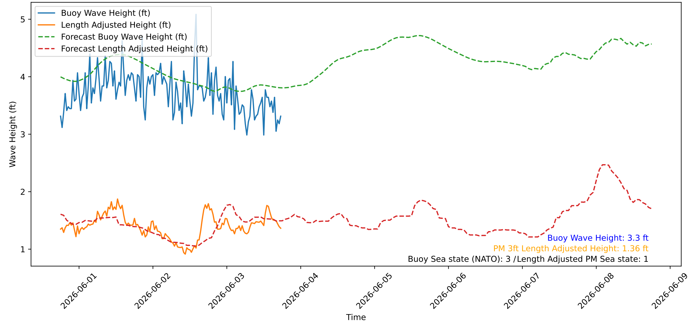
Wave Heights over Time for Oceanside Harbor at 2026-06-03 18:10:26
