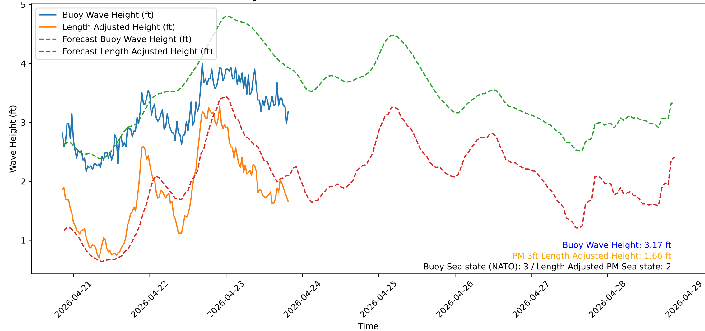
Wave Heights over Time for Green Beach at 2026-04-23 20:31:13
