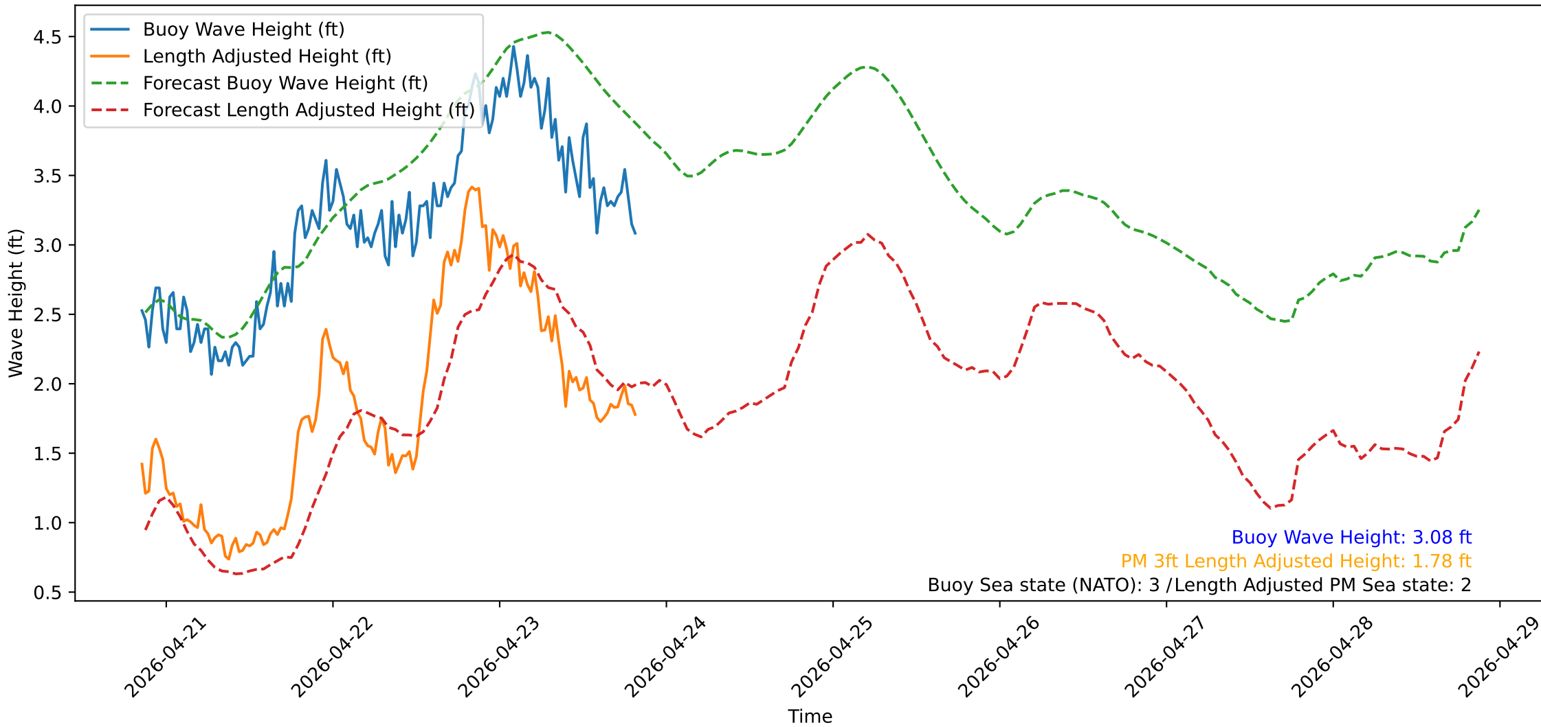
Wave Heights over Time for Oceanside Harbor at 2026-04-23 20:30:31
