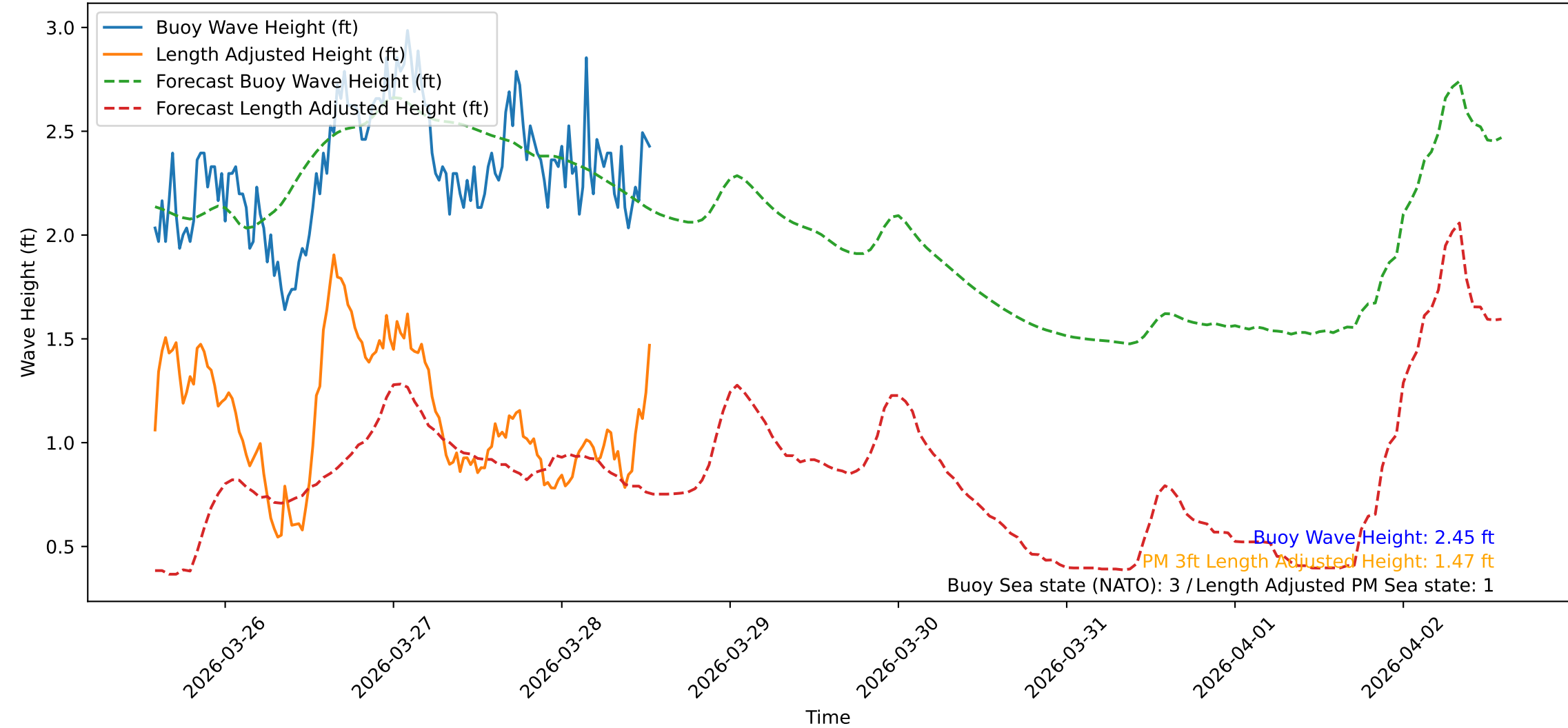
Wave Heights over Time for Red Beach at 2026-03-28 13:30:47
