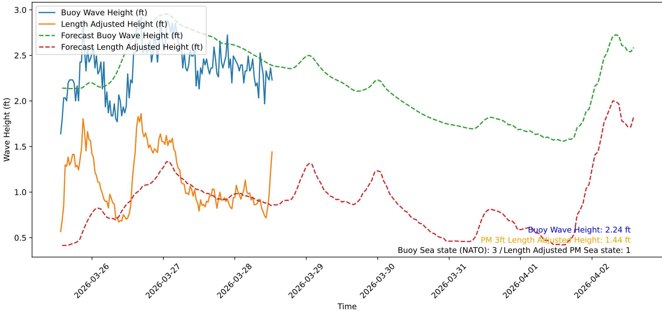
Wave Heights over Time for Oceanside Harbor at 2026-03-28 13:30:31
