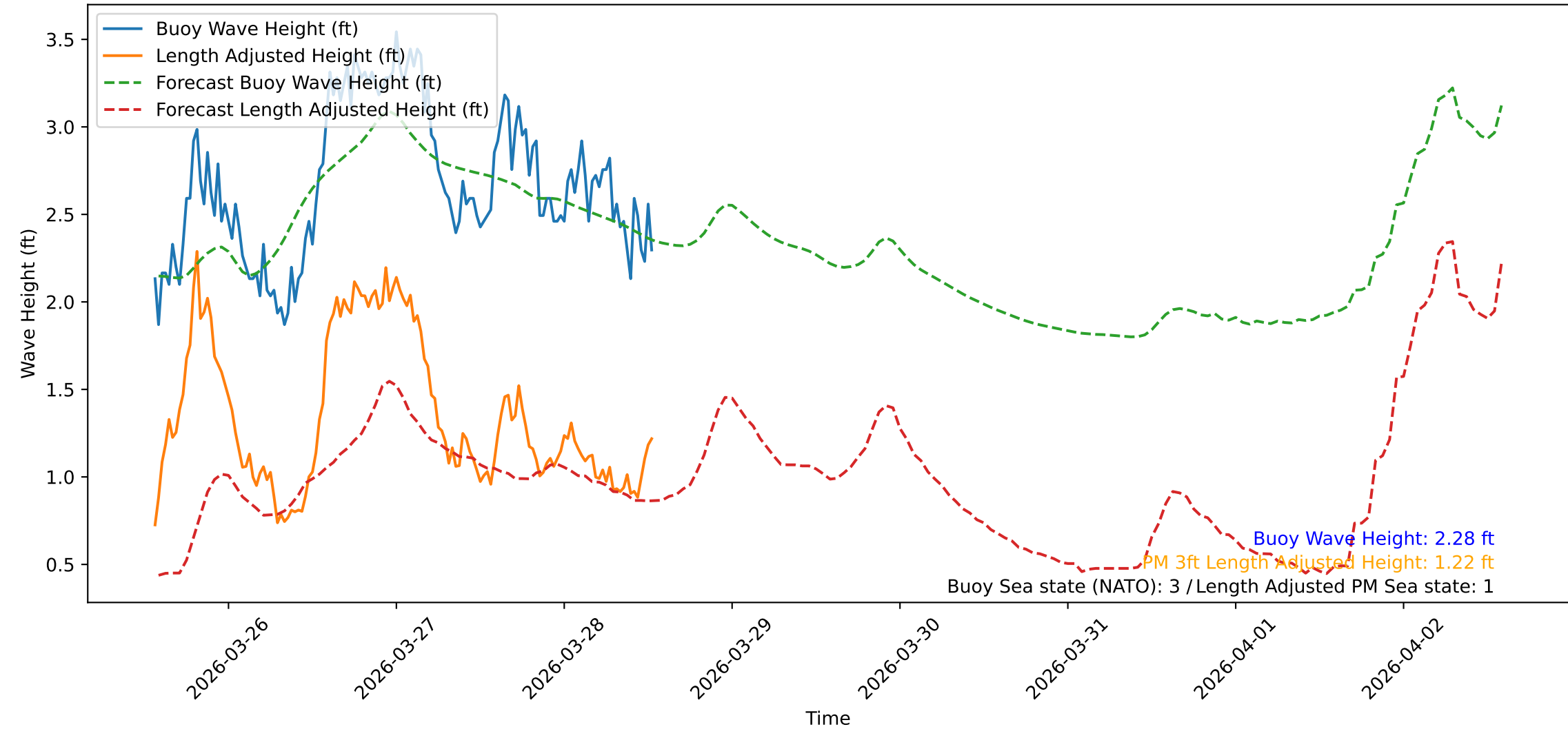
Wave Heights over Time for Green Beach at 2026-03-28 13:31:09
