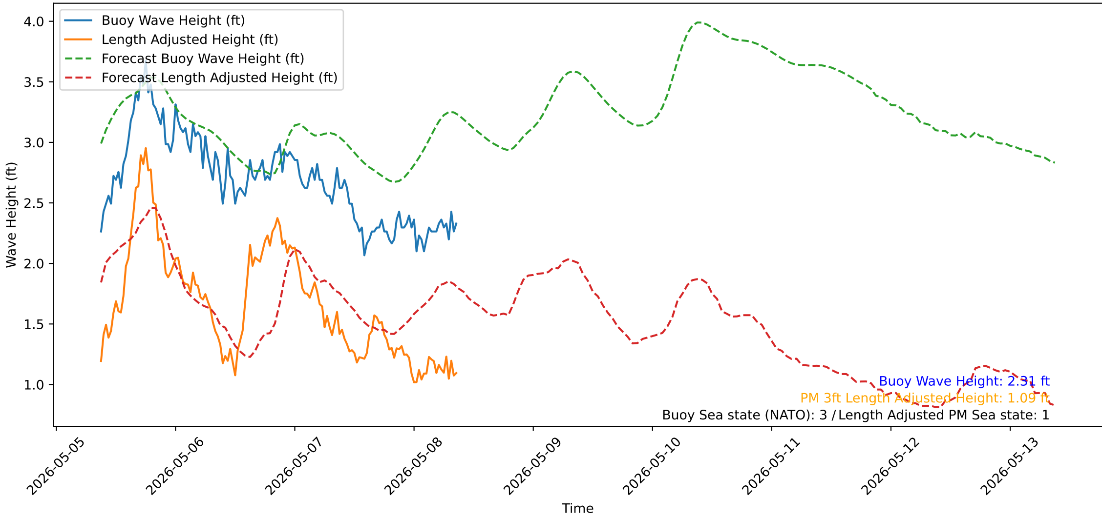
Wave Heights over Time for Green Beach at 2026-05-08 09:11:13
