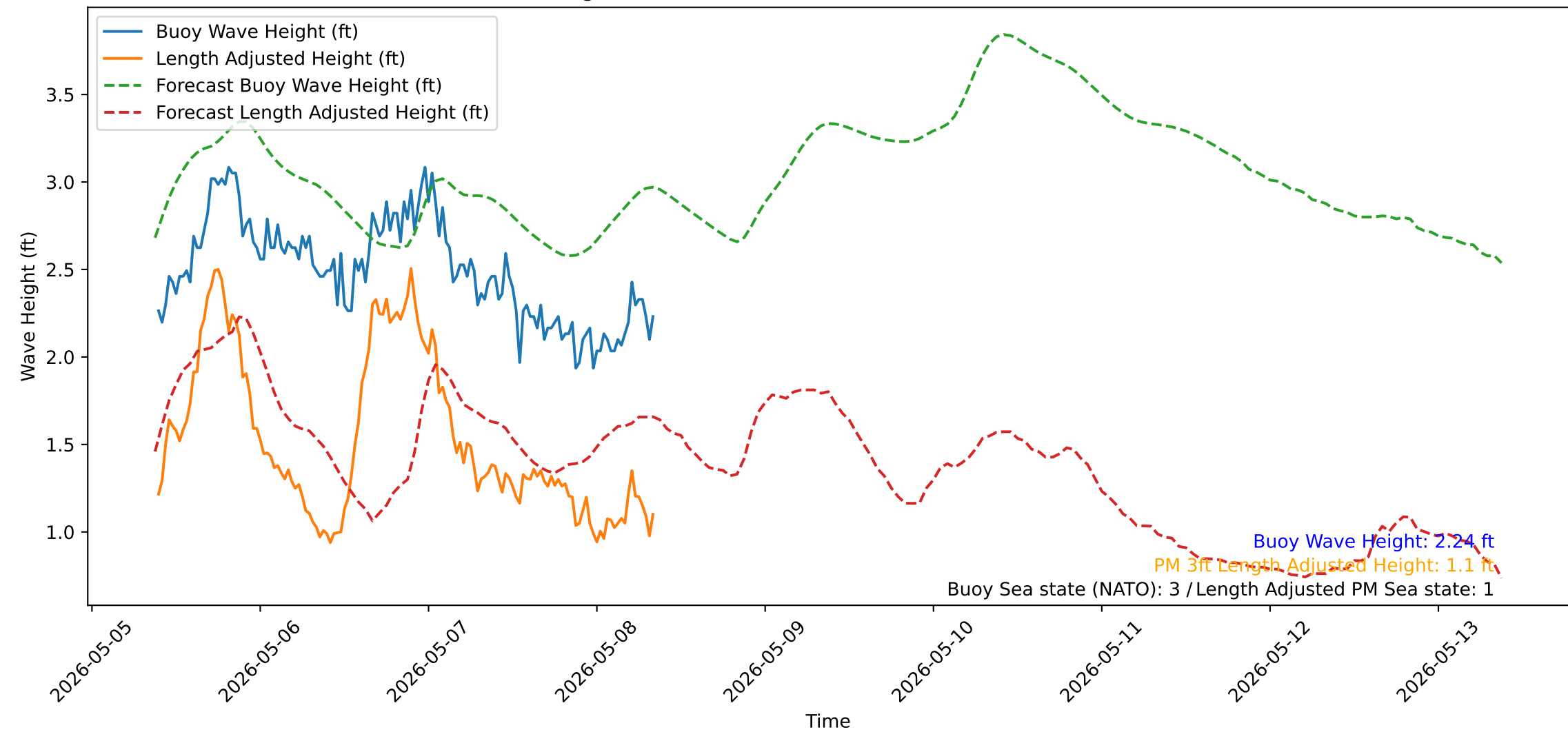
Wave Heights over Time for Red Beach at 2026-05-08 09:10:51
