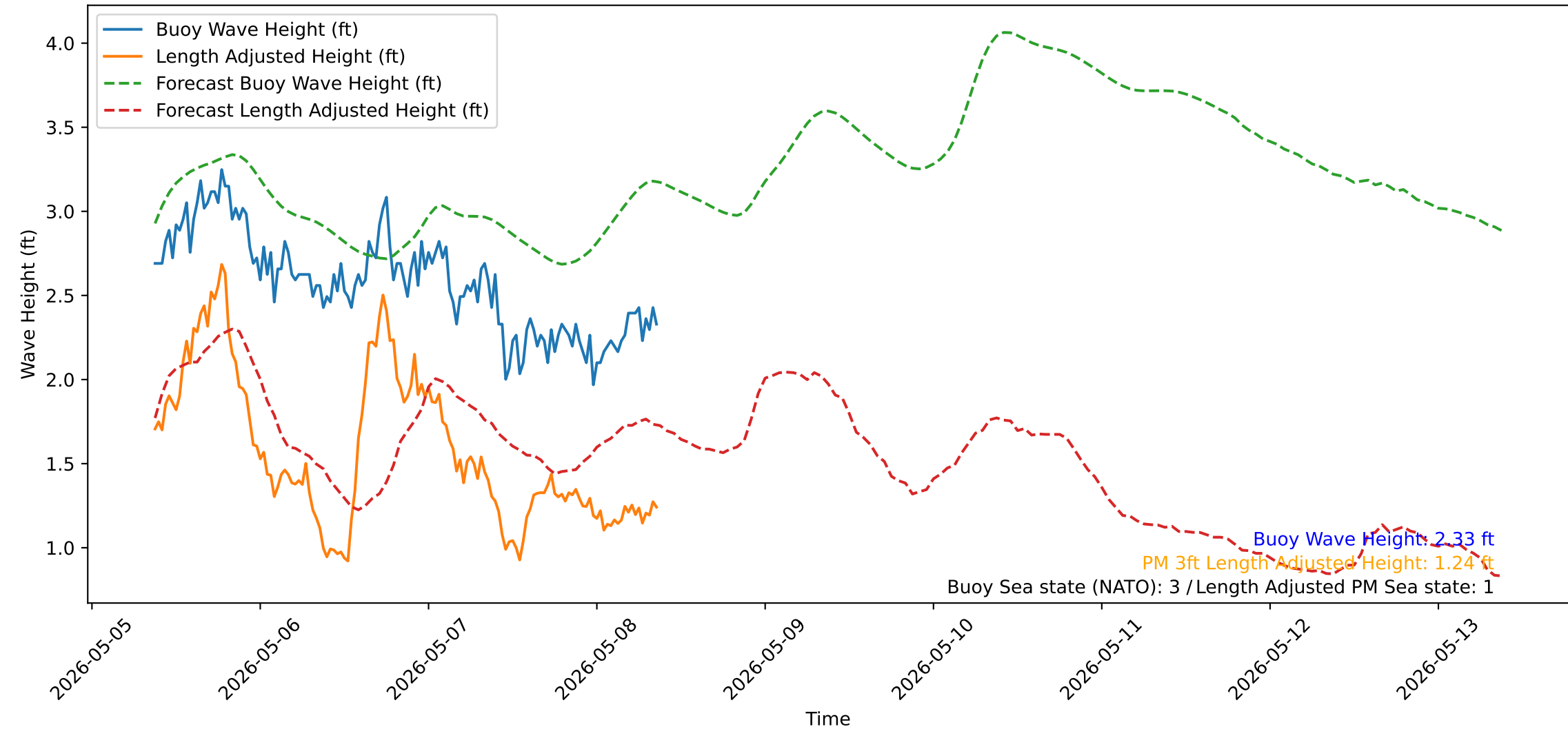
Wave Heights over Time for Oceanside Harbor at 2026-05-08 09:10:31
