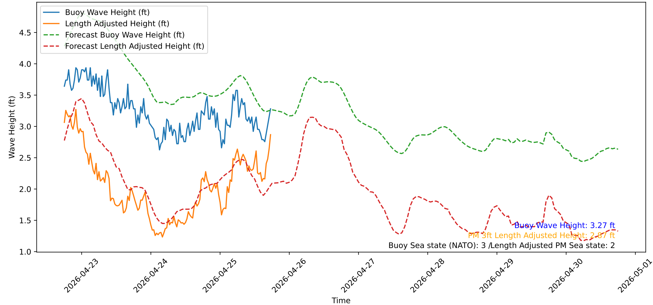
Wave Heights over Time for Green Beach at 2026-04-25 18:11:12
