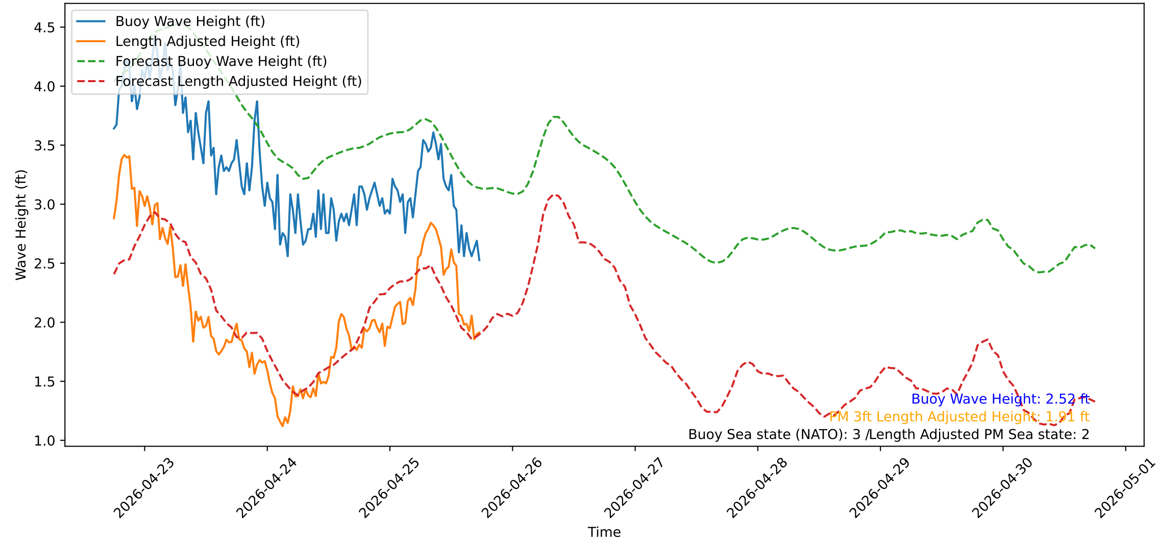
Wave Heights over Time for Oceanside Harbor at 2026-04-25 18:10:31
