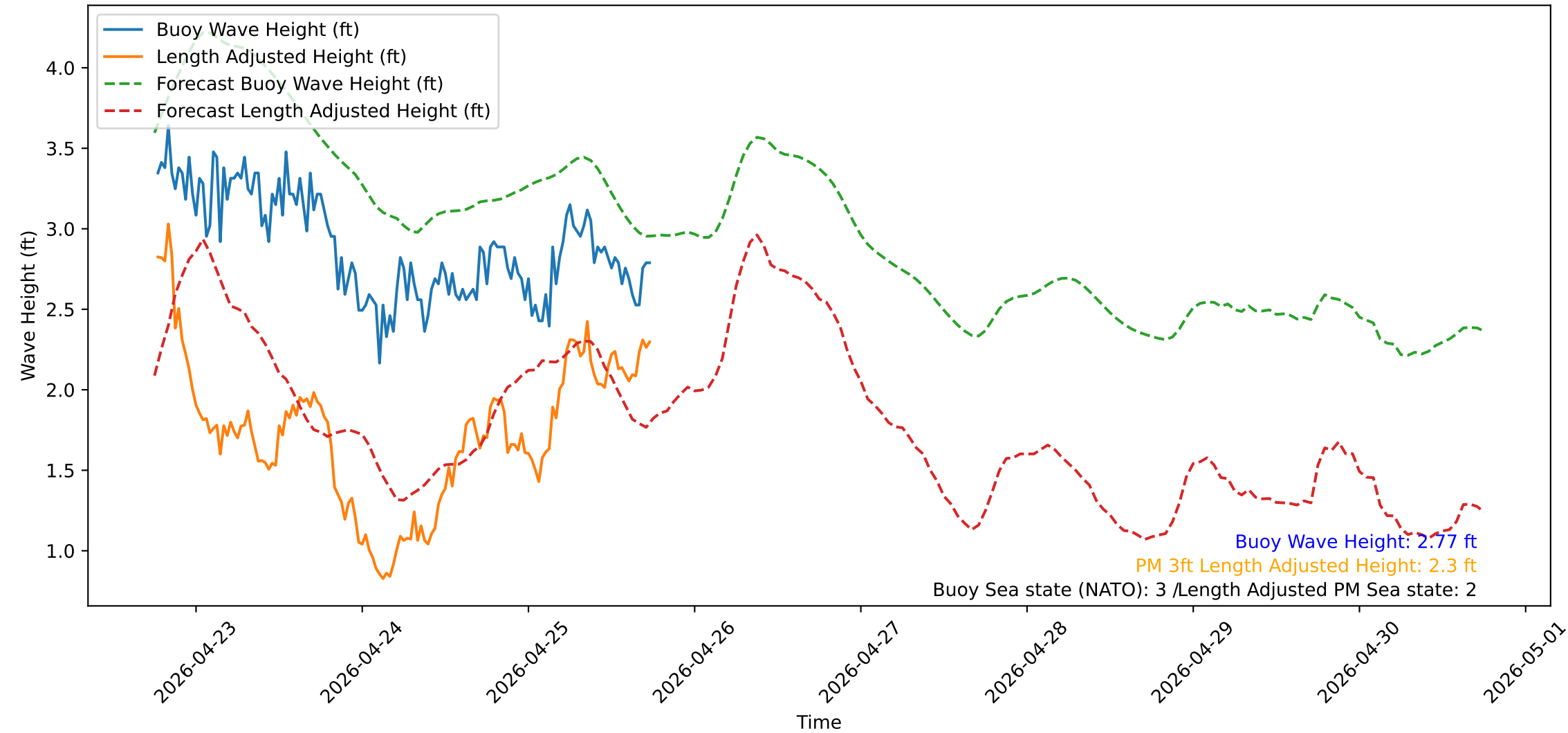
Wave Heights over Time for Red Beach at 2026-04-25 18:10:50
