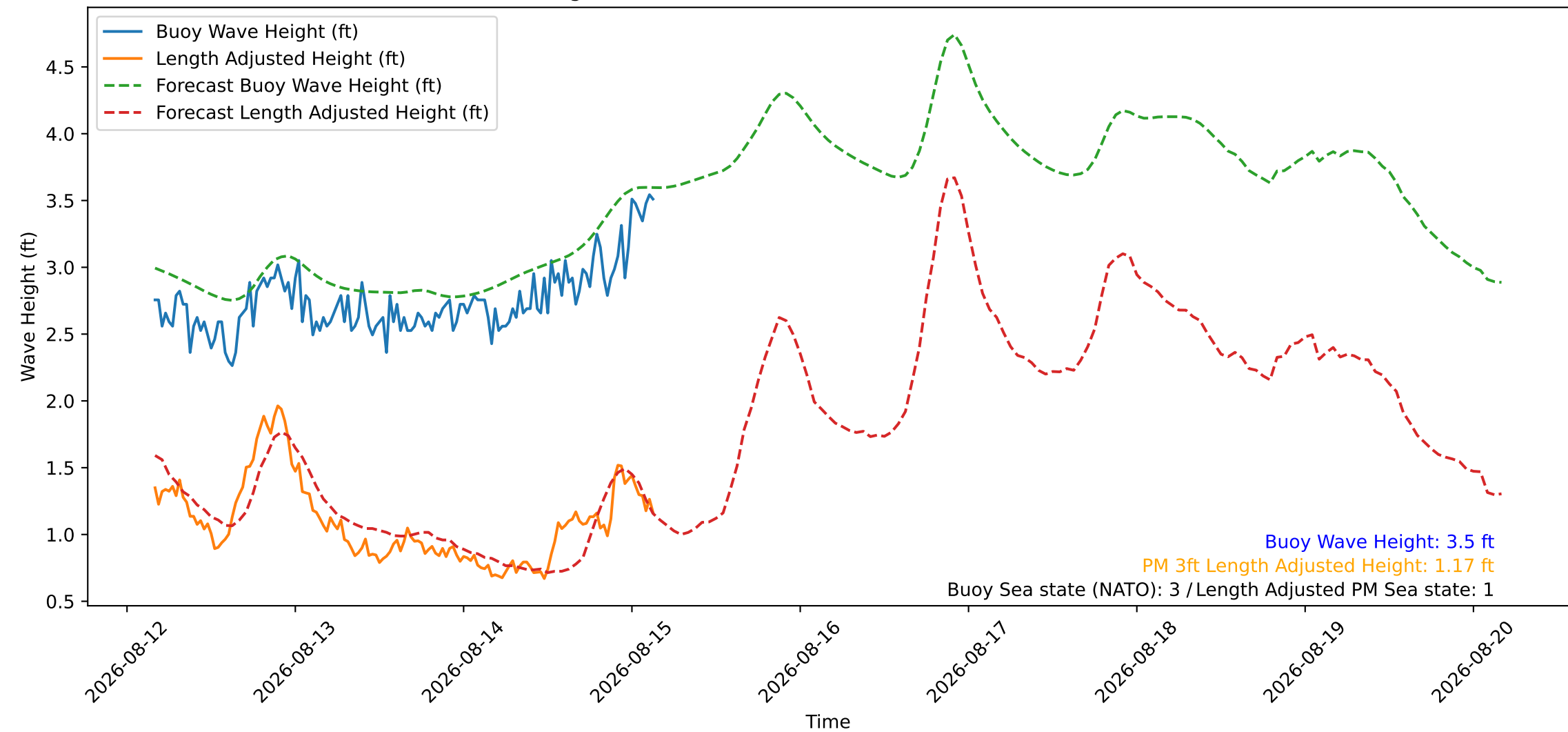
Wave Heights over Time for Green Beach at 2026-08-15 04:01:07
