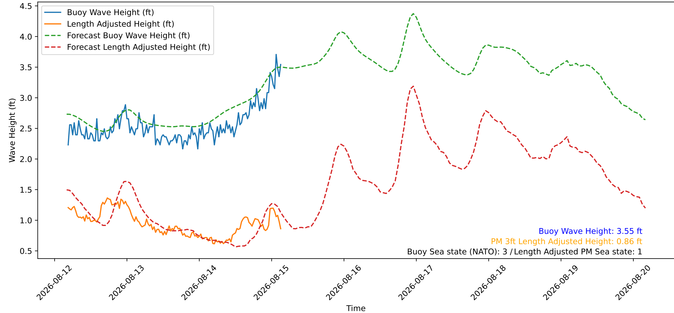
Wave Heights over Time for Red Beach at 2026-08-15 04:00:45
