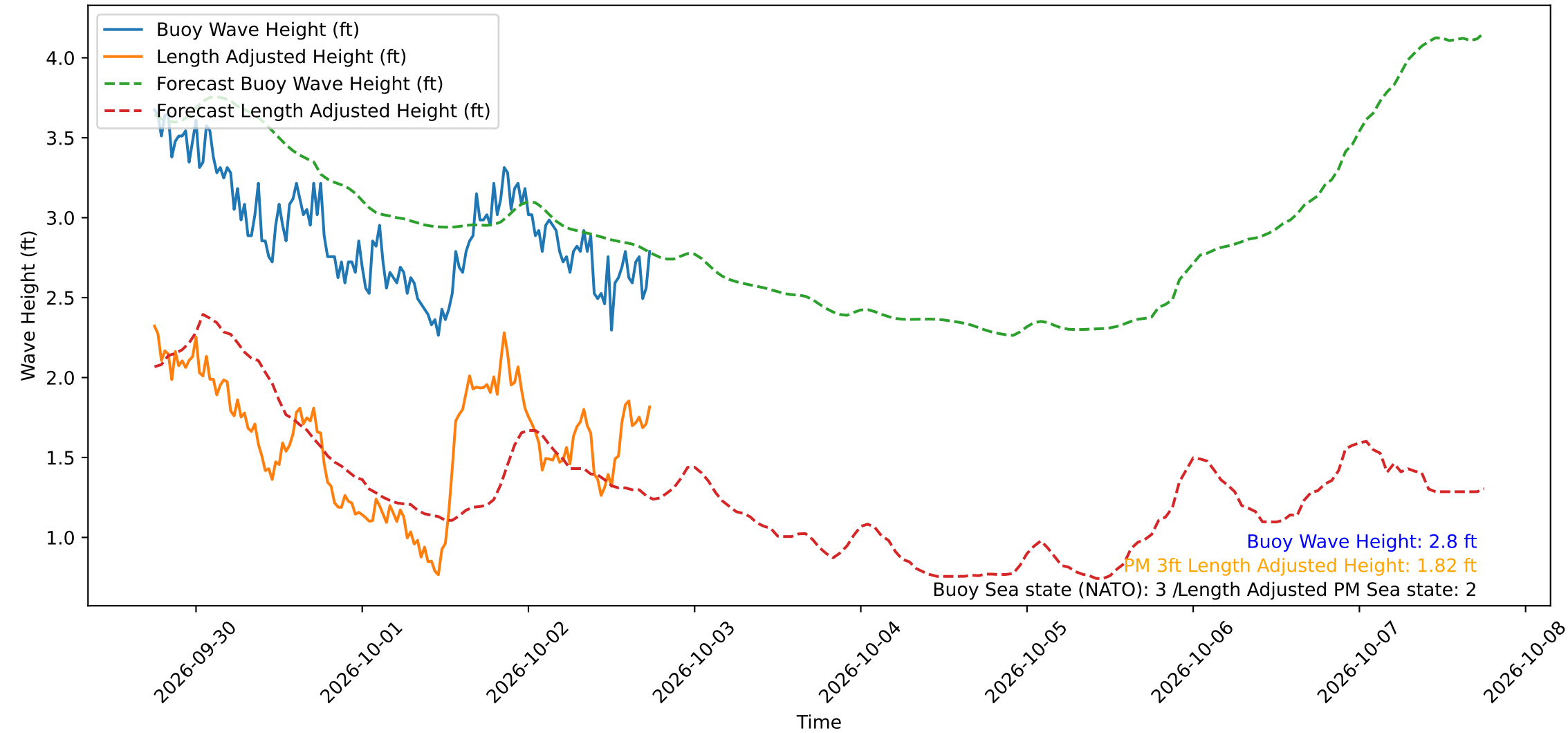
Wave Heights over Time for Oceanside Harbor at 2026-10-02 18:10:29
