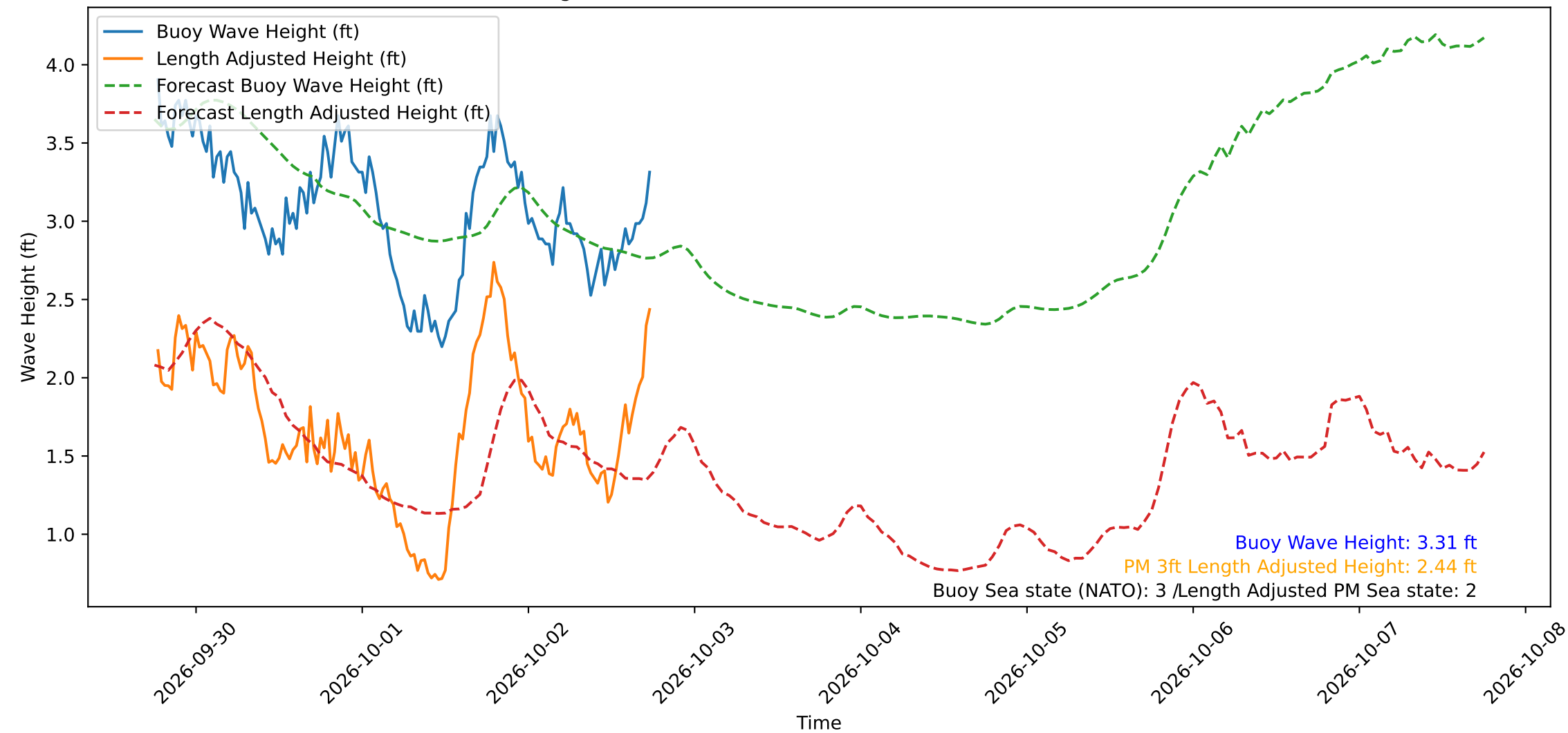
Wave Heights over Time for Green Beach at 2026-10-02 18:11:11
