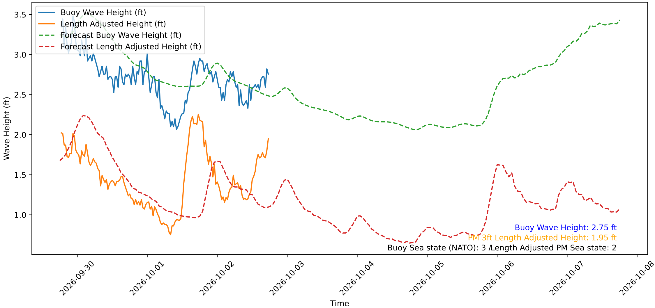
Wave Heights over Time for Red Beach at 2026-10-02 18:10:49
