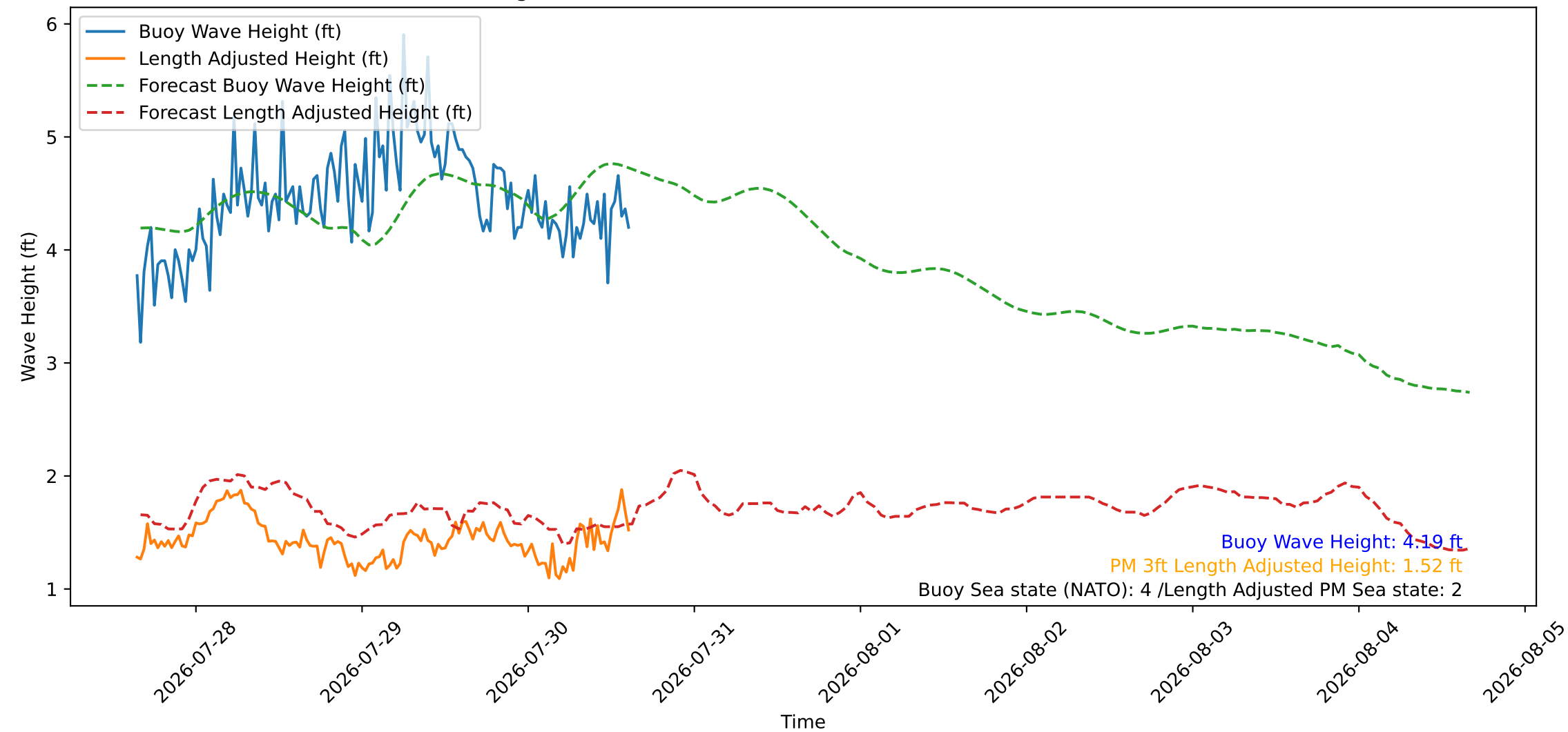
Wave Heights over Time for Oceanside Harbor at 2026-07-30 15:30:26
