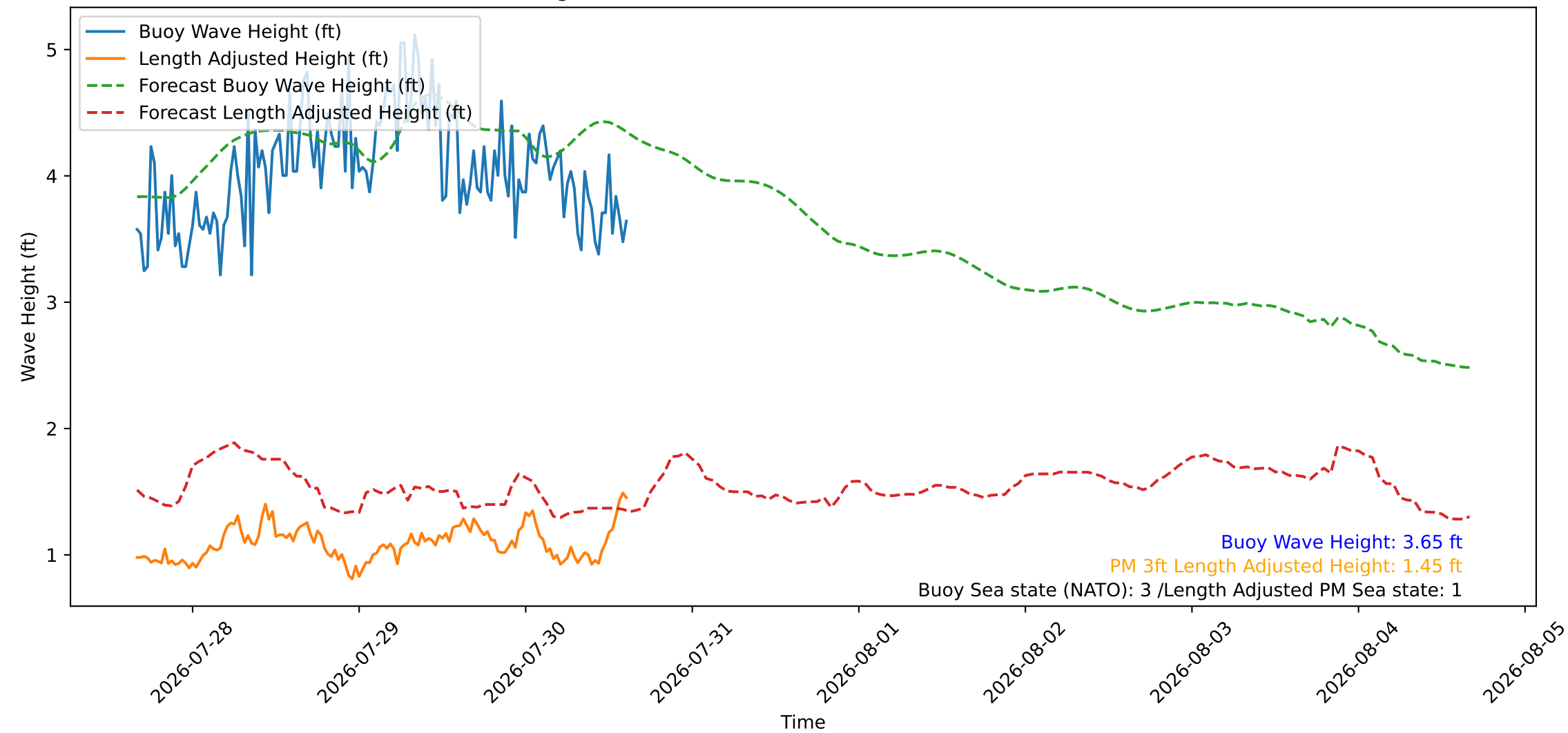
Wave Heights over Time for Red Beach at 2026-07-30 15:30:46
