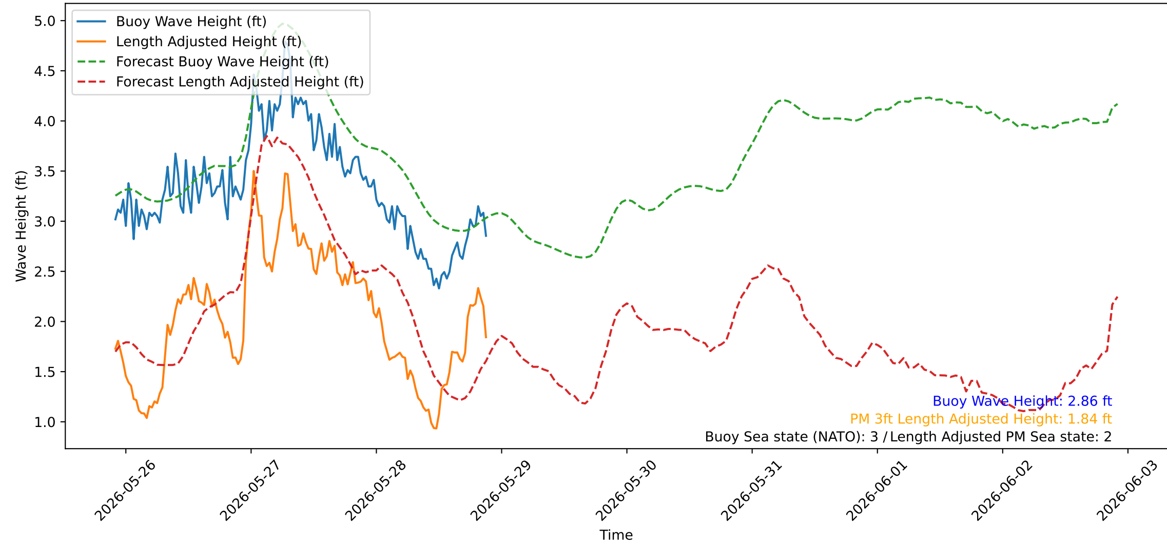
Wave Heights over Time for Red Beach at 2026-05-28 21:50:39
