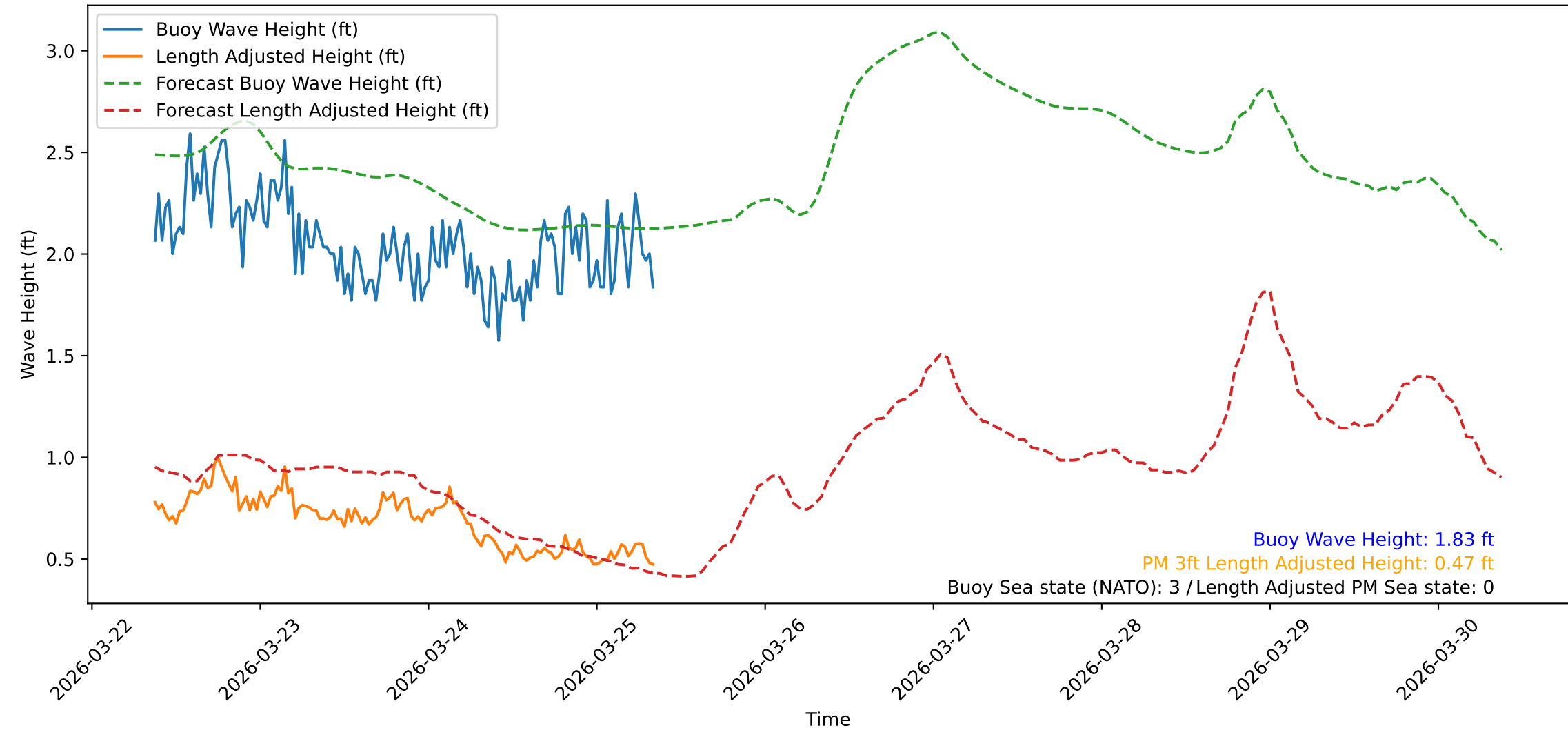
Wave Heights over Time for Oceanside Harbor at 2026-03-25 08:50:31
