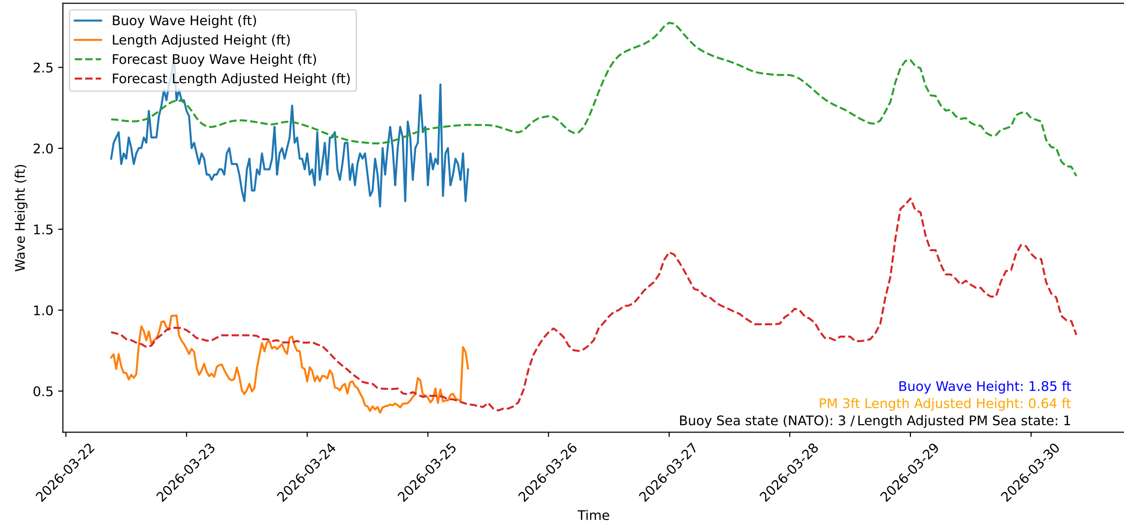
Wave Heights over Time for Red Beach at 2026-03-25 08:50:48
