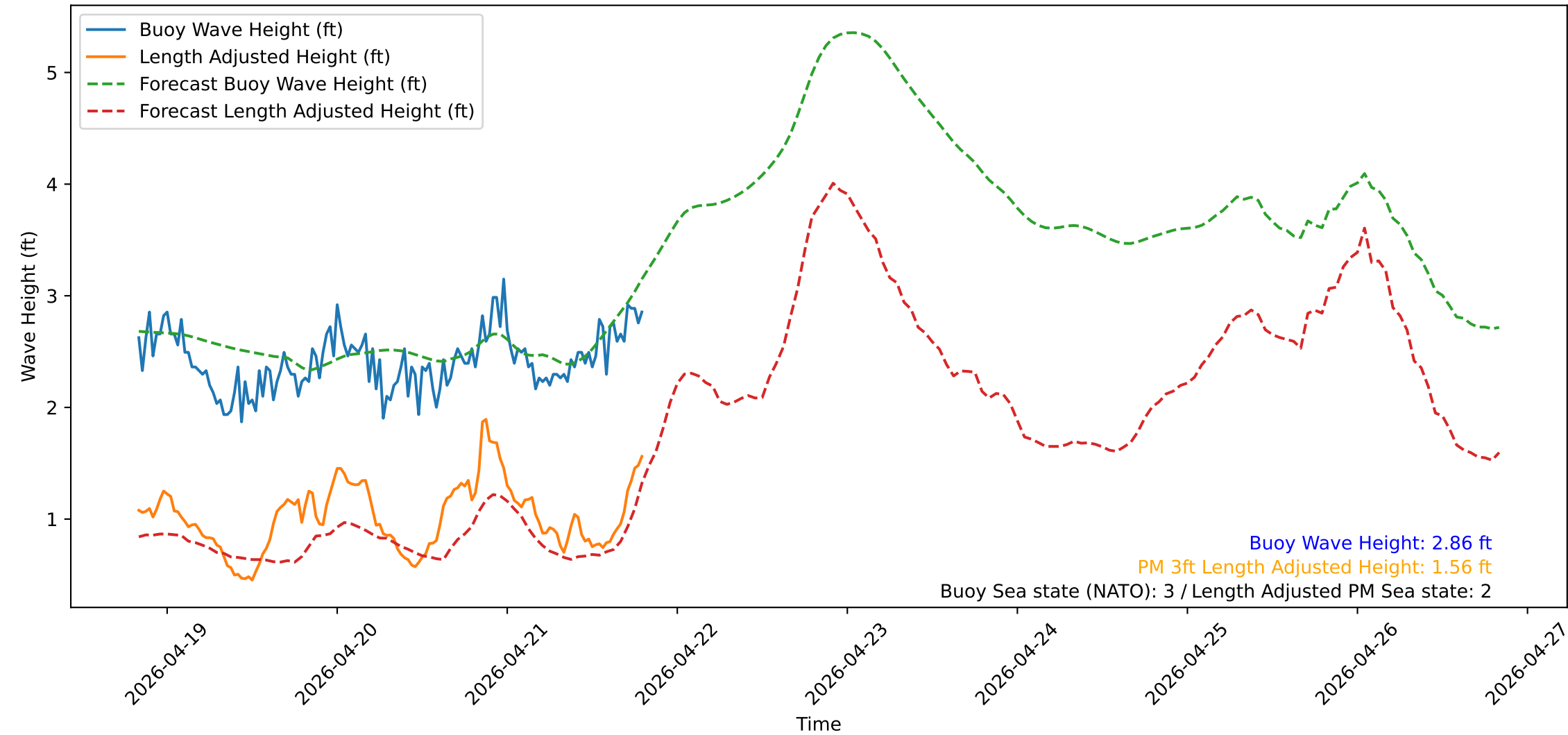
Wave Heights over Time for Green Beach at 2026-04-21 20:01:12
