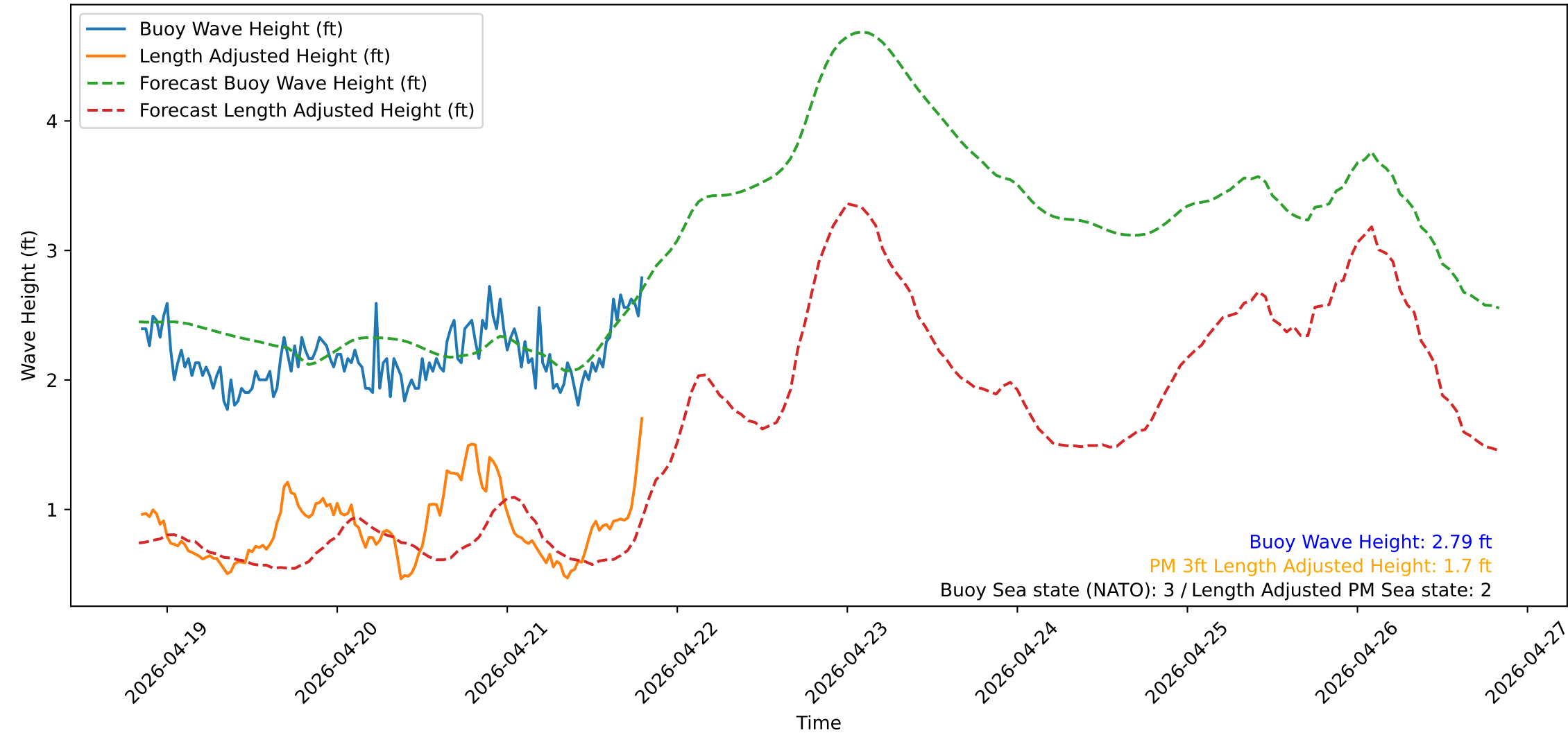
Wave Heights over Time for Red Beach at 2026-04-21 20:00:50
