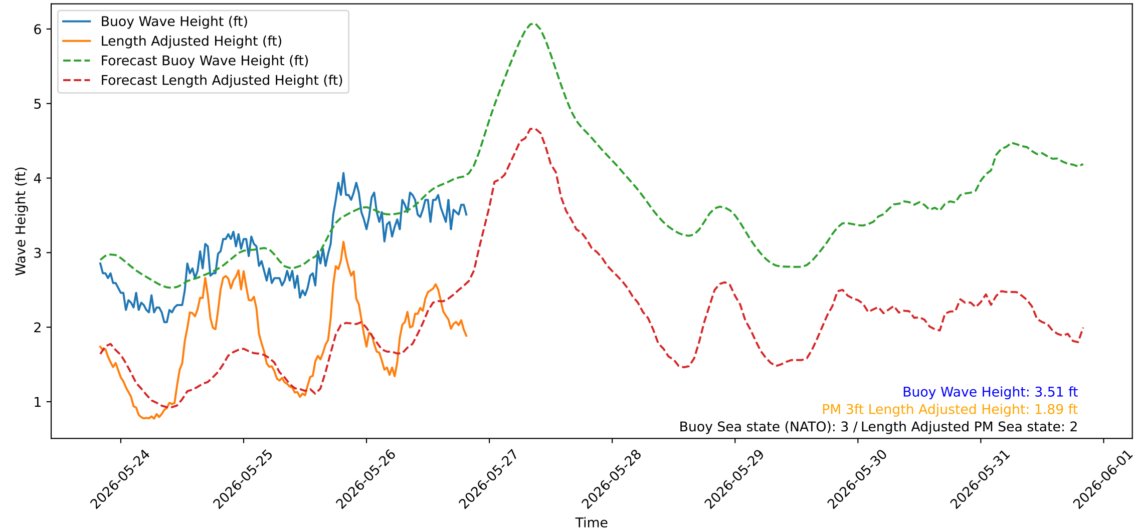
Wave Heights over Time for Green Beach at 2026-05-26 20:11:09
