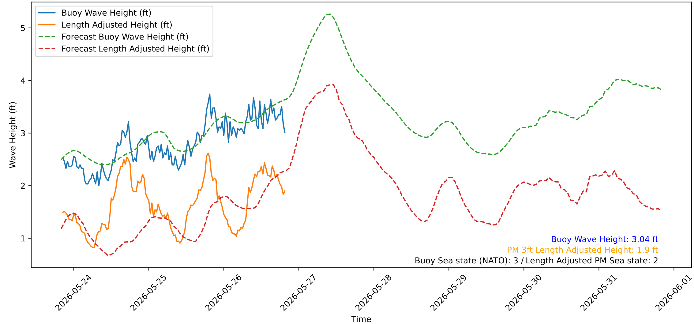
Wave Heights over Time for Red Beach at 2026-05-26 20:10:46
