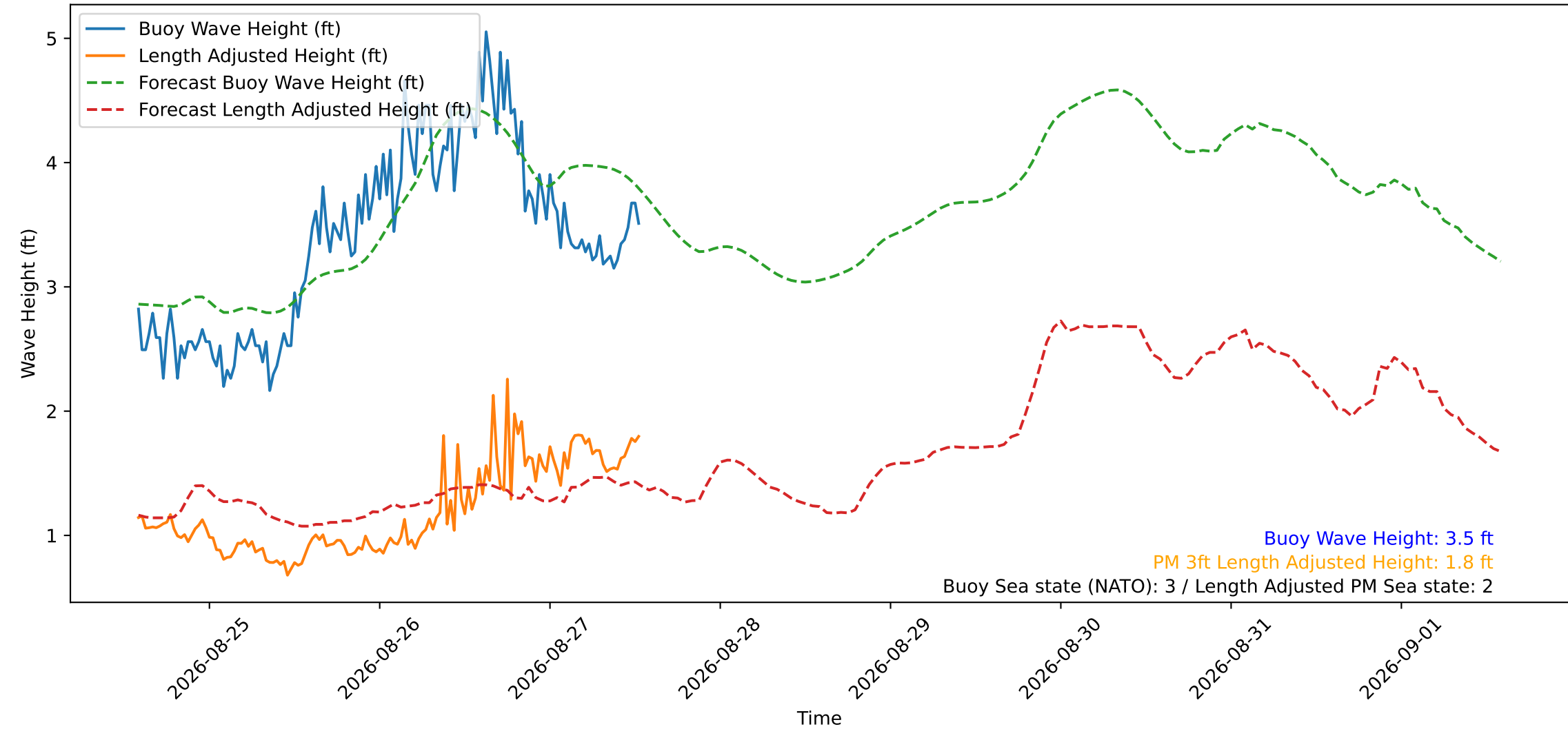
Wave Heights over Time for Red Beach at 2026-08-27 13:30:49
