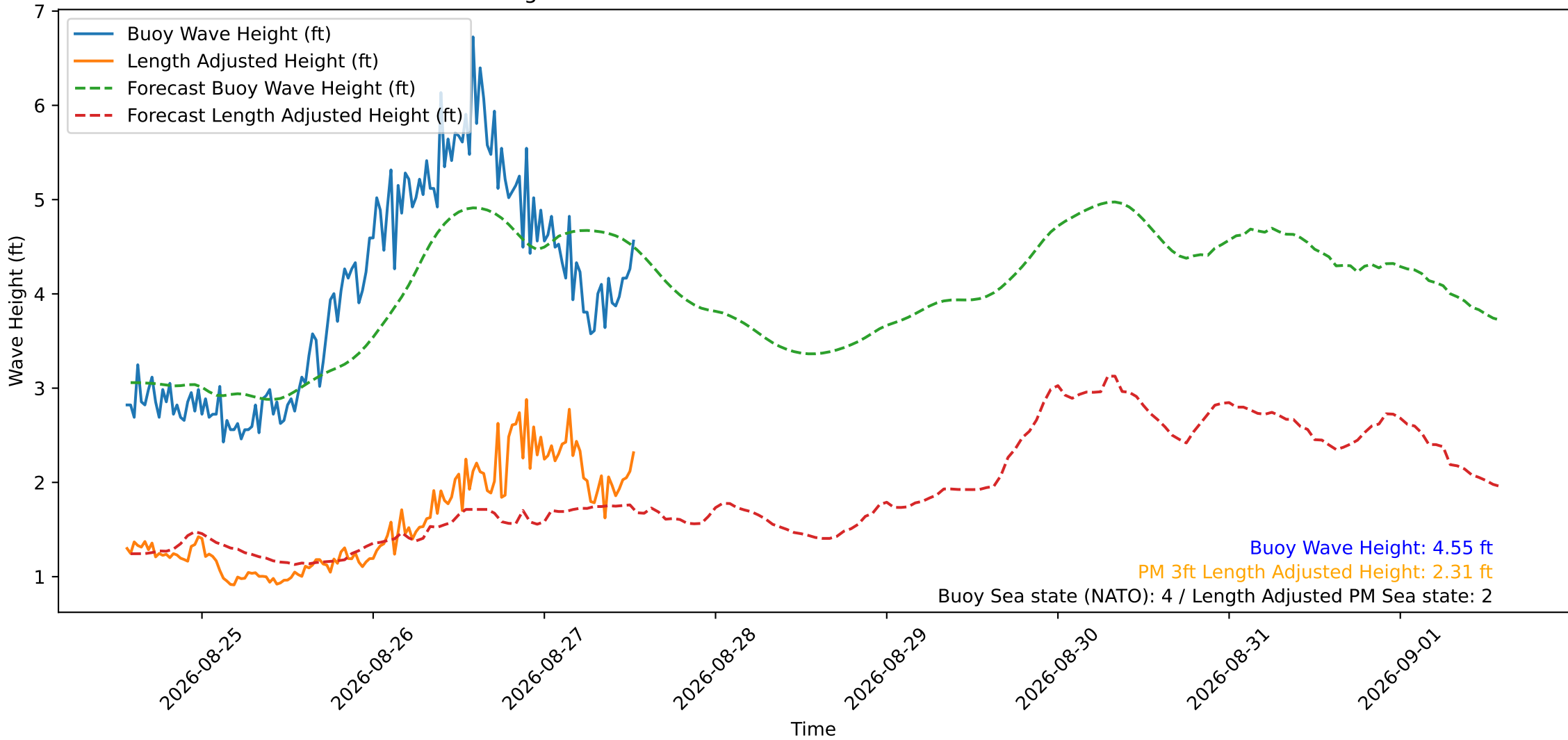
Wave Heights over Time for Oceanside Harbor at 2026-08-27 13:30:29
