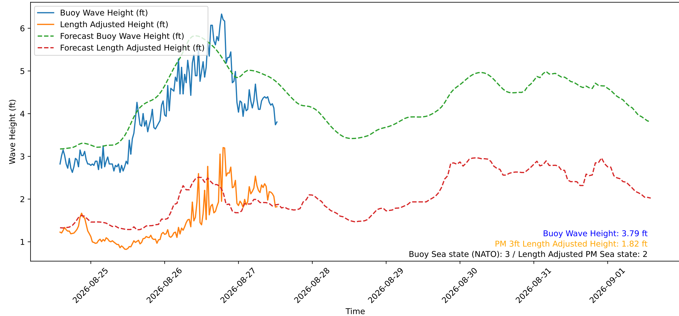
Wave Heights over Time for Green Beach at 2026-08-27 13:31:12
