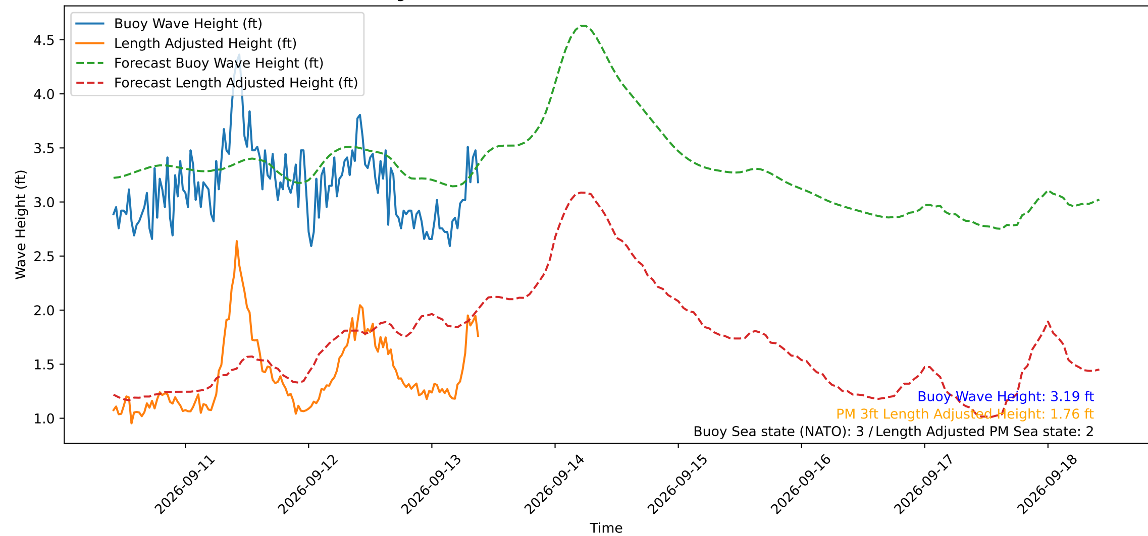
Wave Heights over Time for Oceanside Harbor at 2026-09-13 09:50:30
