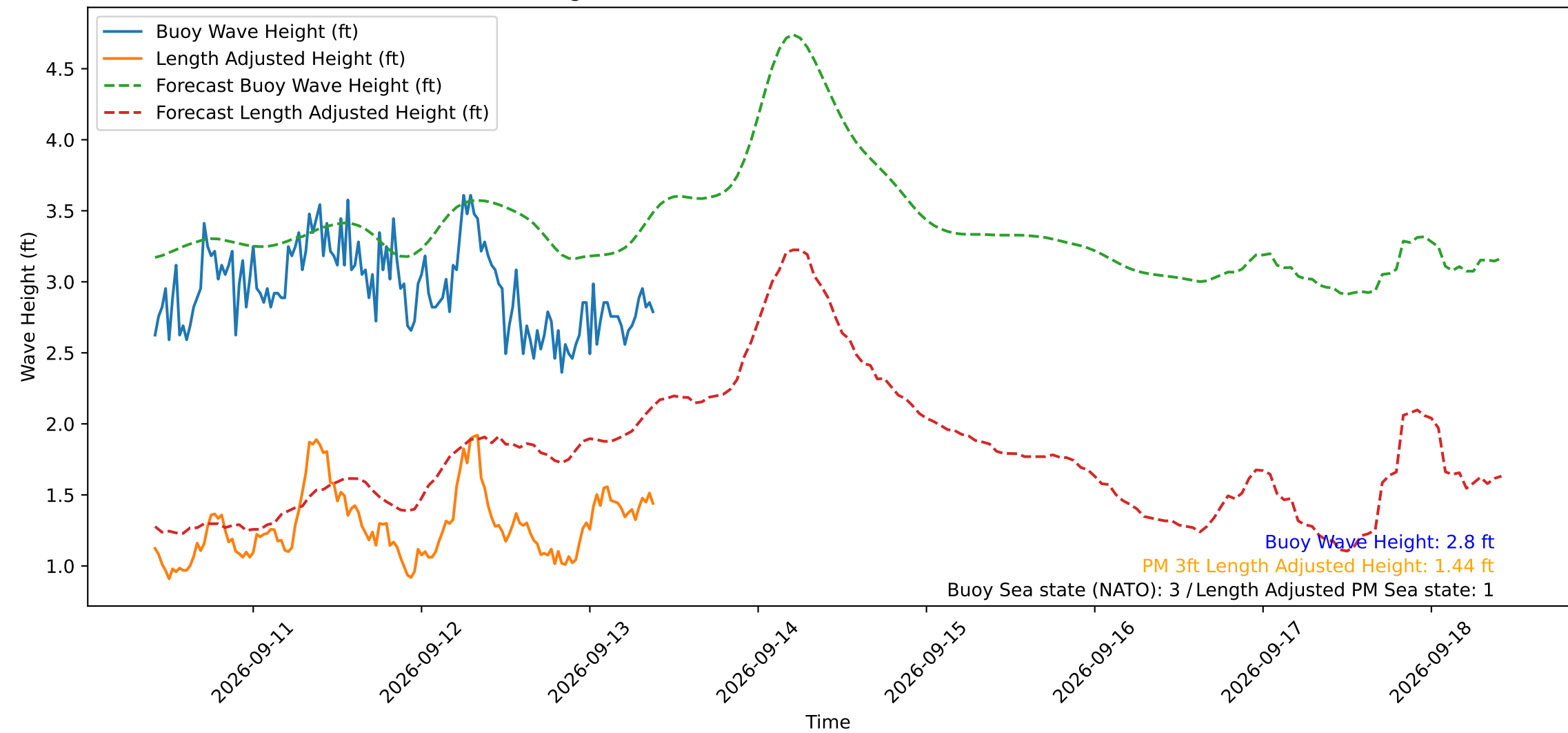
Wave Heights over Time for Green Beach at 2026-09-13 09:51:15
